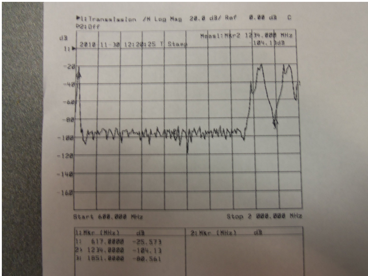
Figure 4-8E. Bandpass Filter Harmonic response
