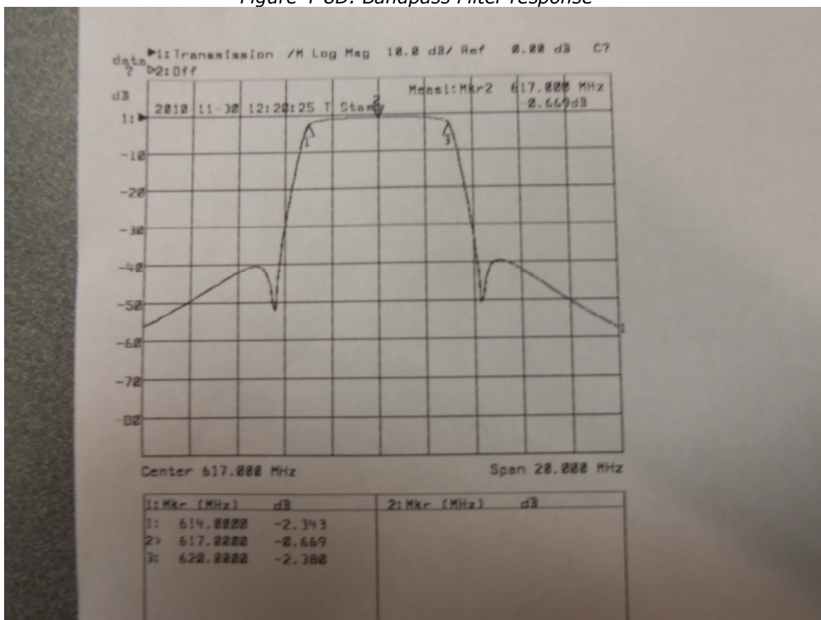
Figure 4-8D. Bandpass Filter response
