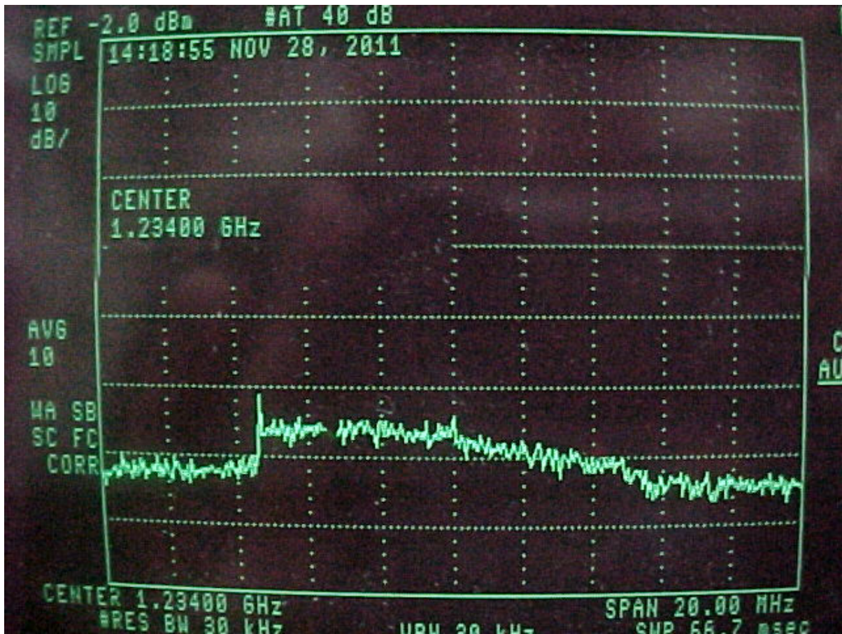
Figure 4-8B. Second Harmonic (1234.00 MHz) = -56 dBc(Pre-Filter)
