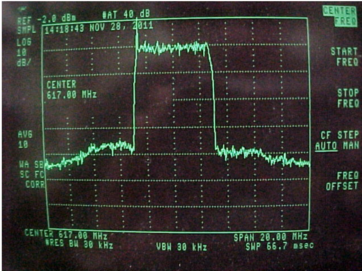
Figure 4-8A. Reference (617.00 MHz) = 0dBc (Pre-Filter)
