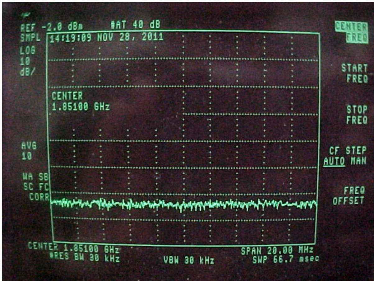
Figure 4-8C. Third Harmonic (1851.00 MHz) = <-65 dBc (Pre-Filter)
