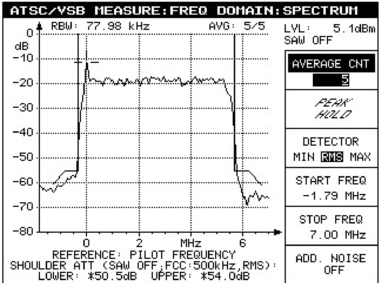
Figure 4-8J. Out of Band Emissions (Post Filter)
