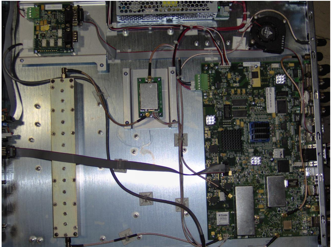
Photograph 3. Modulator Top View
