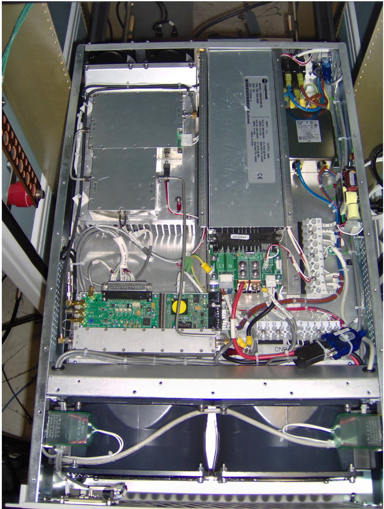
Photograph 2. Amplifier Top View
