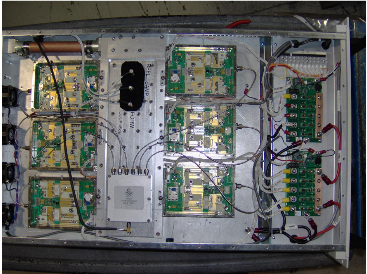
Photograph 1. Amplifier Bottom View
