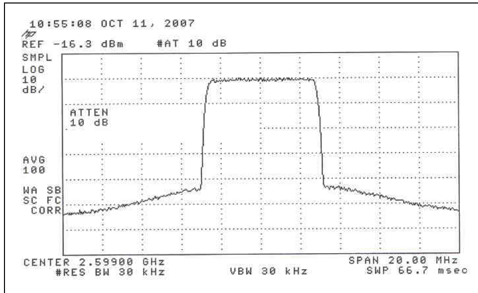
Figure 4-8. Conducted Spurious Emissions (before channel filter)
