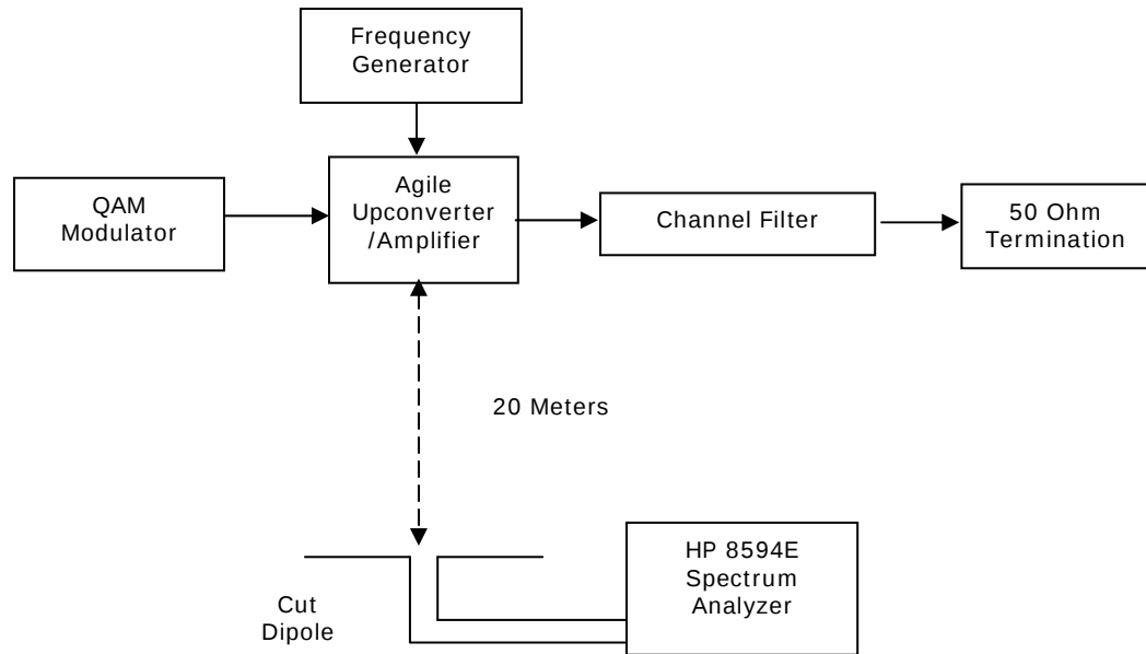
Figure 4-10. Test Setup for Measuring Radiated Emissions
