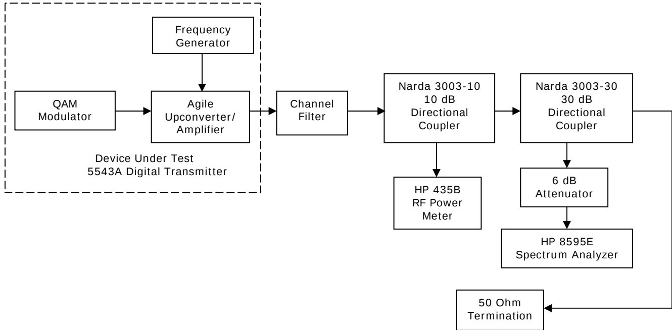
Figure 4-1. Test Equipment Setup for RF Power Measurements
