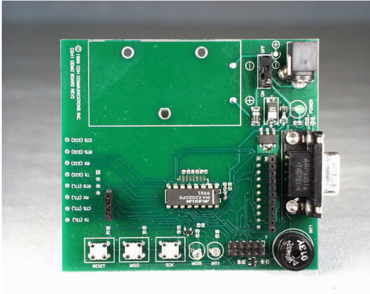
Front View of the Interface Board
