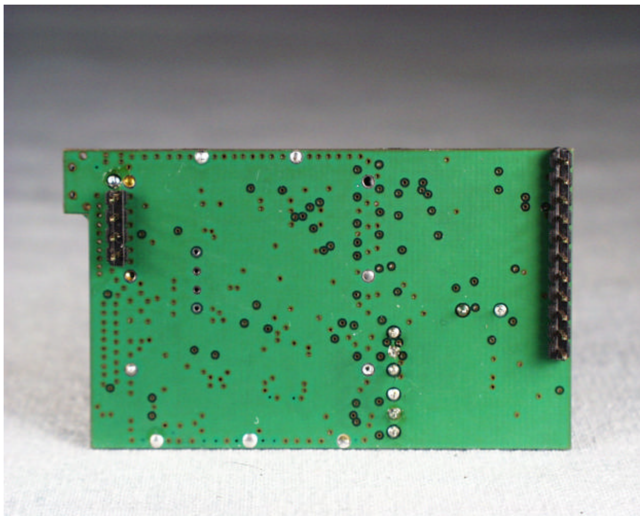
Back View of the Radio Board
