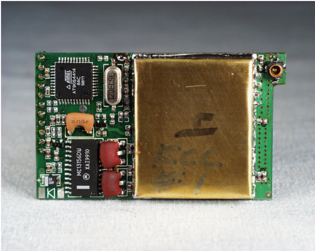
Front View of the Radio Board (with RF Can Installed)
