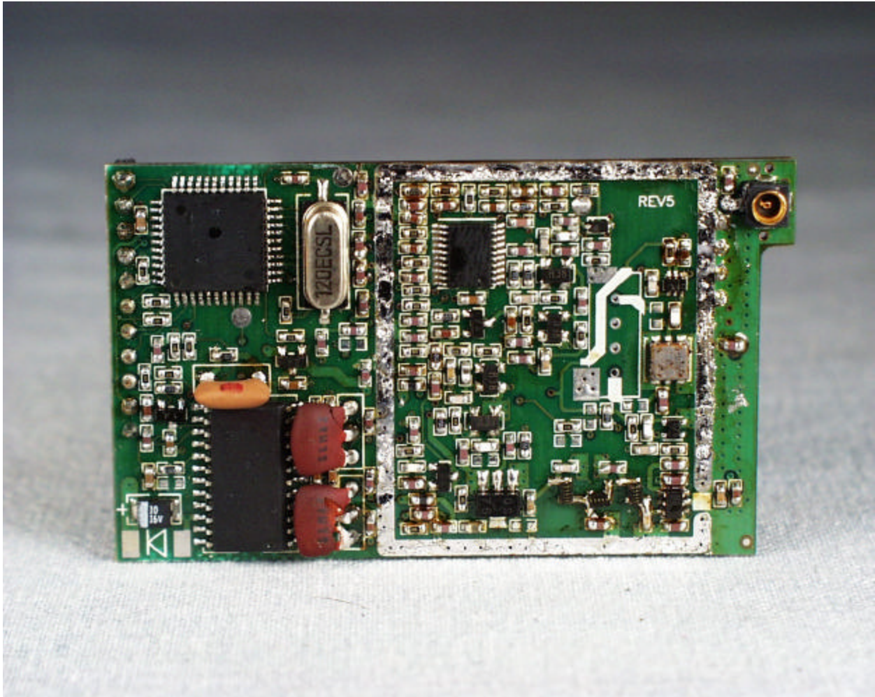
Front View of the Radio Board (with RF Can Removed)
