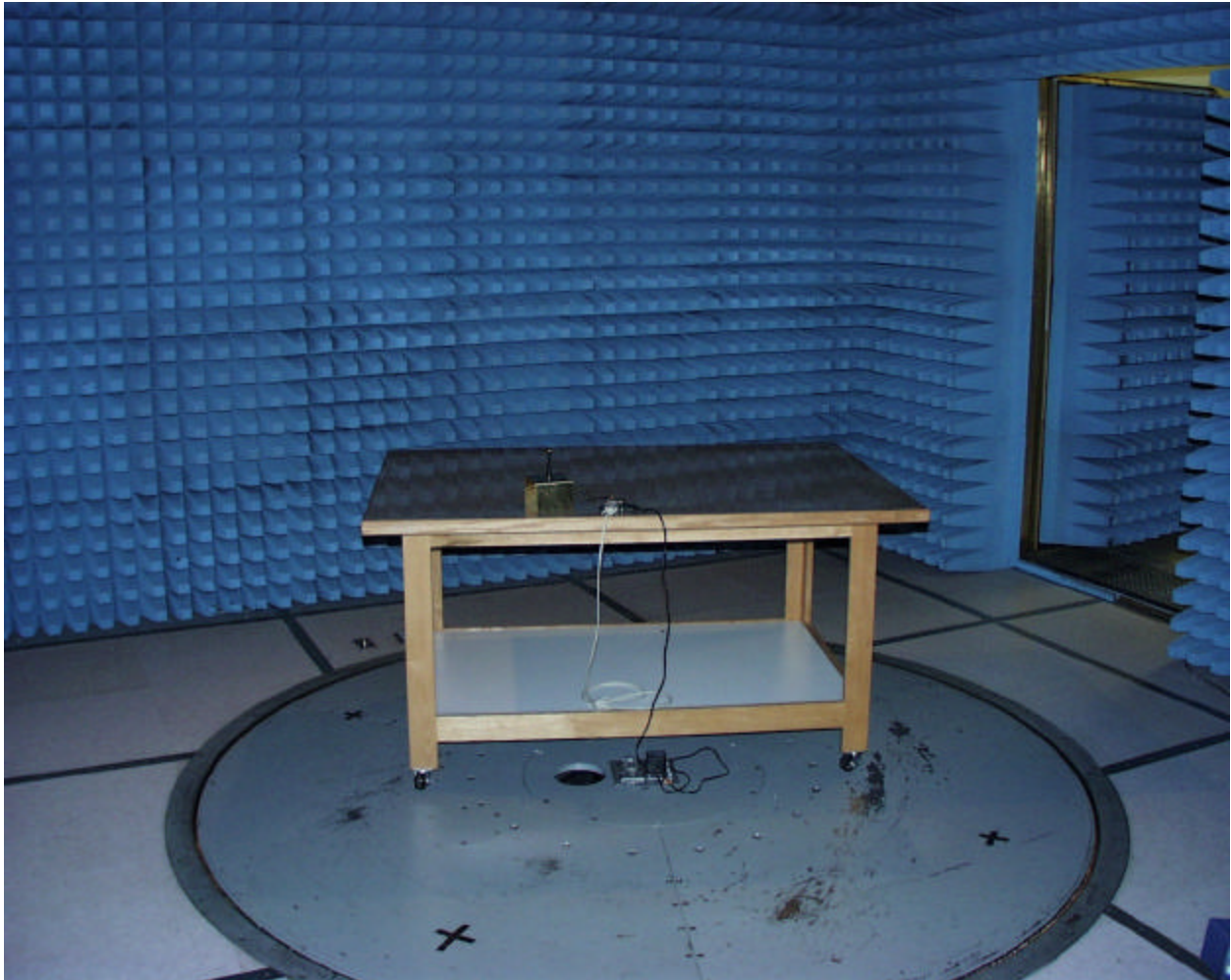
Worst case radiated emissions (Astron Monopole antenna)
