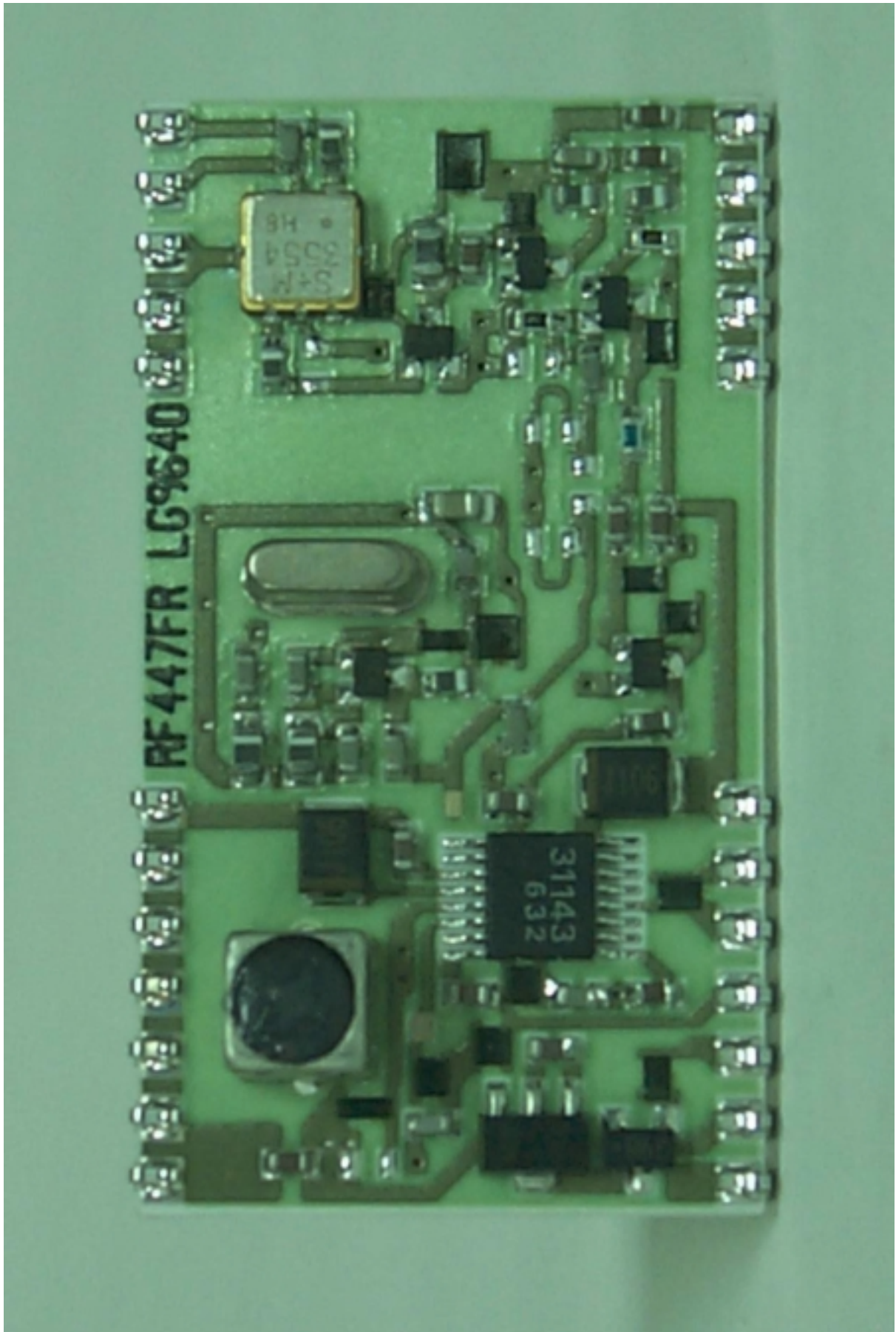
* RF MODULE TOP VIEW
