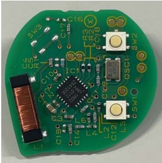
Figure 7.3. PCB assy (front view)
