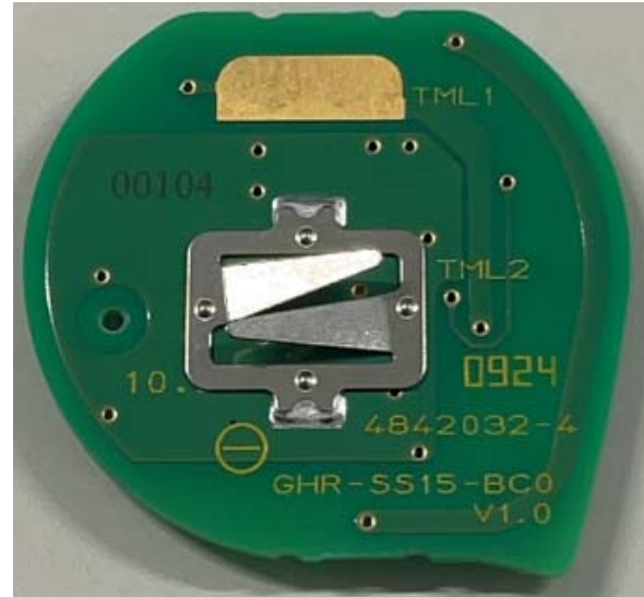
Figure 7.4. PCB assy (back view)
