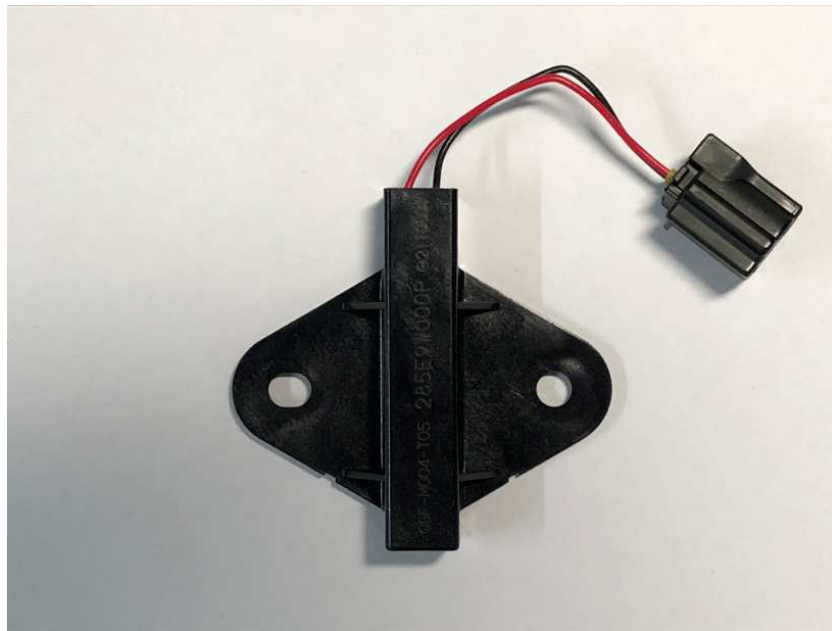
Figure 8.23 LF-antenna TG (CGF-M004-T05) appearance (front view)
