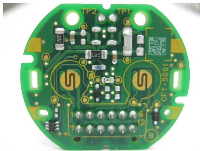
Figure 7.2.1 37290-54P0 PCB assy (top view)
