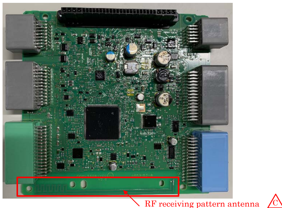
Figure 8.1 K84S0 PCB assy (top view) ※Pattern antenna is in red frame
