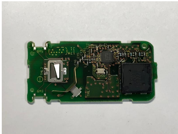
Figure 9.8 PCB assy (back view)
