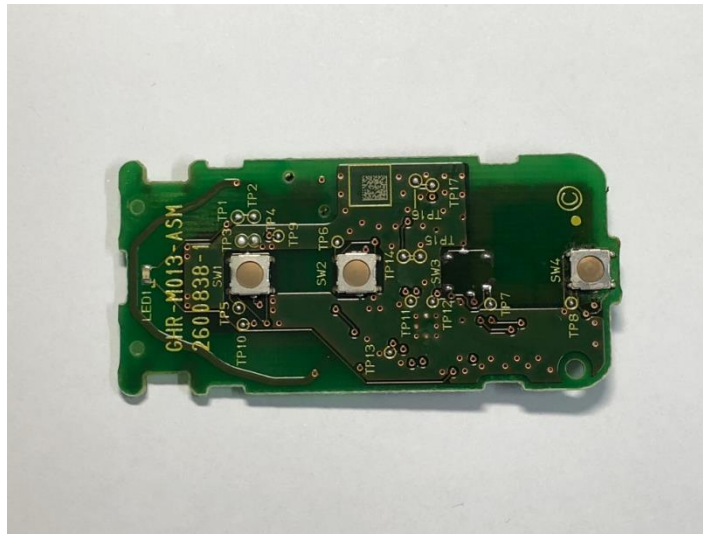
Figure 9.7 PCB assy (front view)
