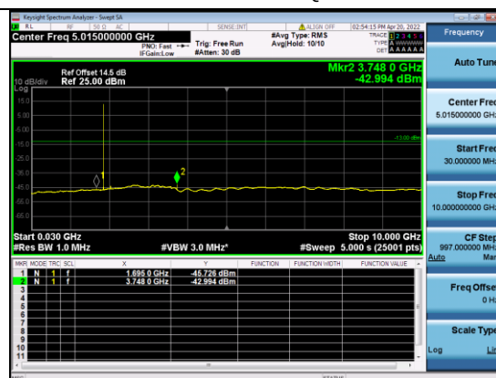
B25-20M-Mid CH-CSE-2-QPSK-1 RB 0
