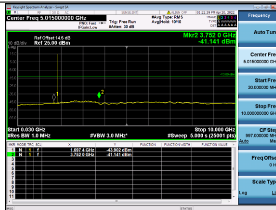
B25-15M-Mid CH-CSE-2-QPSK-1 RB 0
