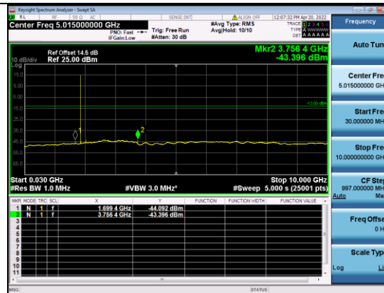
B25-10M-Mid CH-CSE-2-QPSK-1 RB 0
