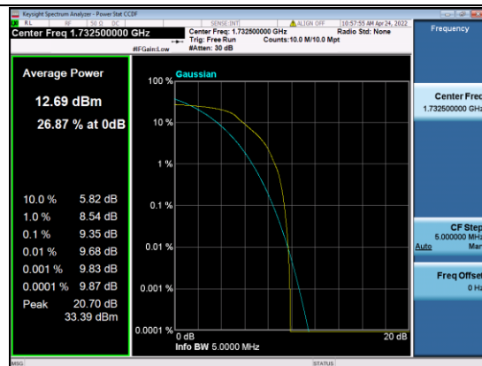
B4-3M-High CH-PAPR-QPSK
