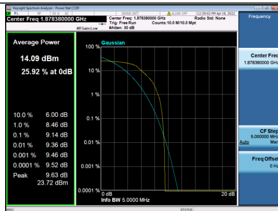
B2-10M-High CH-PAPR-QPSK
