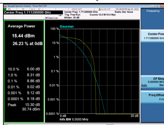
B4-15M-Low CH-PAPR-QPSK
