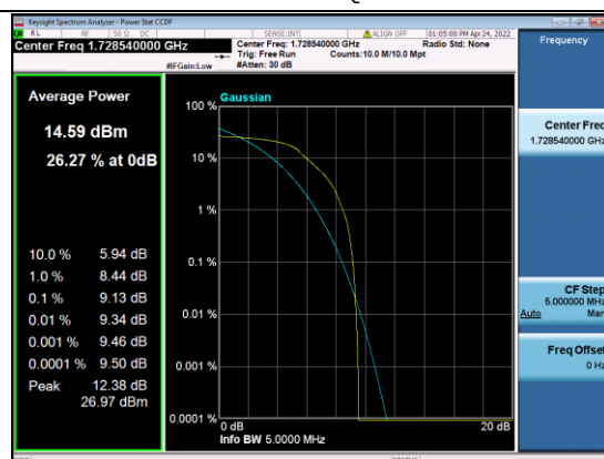
B4-15M-High CH-PAPR-QPSK
