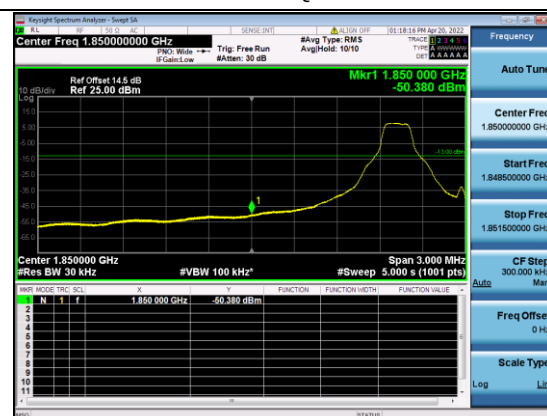
B25-15M-Low CH-BE-QPSK-1 RB 0
