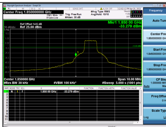
B25-10M-Low CH-BE-QPSK-Full RB 0
