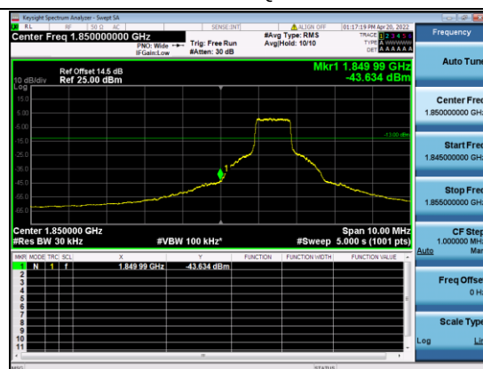
B25-15M-Low CH-BE-QPSK-Full RB 0
