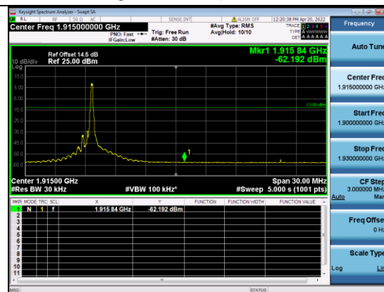
B25-10M-High CH-BE-QPSK-1 RB MAX
