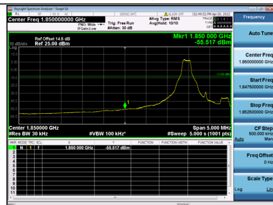
B25-20M-Low CH-BE-QPSK-1 RB 0
