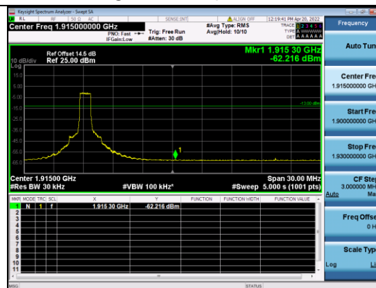
B25-10M-High CH-BE-QPSK-Full RB 0
