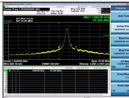
B25-10M-Low CH-BE-QPSK-1 RB 0
