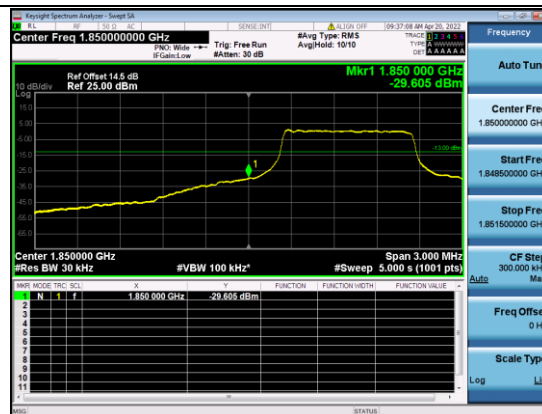
B25-5M-Low CH-BE-QPSK-Full RB 0
