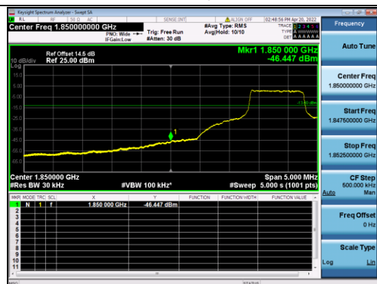
B25-20M-Low CH-BE-QPSK-Full RB 0
