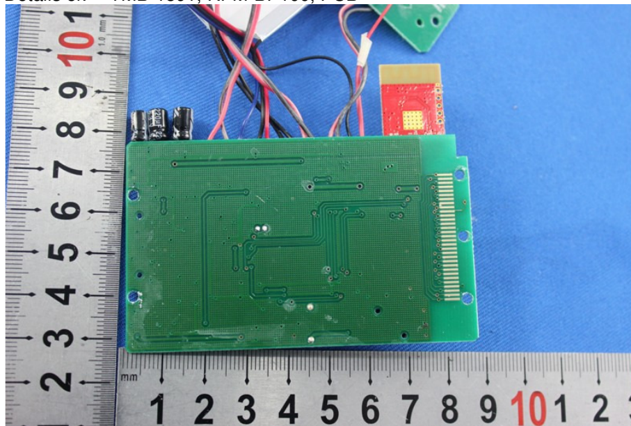
Details of: TMB-1591, RPM-BP100, PCB
