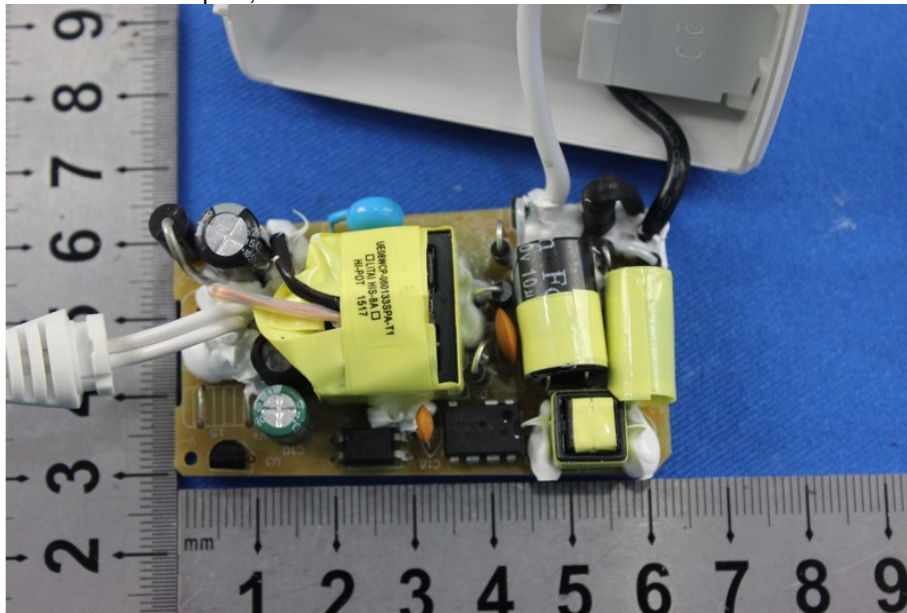
Details of: Adaptor, PCB
