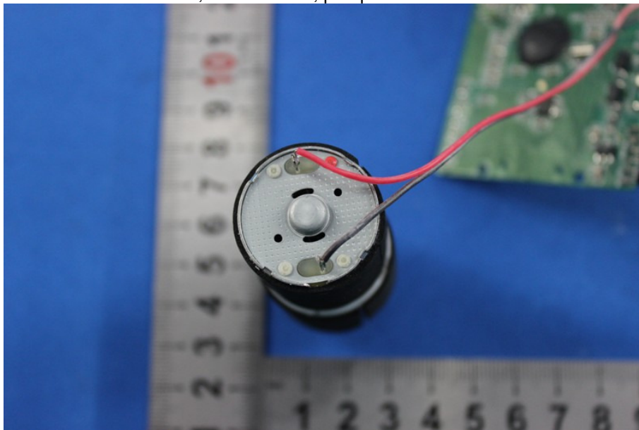
Details of: TMB-1591, RPM-BP100, pump
