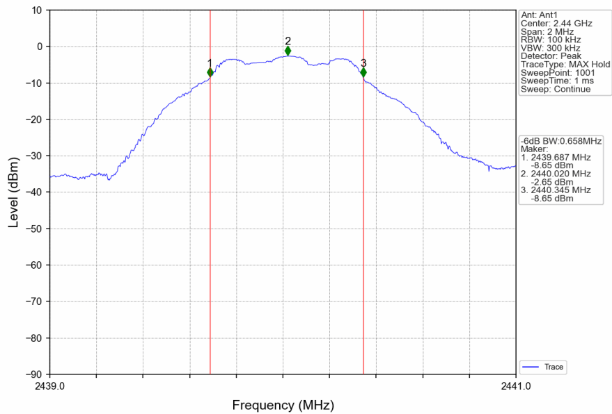
1M_MCH_2440MHz_Ant1_NTNV
