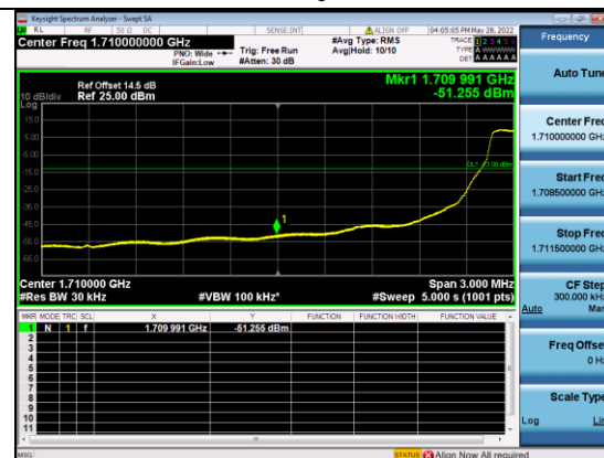
B4-20M-Low CH-BE-QPSK-1 RB 0
