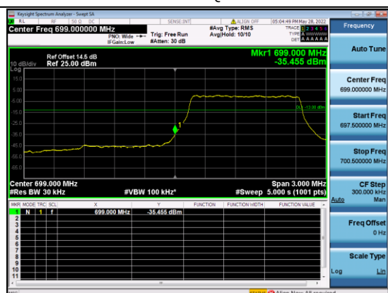
B12-1.4M-Low CH-BE-QPSK-Full RB 0
