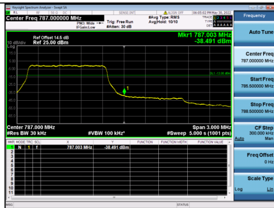
B13-5M-High CH-BE-QPSK-Full RB 0
