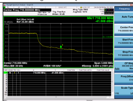
B12-10M-High CH-BE-QPSK-Full RB 0
