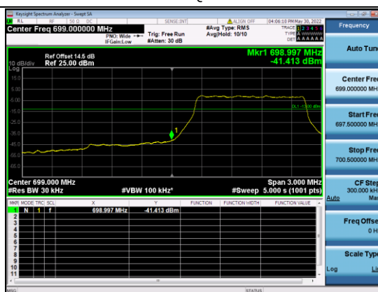
B12-5M-Low CH-BE-QPSK-Full RB 0
