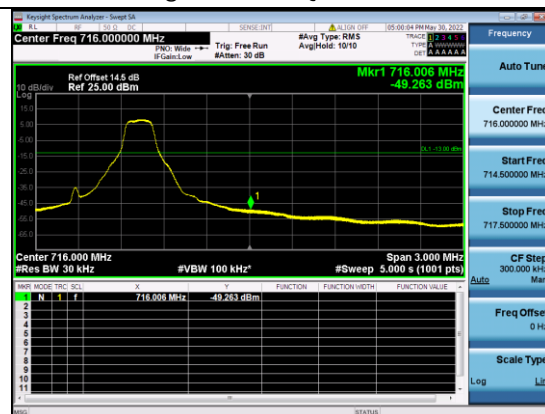
B12-10M-High CH-BE-Q16-Full RB 0
