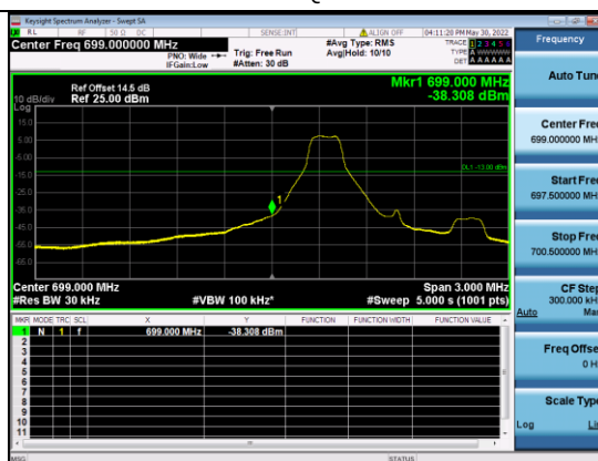
B12-5M-Low CH-BE-Q16-Full RB 0
