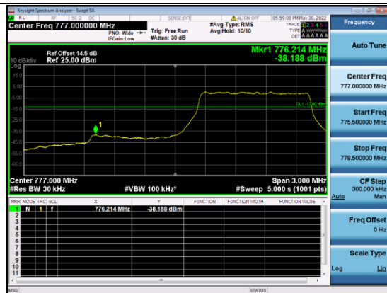
B13-5M-Low CH-BE-QPSK-Full RB 0
