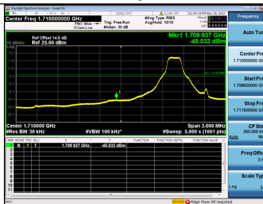
B4-10M-Low CH-BE-QPSK-1 RB 0
