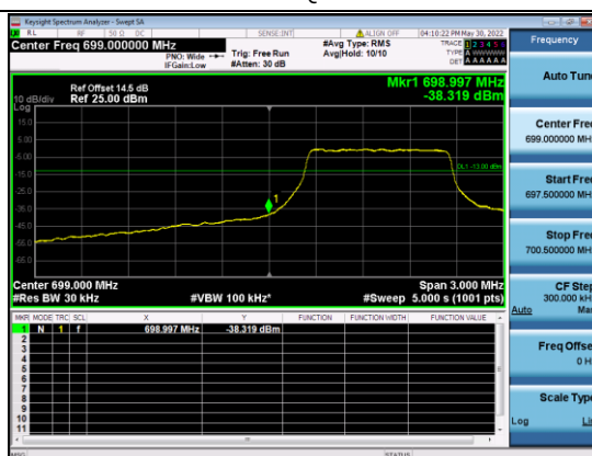
B12-5M-Low CH-BE-QPSK-1 RB 0
