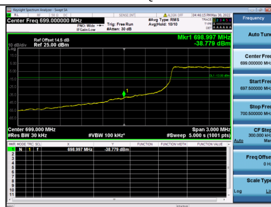
B12-10M-Low CH-BE-QPSK-1 RB 0
