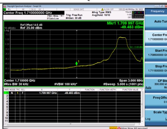
B4-15M-Low CH-BE-QPSK-1 RB 0
