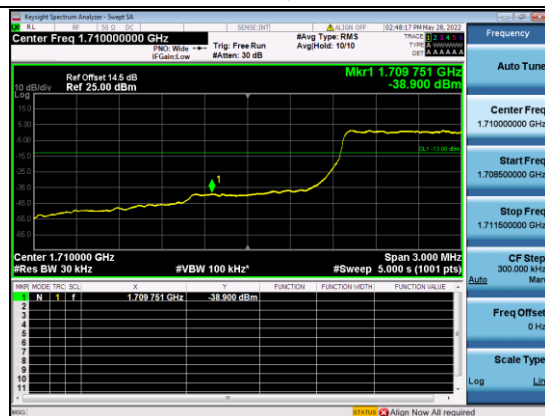
B4-10M-Low CH-BE-QPSK-Full RB 0
