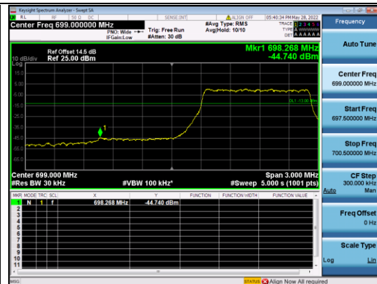
B12-3M-Low CH-BE-QPSK-Full RB 0
