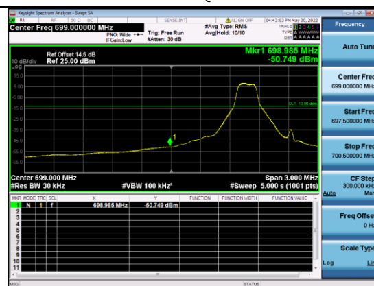
B12-10M-Low CH-BE-QPSK-Full RB 0
