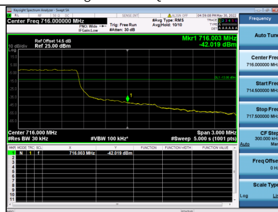
B12-10M-High CH-BE-QPSK-1 RB MAX
