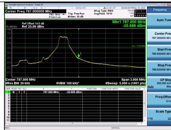
B13-5M-High CH-BE-QPSK-1 RB MAX
