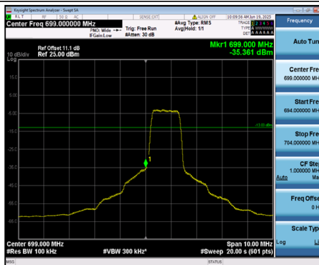
Band12-5MHz-QPSK-23035-6-0-Low--35.36-PASS
