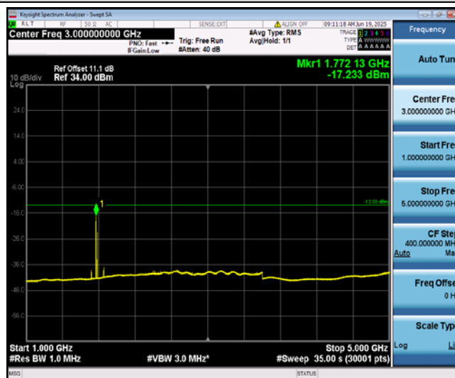
Band12-1.4MHz-16QAM-23095-1-0-Low-1000-5000--17.23-PASS
