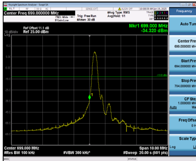
Band12-5MHz-QPSK-23035-1-0-Low--34.32-PASS
