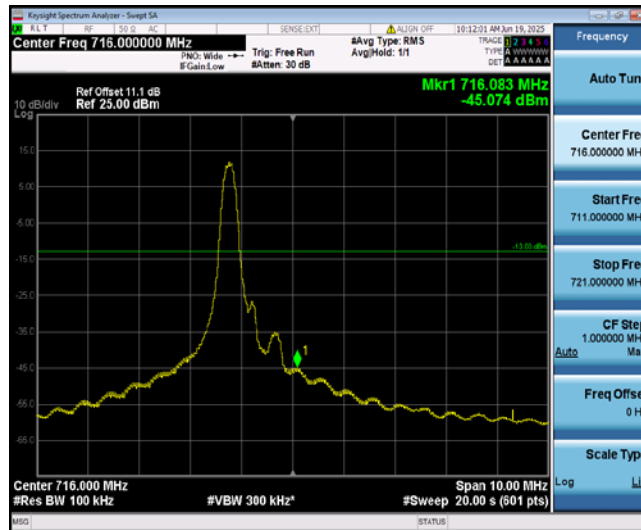
Band12-5MHz-16QAM-23155-1-0-High--45.07-PASS
