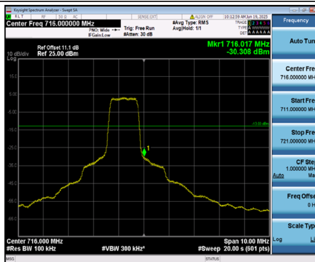
Band12-5MHz-16QAM-23155-6-0-High--30.31-PASS
