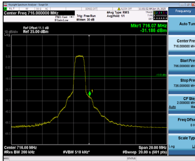
Band12-10MHz-16QAM-23130-6-0-High--31.19-PASS
