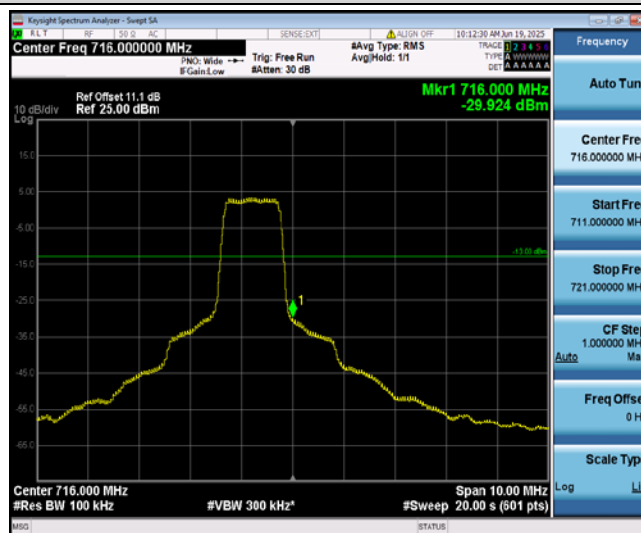
Band12-5MHz-QPSK-23155-6-0-High--29.92-PASS
