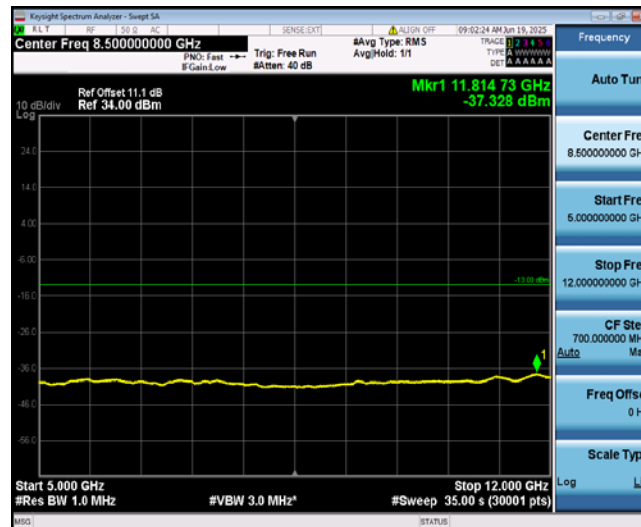
Band12-1.4MHz-QPSK-23017-1-0-Low-5000-12000--37.33-PASS
