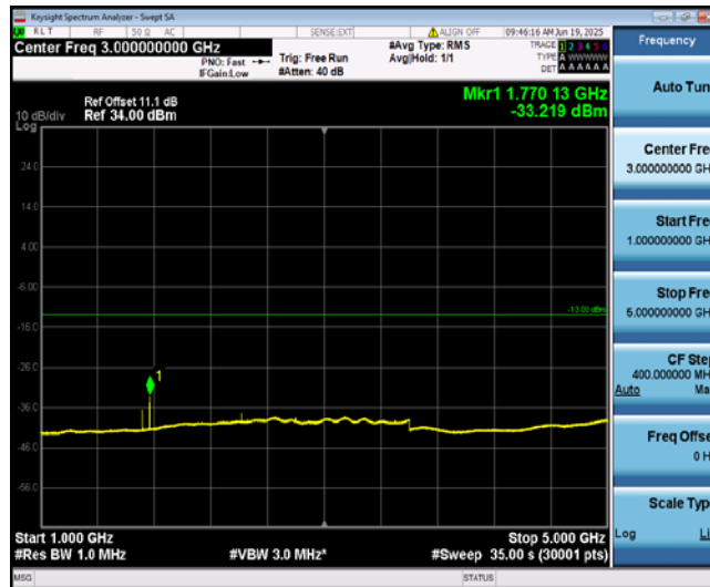
Band12-3MHz-QPSK-23025-1-0-Low-1000-5000--33.22-PASS
