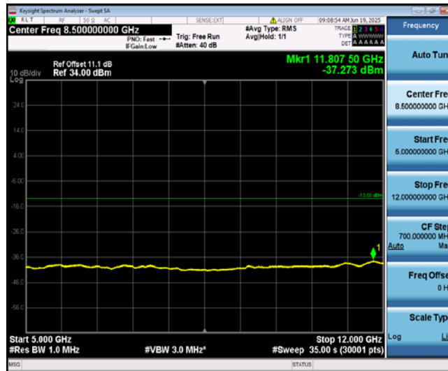
Band12-1.4MHz-QPSK-23095-1-0-Low-5000-12000--37.27-PASS
