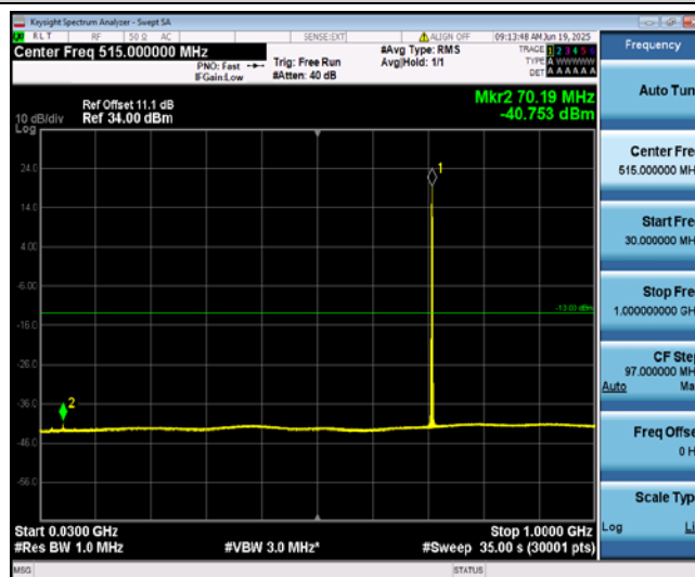
Band12-1.4MHz-QPSK-23173-1-0-High-30-1000--40.75-PASS
