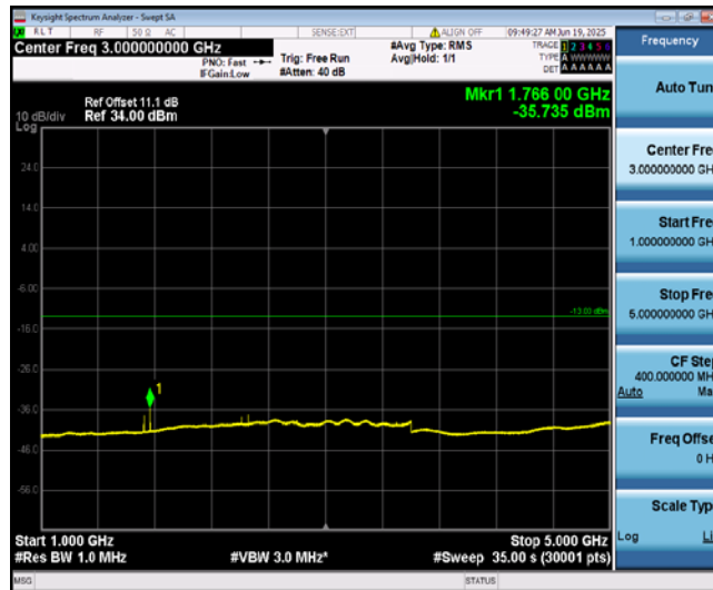
Band12-3MHz-16QAM-23025-1-0-Low-1000-5000--35.74-PASS
