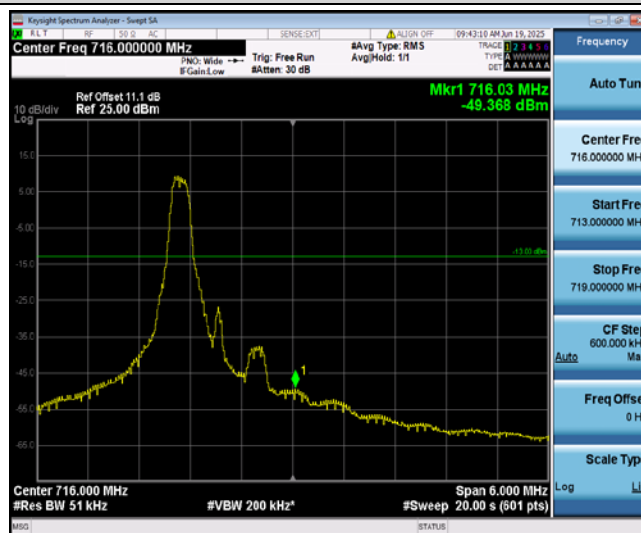
Band12-3MHz-QPSK-23165-1-0-High--49.37-PASS
