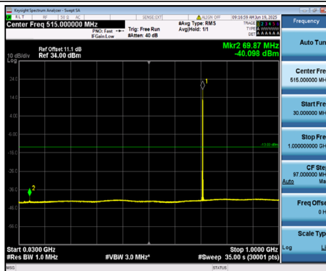
Band12-1.4MHz-16QAM-23173-1-0-High-30-1000--40.1-PASS
