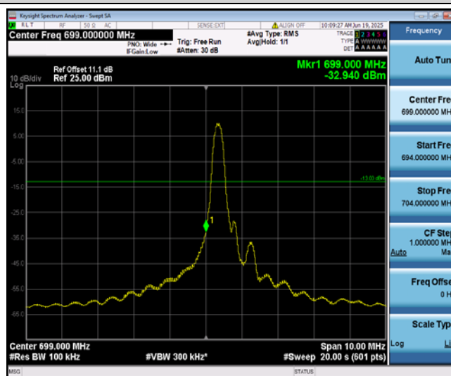
Band12-5MHz-16QAM-23035-1-0-Low--32.94-PASS
