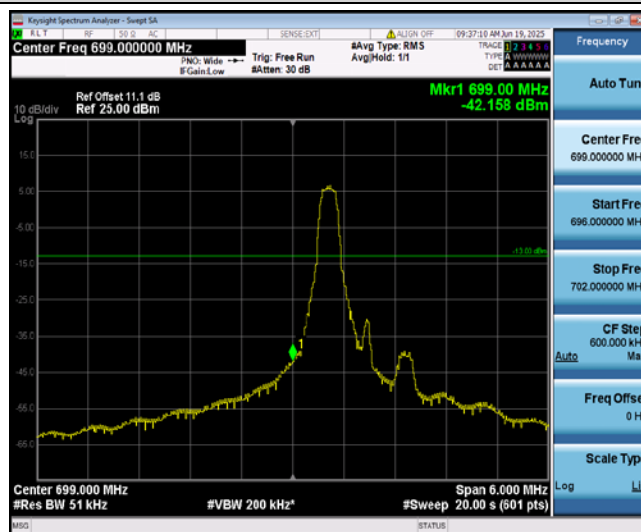
Band12-3MHz-QPSK-23025-1-0-Low--42.16-PASS
