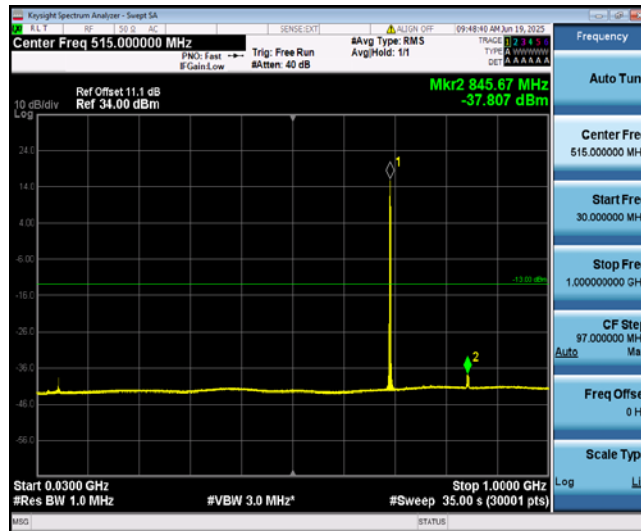
Band12-3MHz-16QAM-23025-1-0-Low-30-1000--37.81-PASS
