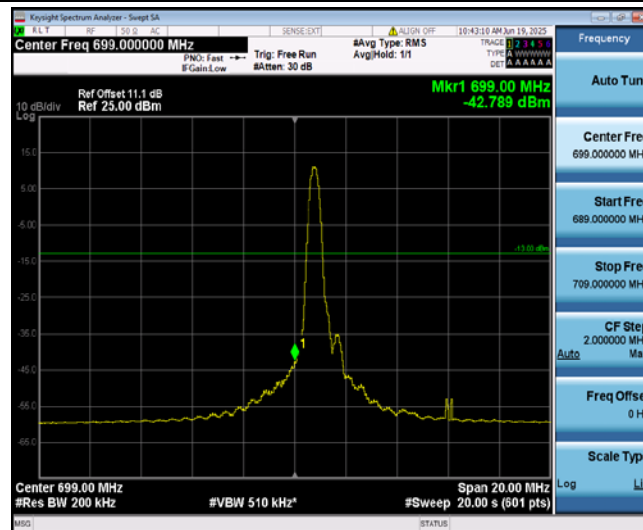
Band12-10MHz-16QAM-23060-1-0-Low--42.79-PASS
