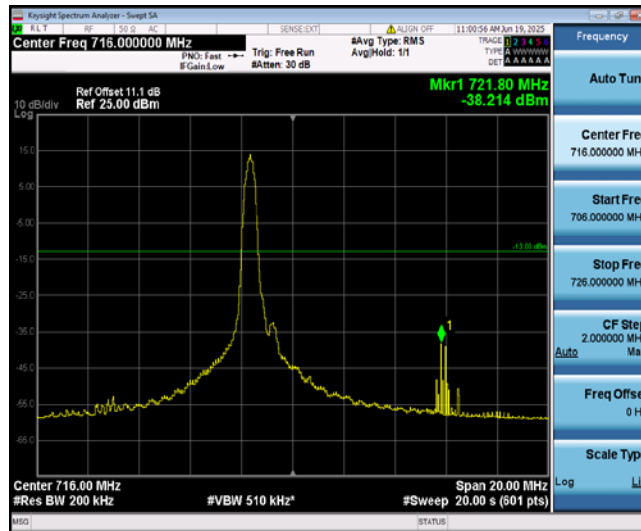
Band12-10MHz-16QAM-23130-1-0-High--38.21-PASS
