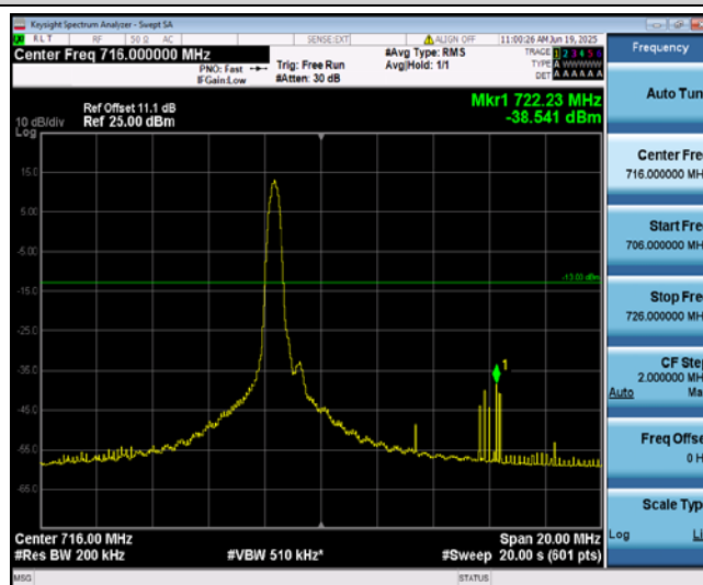
Band12-10MHz-QPSK-23130-1-0-High--38.54-PASS
