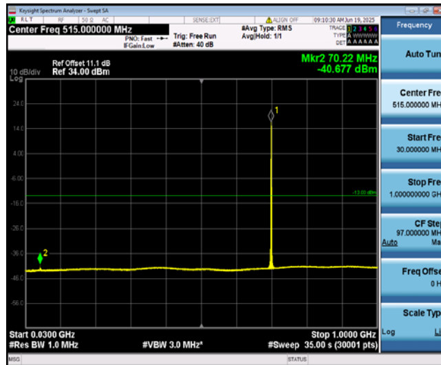
Band12-1.4MHz-16QAM-23095-1-0-Low-30-1000--40.68-PASS
