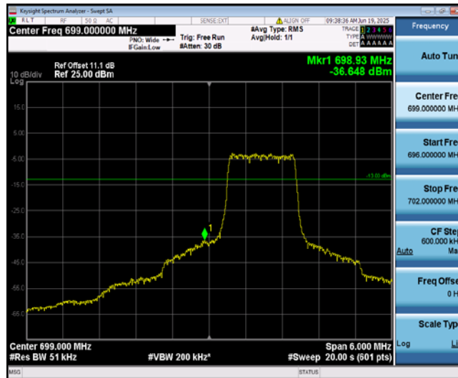
Band12-3MHz-16QAM-23025-6-0-Low--36.65-PASS
