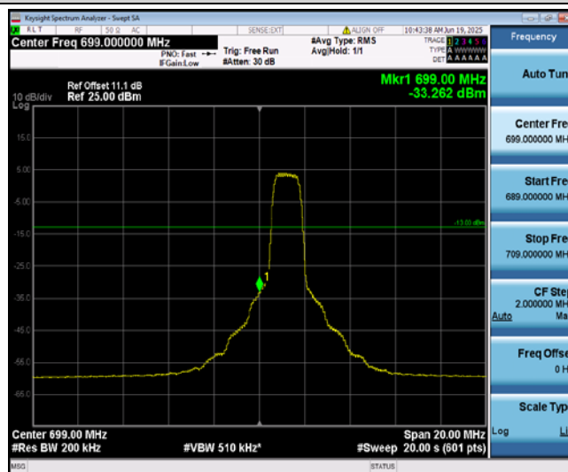
Band12-10MHz-QPSK-23060-6-0-Low--33.26-PASS
