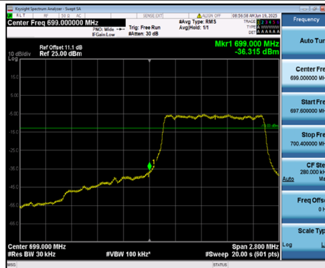
Band12-1.4MHz-QPSK-23017-6-0-Low--36.32-PASS
