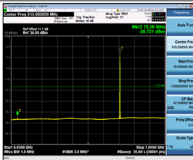
Band12-3MHz-16QAM-23165-1-0-High-30-1000--39.72-PASS
