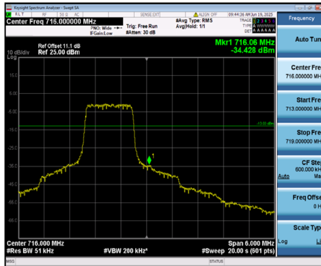
Band12-3MHz-16QAM-23165-6-0-High--34.43-PASS
