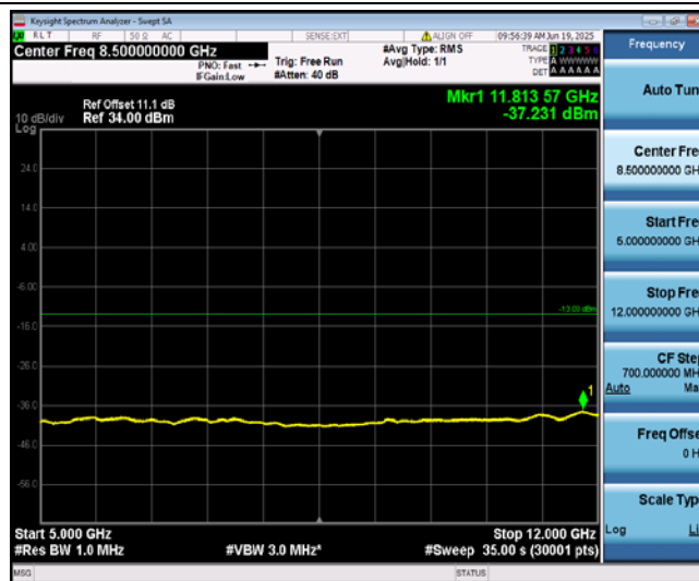
Band12-3MHz-16QAM-23095-1-0-Low-5000-12000--37.23-PASS
