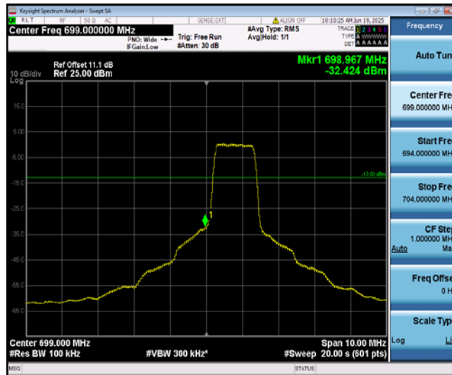
Band12-5MHz-16QAM-23035-6-0-Low--32.42-PASS
