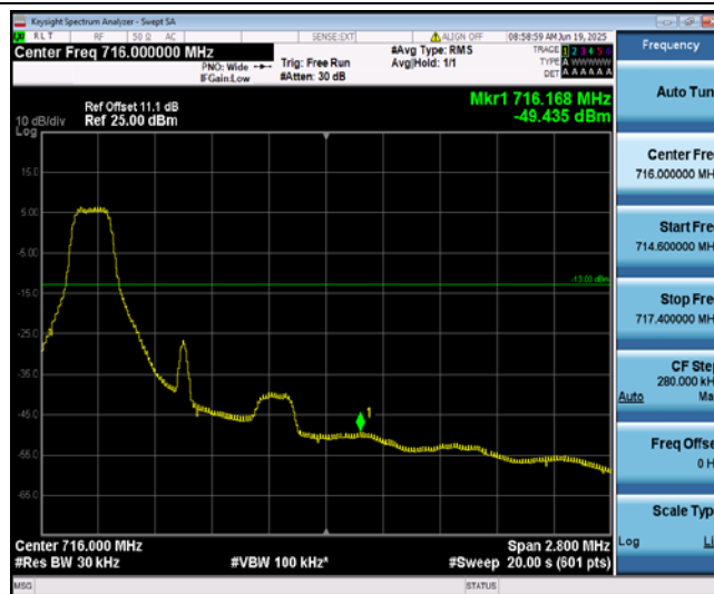
Band12-1.4MHz-16QAM-23173-1-0-High--49.44-PASS
