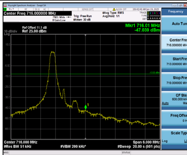
Band12-3MHz-16QAM-23165-1-0-High--47.04-PASS
