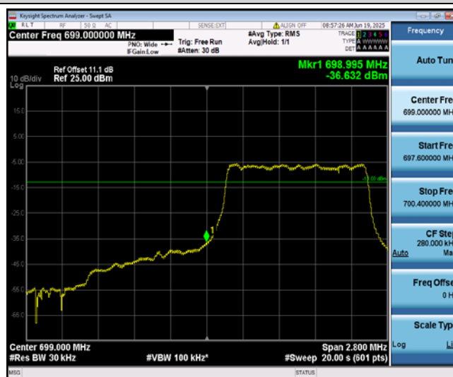
Band12-1.4MHz-16QAM-23017-6-0-Low--36.63-PASS
