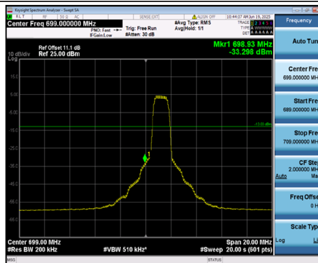
Band12-10MHz-16QAM-23060-6-0-Low--33.30-PASS
