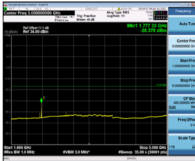
Band12-1.4MHz-16QAM-23017-1-0-Low-1000-5000--28.38-PASS
