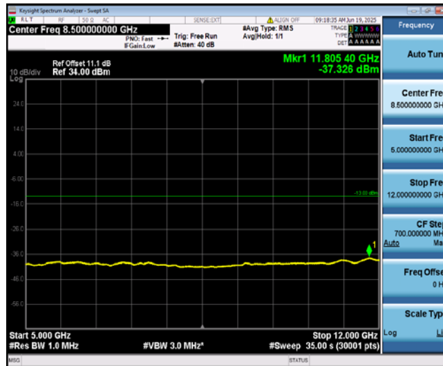
Band12-1.4MHz-16QAM-23173-1-0-High-5000-12000--37.33-PASS
