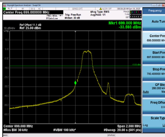
Band12-1.4MHz-16QAM-23017-1-0-Low--33.59-PASS
