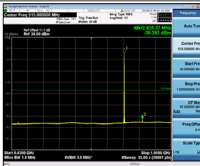
Band12-3MHz-QPSK-23165-1-0-High-30-1000--39.29-PASS
