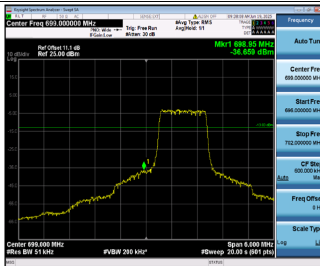
Band12-3MHz-QPSK-23025-6-0-Low--36.66-PASS
