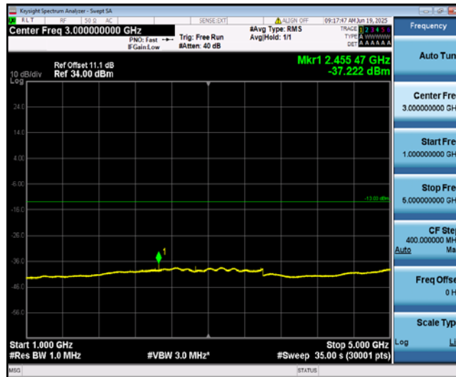
Band12-1.4MHz-16QAM-23173-1-0-High-1000-5000--37.22-PASS
