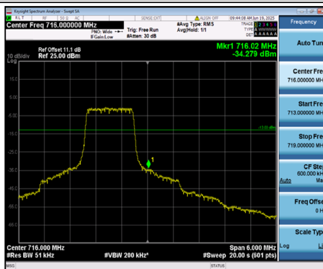
Band12-3MHz-QPSK-23165-6-0-High--34.28-PASS
