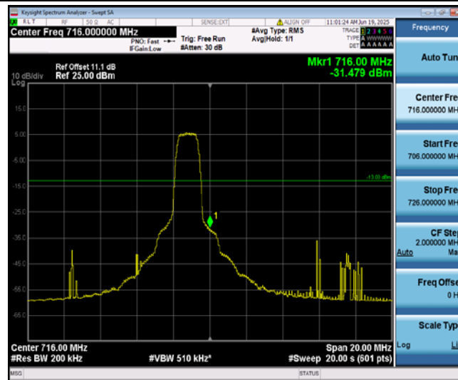
Band12-10MHz-QPSK-23130-6-0-High--31.48-PASS
