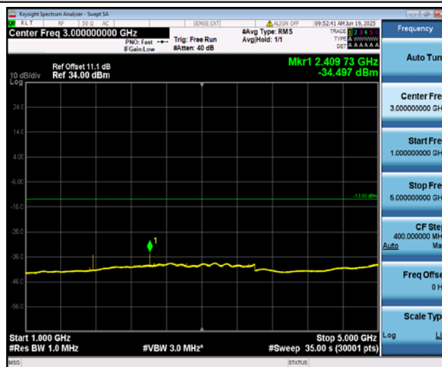
Band12-3MHz-QPSK-23095-1-0-Low-1000-5000--34.5-PASS
