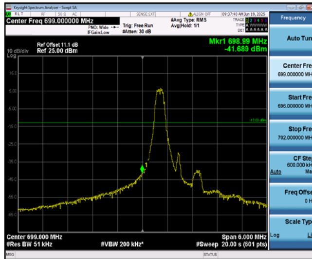
Band12-3MHz-16QAM-23025-1-0-Low--41.69-PASS
