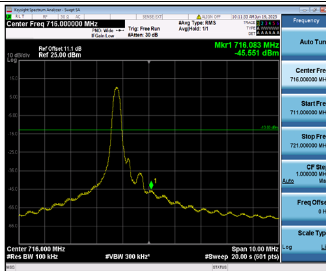
Band12-5MHz-QPSK-23155-1-0-High--45.55-PASS
