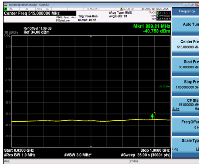
Band4-5MHz-QPSK-20175-1-0-Low-30-1000--40.76-PASS
