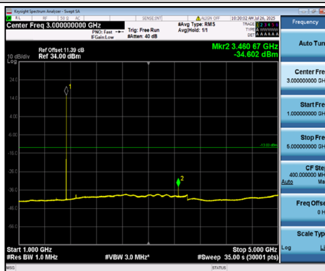
Band4-5MHz-16QAM-20175-1-0-Low-1000-5000--34.6-PASS
