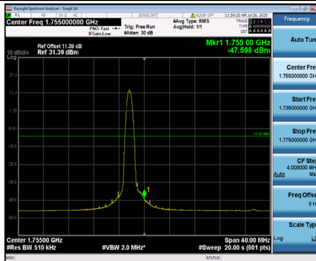
Band4-20MHz-16QAM-20300-1-0-High--47.60-PASS
