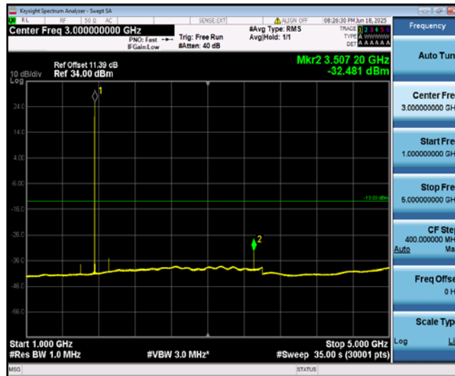
Band4-3MHz-QPSK-20385-1-0-High-1000-5000--32.48-PASS
