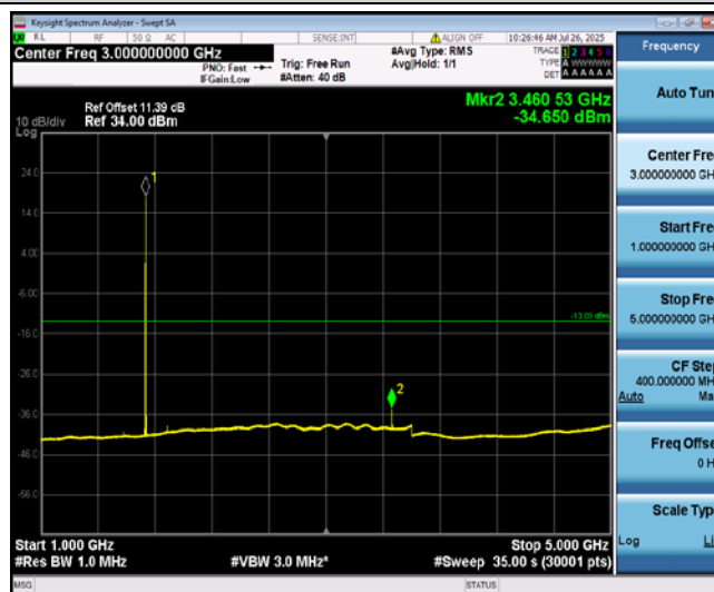
Band4-5MHz-QPSK-20175-1-0-Low-1000-5000--34.65-PASS
