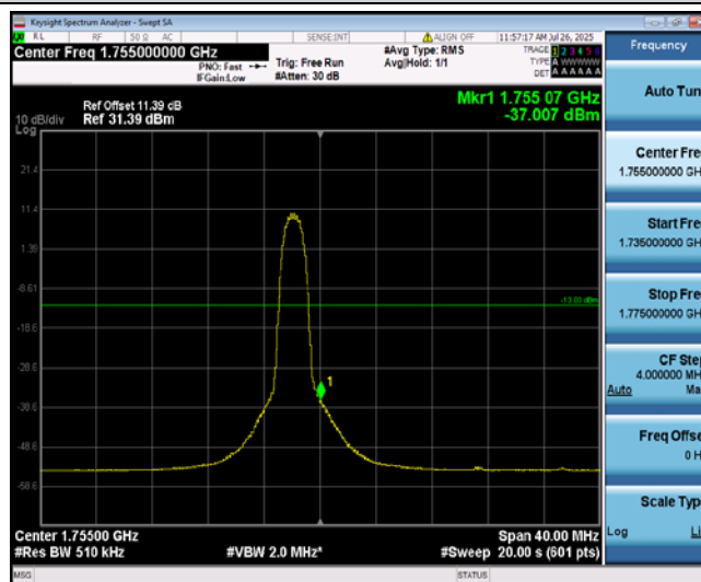
Band4-20MHz-16QAM-20300-6-0-High--37.01-PASS
