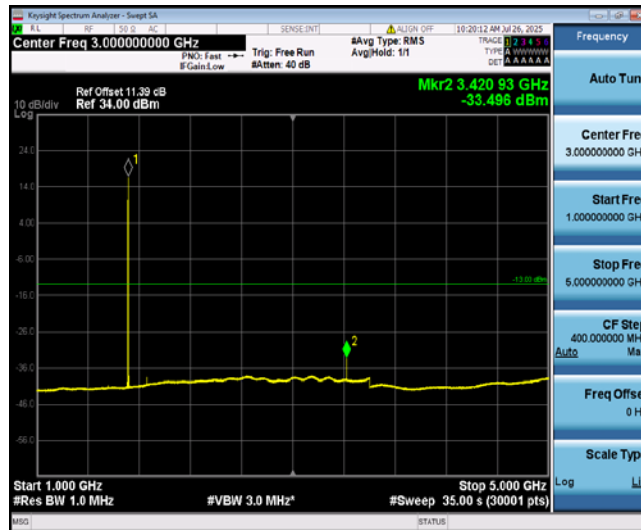
Band4-5MHz-QPSK-19975-1-0-Low-1000-5000--33.5-PASS
