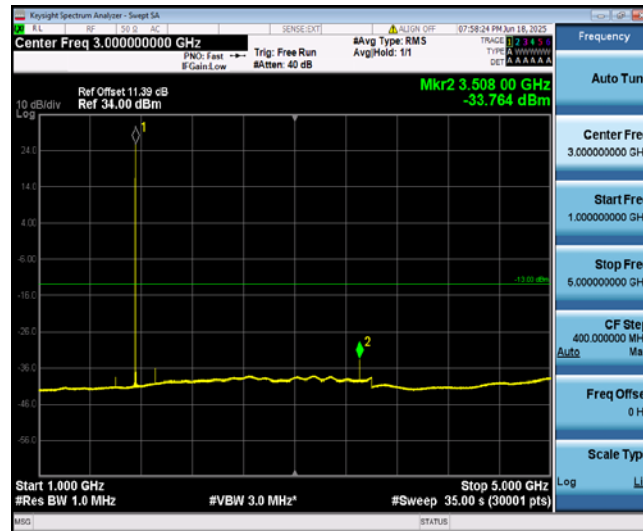
Band4-1.4MHz-16QAM-20393-1-0-High-1000-5000--33.76-PASS
