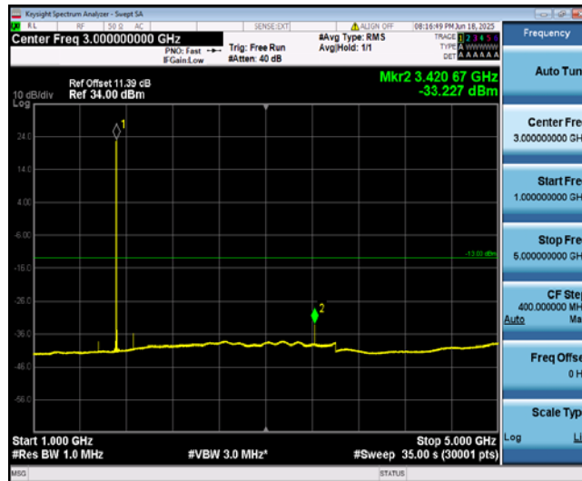
Band4-3MHz-16QAM-19965-1-0-Low-1000-5000--33.23-PASS
