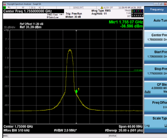
Band4-20MHz-QPSK-20300-6-0-High--36.60-PASS
