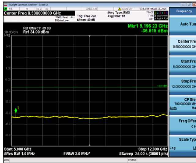
Band4-1.4MHz-16QAM-20175-1-0-Low-5000-12000--36.52-PASS
