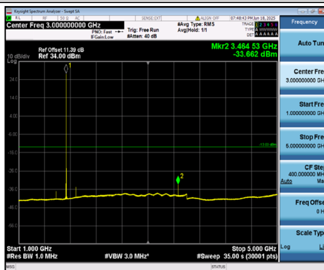
Band4-1.4MHz-QPSK-20175-1-0-Low-1000-5000--33.66-PASS
