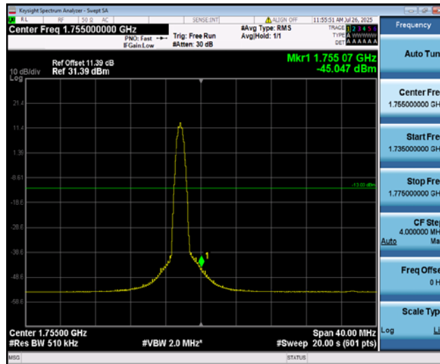
Band4-20MHz-QPSK-20300-1-0-High--45.05-PASS
