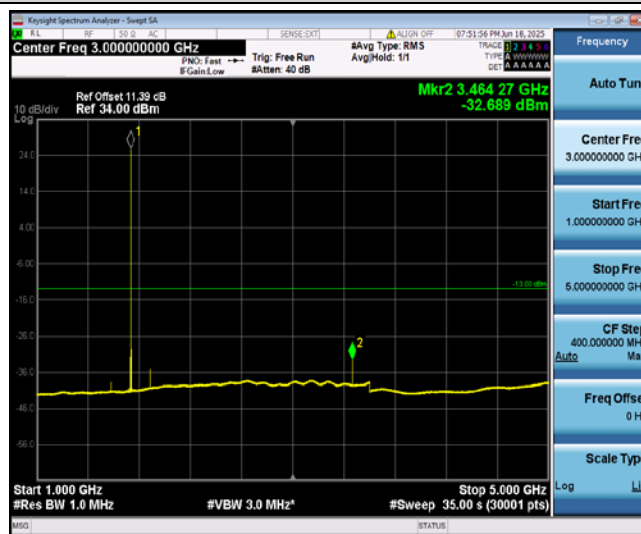
Band4-1.4MHz-16QAM-20175-1-0-Low-1000-5000--32.69-PASS
