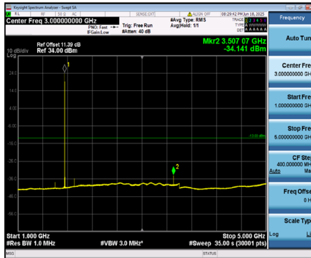
Band4-3MHz-16QAM-20385-1-0-High-1000-5000--34.14-PASS
