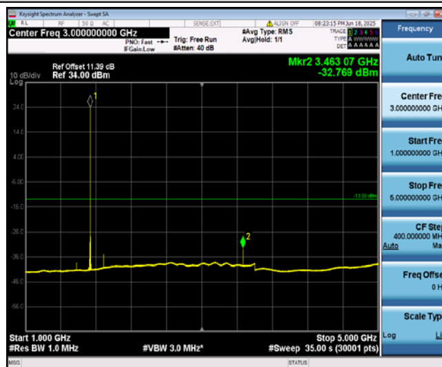
Band4-3MHz-16QAM-20175-1-0-Low-1000-5000--32.77-PASS
