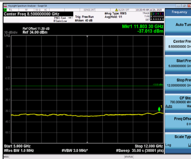
Band4-5MHz-16QAM-20175-1-0-Low-5000-12000--37.01-PASS
