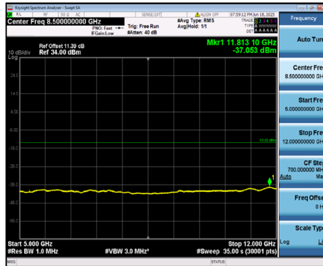
Band4-1.4MHz-16QAM-20393-1-0-High-5000-12000--37.05-PASS
