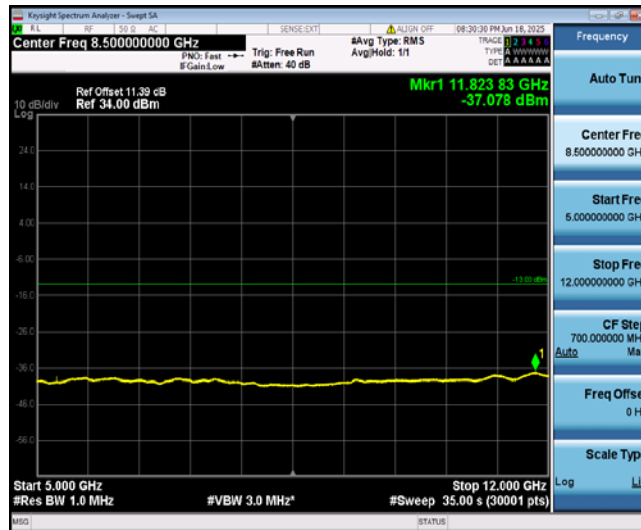
Band4-3MHz-16QAM-20385-1-0-High-5000-12000--37.08-PASS
