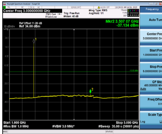
Band4-5MHz-QPSK-20375-1-0-High-1000-5000--37.13-PASS
