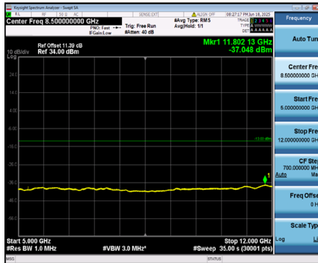
Band4-3MHz-QPSK-20385-1-0-High-5000-12000--37.05-PASS
