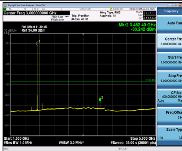
Band4-3MHz-QPSK-20175-1-0-Low-1000-5000--33.24-PASS
