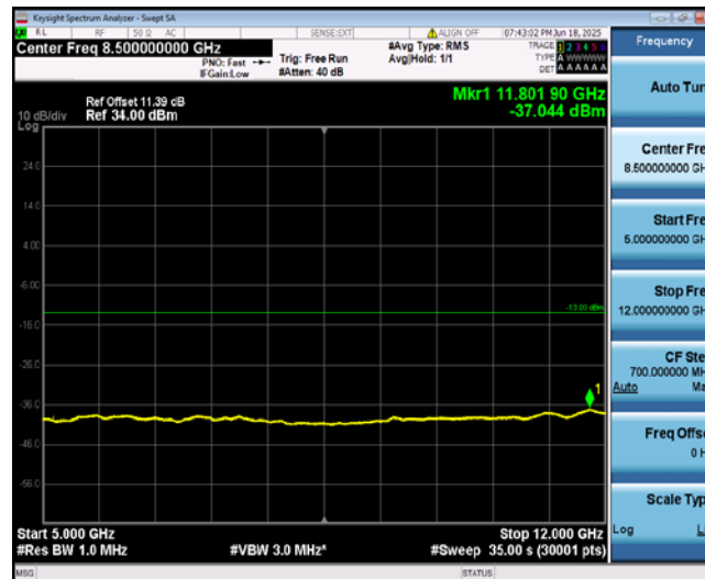
Band4-1.4MHz-QPSK-19957-1-0-Low-5000-12000--37.04-PASS
