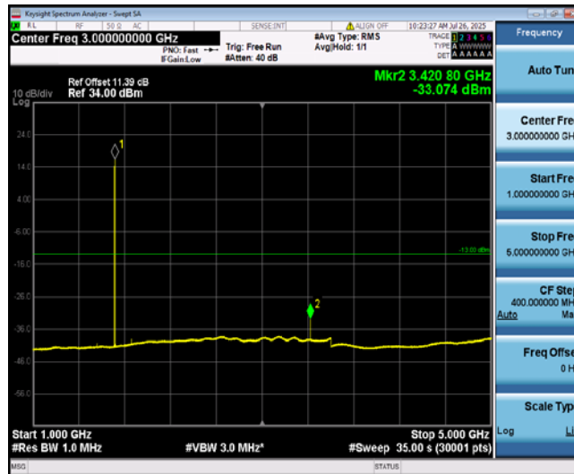
Band4-5MHz-16QAM-19975-1-0-Low-1000-5000--33.07-PASS
