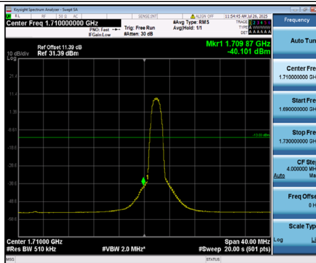
Band4-20MHz-16QAM-20050-6-0-Low--40.10-PASS
