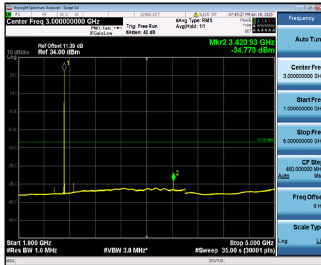
Band4-1.4MHz-16QAM-19957-1-0-Low-1000-5000--34.77-PASS
