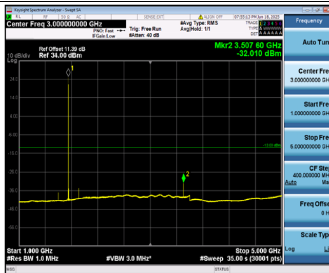
Band4-1.4MHz-QPSK-20393-1-0-High-1000-5000--32.01-PASS
