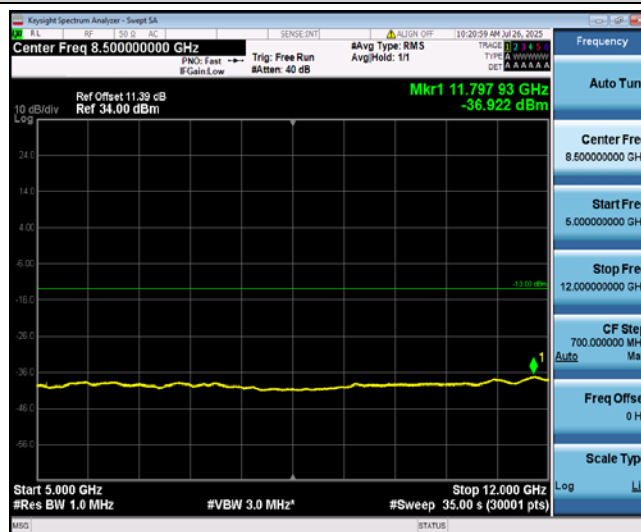
Band4-5MHz-QPSK-19975-1-0-Low-5000-12000--36.92-PASS
