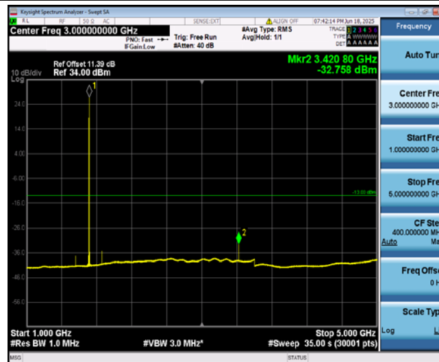
Band4-1.4MHz-QPSK-19957-1-0-Low-1000-5000--32.76-PASS
