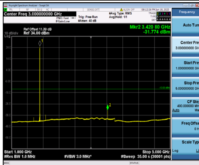
Band4-3MHz-QPSK-19965-1-0-Low-1000-5000--31.77-PASS
