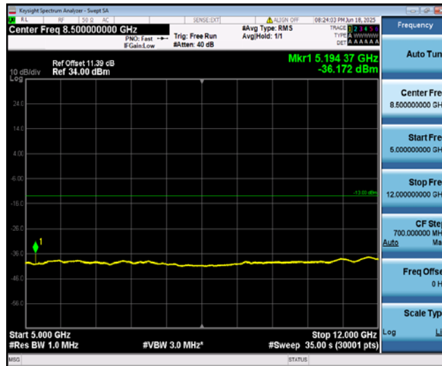
Band4-3MHz-16QAM-20175-1-0-Low-5000-12000--36.17-PASS
