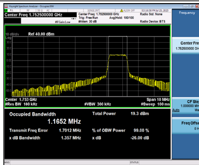
Band4-5MHz-QPSK-20375-6-0-High-1.1652-1.165-PASS
