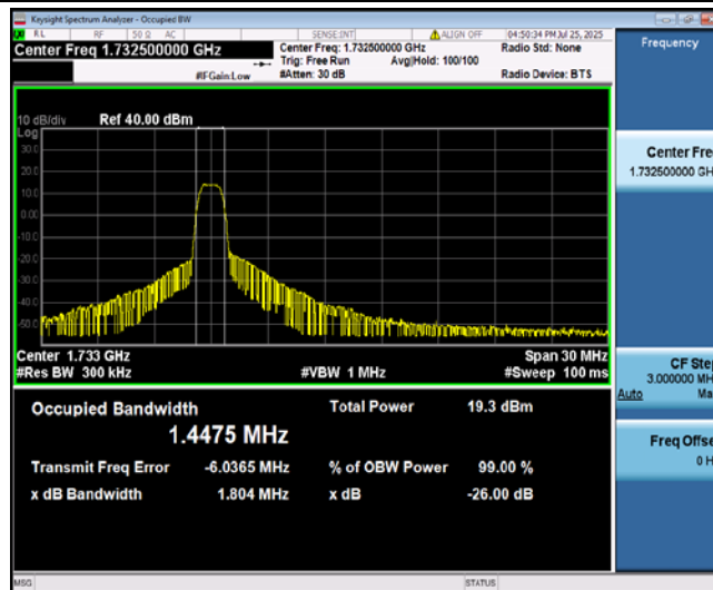
Band4-15MHz-QPSK-20175-6-0-Low-1.4475-1.447-PASS
