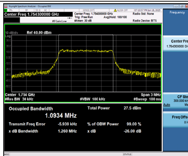
Band4-1.4MHz-QPSK-20393-6-0-High-1.0934-1.093-PASS
