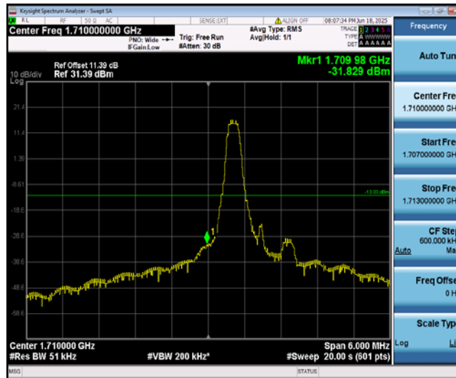
Band4-3MHz-16QAM-19965-1-0-Low--31.83-PASS
