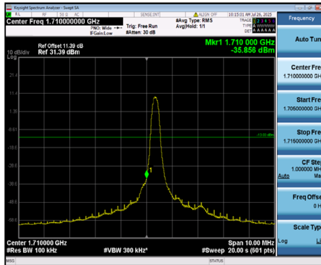
Band4-5MHz-QPSK-19975-1-0-Low--35.86-PASS
