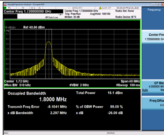
Band4-20MHz-QPSK-20050-6-0-Low-1.8000-1.800-PASS
