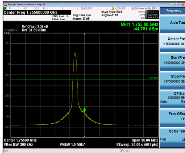
Band4-15MHz-QPSK-20325-1-0-High--44.75-PASS
