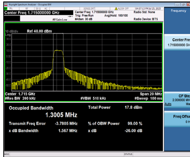
Band4-10MHz-QPSK-20000-6-0-Low-1.3005-1.300-PASS
