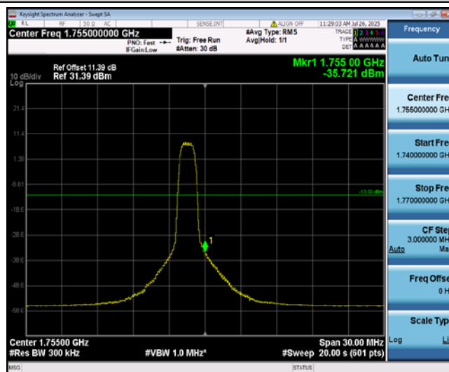
Band4-15MHz-QPSK-20325-6-0-High--35.72-PASS
