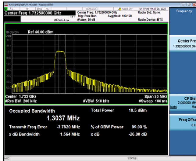
Band4-10MHz-QPSK-20175-6-0-Low-1.3037-1.304-PASS
