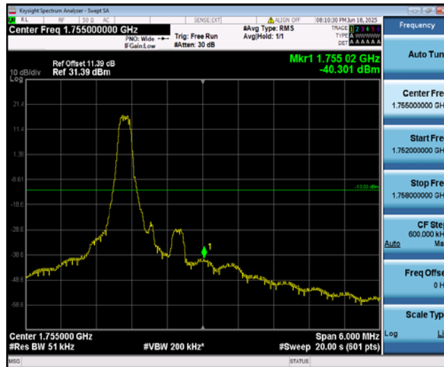
Band4-3MHz-QPSK-20385-1-0-High--40.30-PASS
