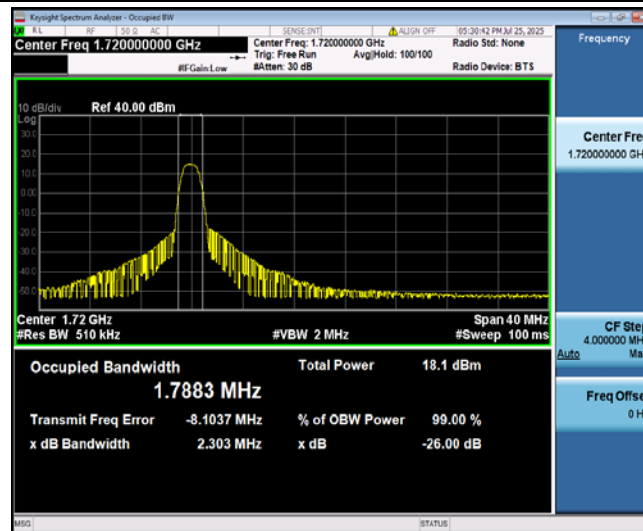
Band4-20MHz-16QAM-20050-6-0-Low-1.7883-1.788-PASS
