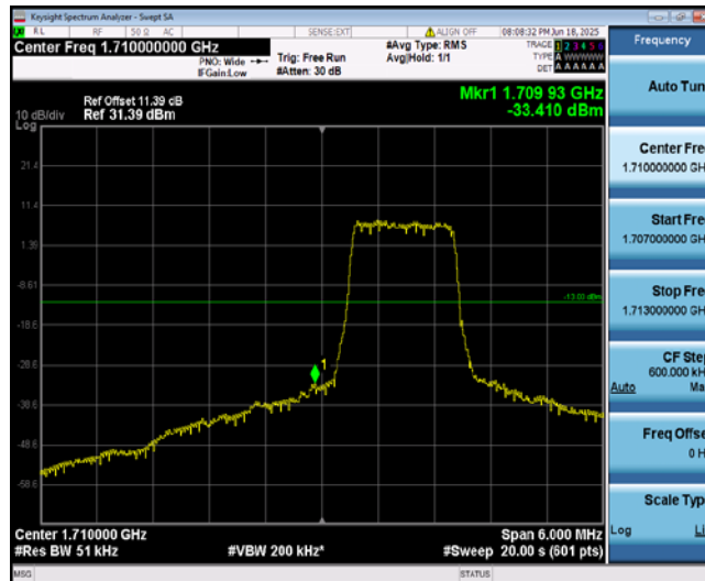
Band4-3MHz-16QAM-19965-6-0-Low--33.41-PASS
