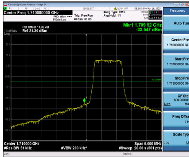
Band4-3MHz-QPSK-19965-6-0-Low--33.55-PASS
