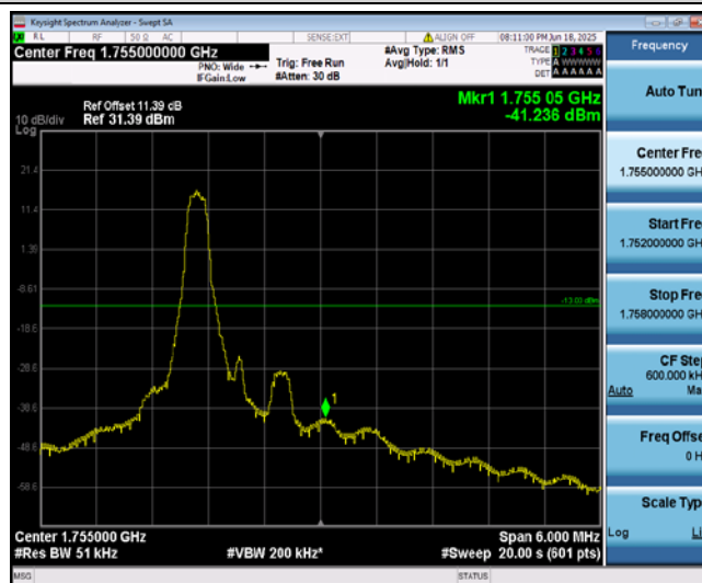
Band4-3MHz-16QAM-20385-1-0-High--41.24-PASS
