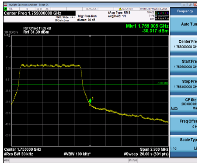
Band4-1.4MHz-16QAM-20393-6-0-High--30.32-PASS
