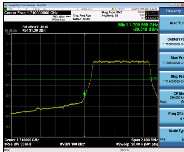
Band4-1.4MHz-QPSK-19957-6-0-Low--29.52-PASS
