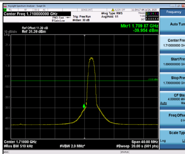
Band4-20MHz-QPSK-20050-6-0-Low--39.95-PASS
