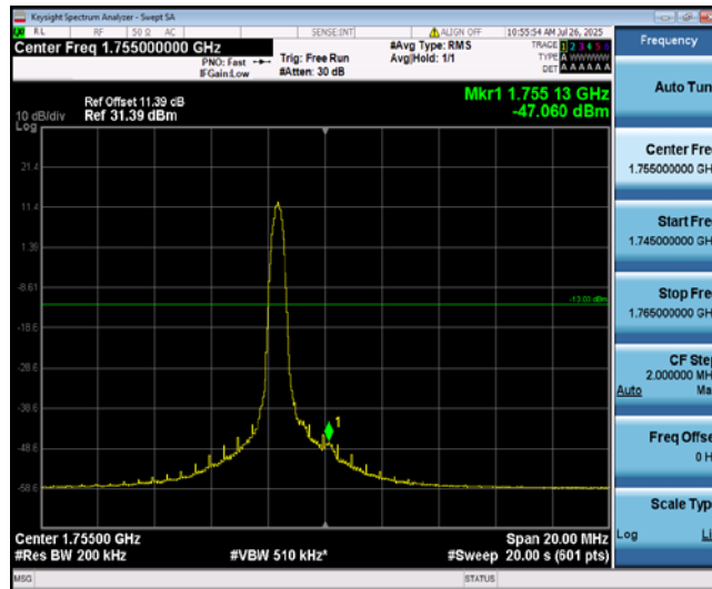
Band4-10MHz-16QAM-20350-1-0-High--47.06-PASS
