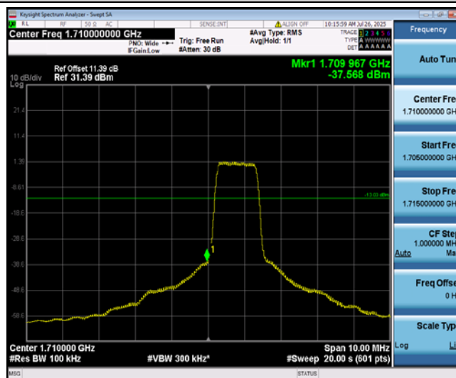
Band4-5MHz-QPSK-19975-6-0-Low--37.57-PASS
