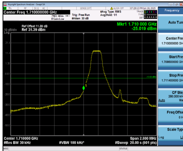
Band4-1.4MHz-16QAM-19957-1-0-Low--25.02-PASS
