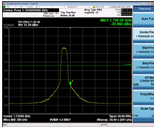
Band4-15MHz-16QAM-20325-6-0-High--35.56-PASS
