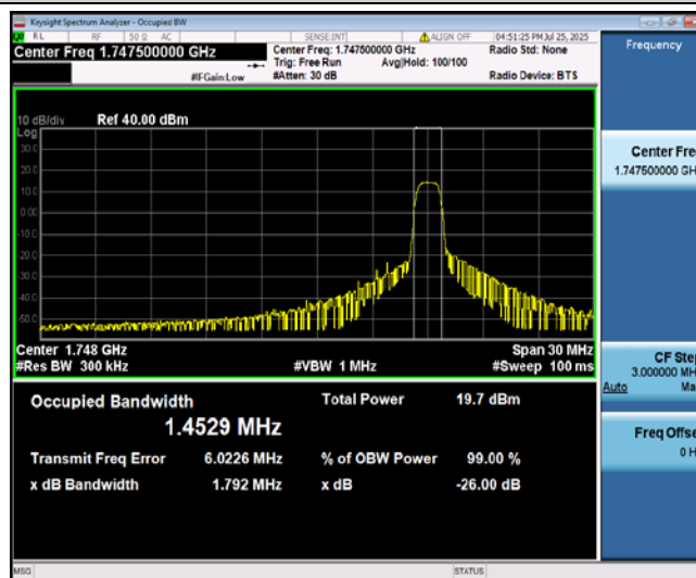
Band4-15MHz-16QAM-20325-6-0-High-1.4529-1.453-PASS
