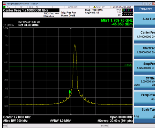
Band4-15MHz-16QAM-20025-1-0-Low--45.06-PASS
