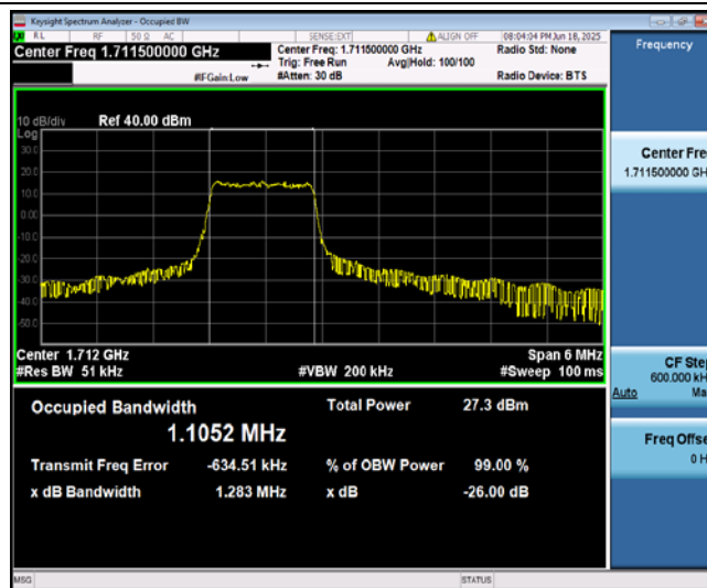
Band4-3MHz-16QAM-19965-6-0-Low-1.1052-1.105-PASS
