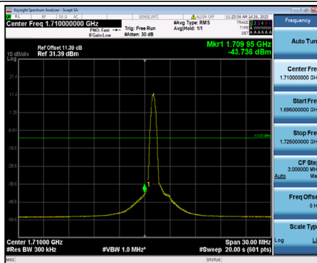
Band4-15MHz-QPSK-20025-1-0-Low--43.74-PASS
