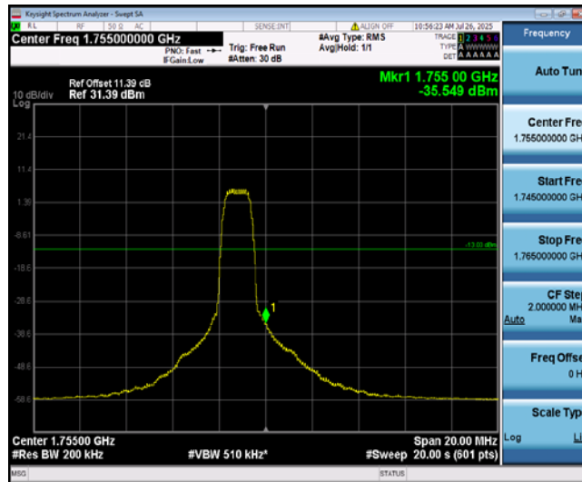
Band4-10MHz-QPSK-20350-6-0-High--35.55-PASS
