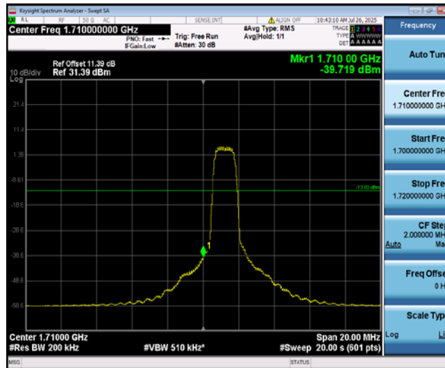
Band4-10MHz-QPSK-20000-6-0-Low--39.72-PASS
