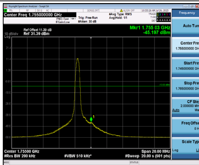
Band4-10MHz-QPSK-20350-1-0-High--45.20-PASS
