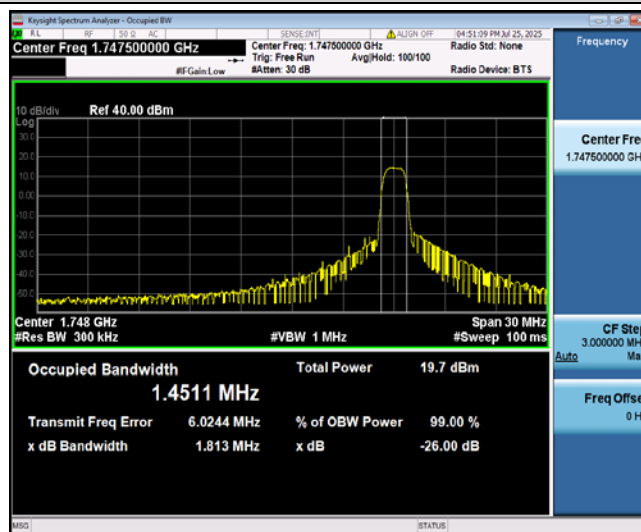
Band4-15MHz-QPSK-20325-6-0-High-1.4511-1.451-PASS
