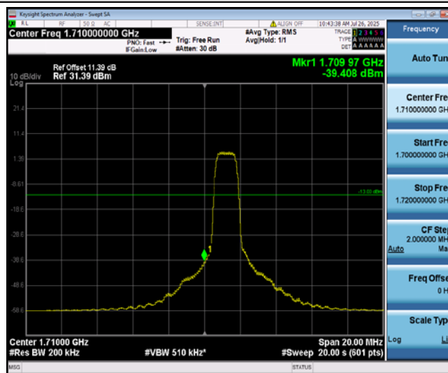
Band4-10MHz-16QAM-20000-6-0-Low--39.41-PASS
