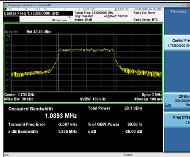
Band4-1.4MHz-16QAM-20175-6-0-Low-1.0893-1.089-PASS
