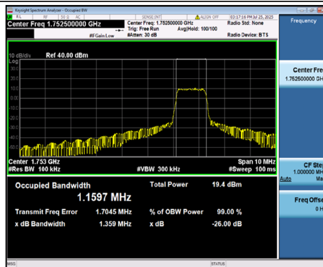
Band4-5MHz-16QAM-20375-6-0-High-1.1597-1.160-PASS
