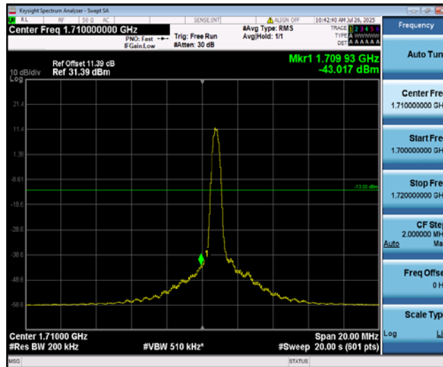
Band4-10MHz-16QAM-20000-1-0-Low--43.02-PASS
