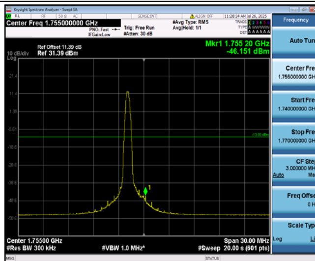
Band4-15MHz-16QAM-20325-1-0-High--46.15-PASS
