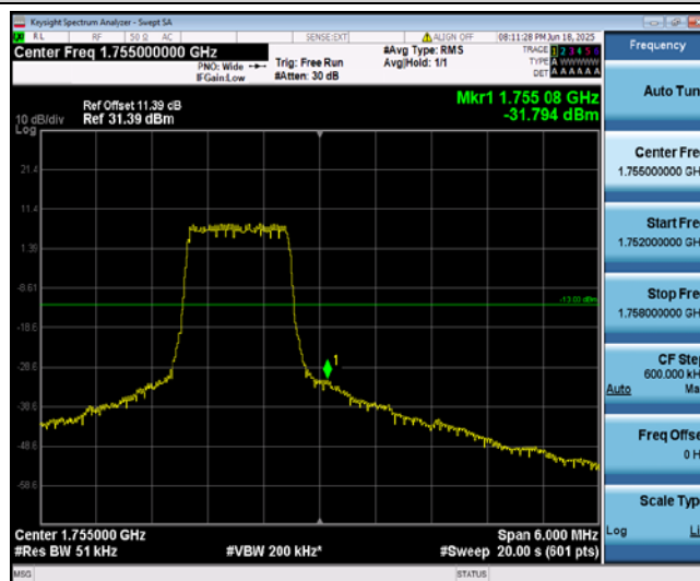
Band4-3MHz-QPSK-20385-6-0-High--31.79-PASS
