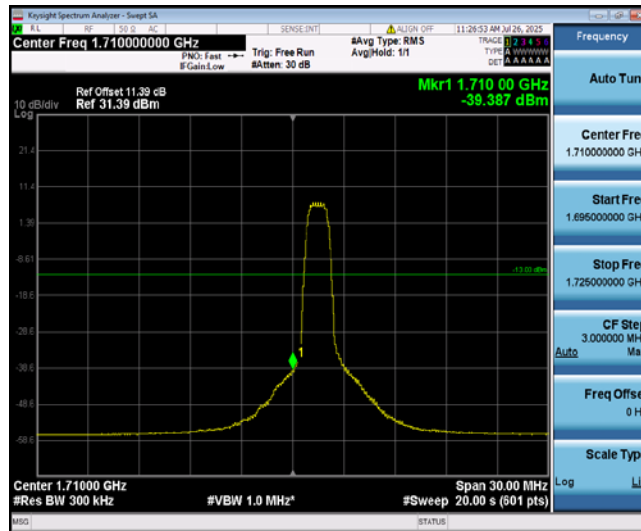
Band4-15MHz-QPSK-20025-6-0-Low--39.39-PASS
