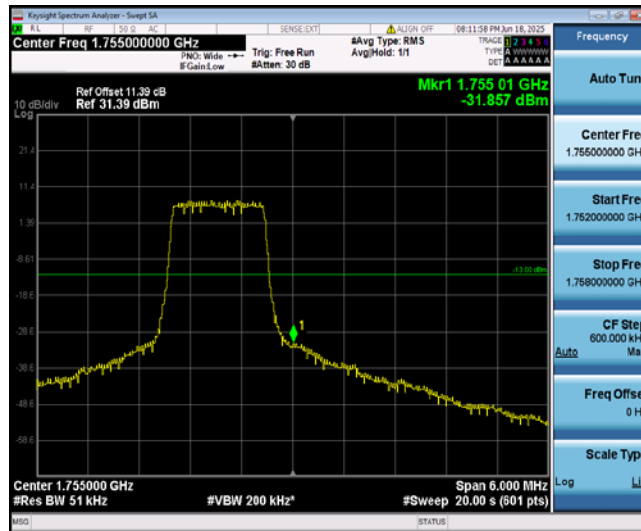
Band4-3MHz-16QAM-20385-6-0-High--31.86-PASS
