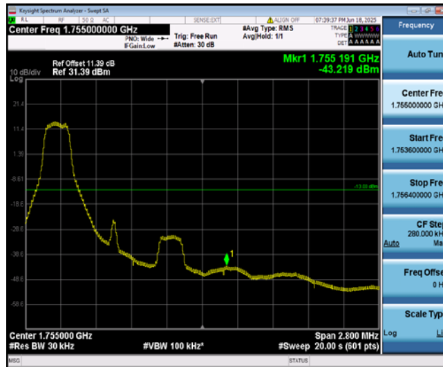
Band4-1.4MHz-16QAM-20393-1-0-High--43.22-PASS
