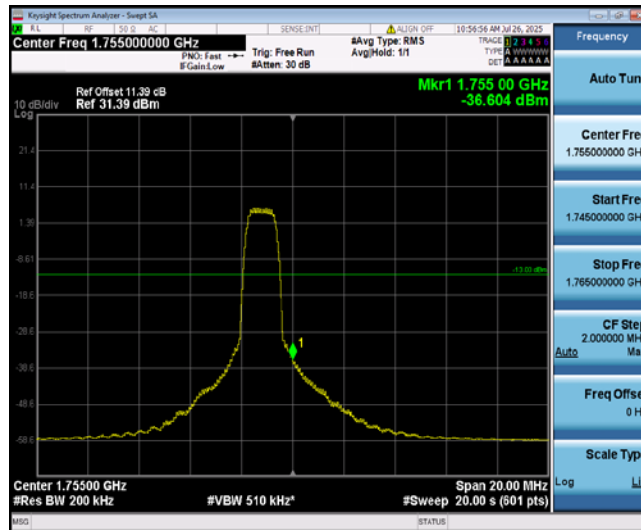
Band4-10MHz-16QAM-20350-6-0-High--36.60-PASS
