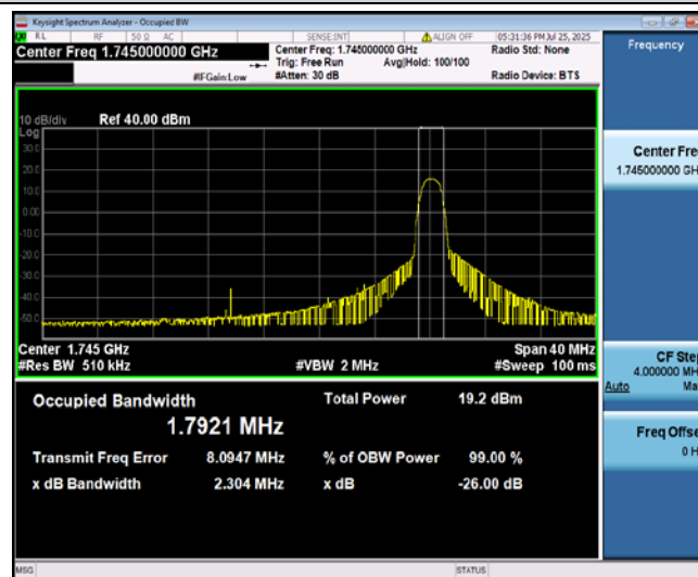
Band4-20MHz-QPSK-20300-6-0-High-1.7921-1.792-PASS
