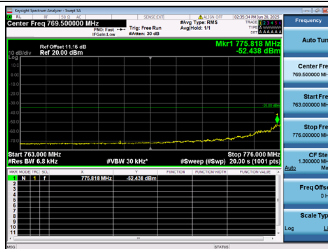
Band13-10MHz-16QAM-23230-1-0-Middle--52.438-PASS
