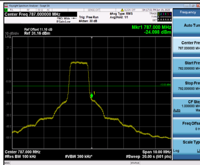
Band13-5MHz-16QAM-23255-6-0-High--24.10-PASS
