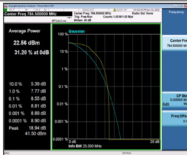
Band13-5MHz-QPSK-23255-6-0-High-8.55-<=13-PASS
