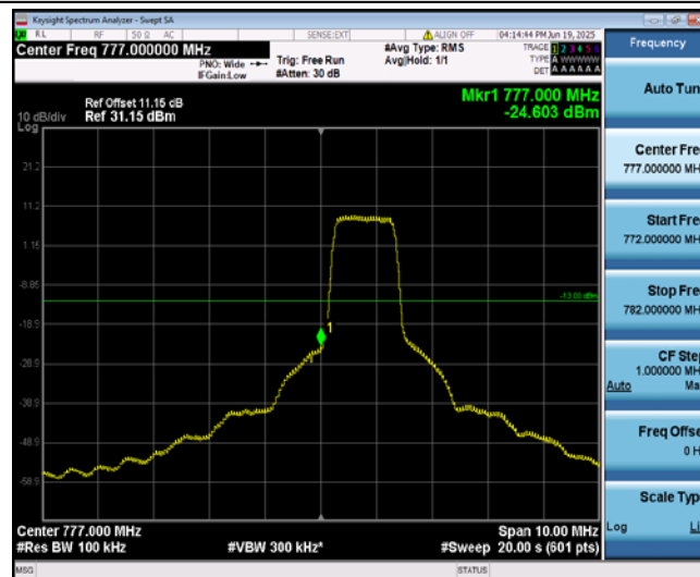
Band13-5MHz-16QAM-23205-6-0-Low--24.60-PASS
