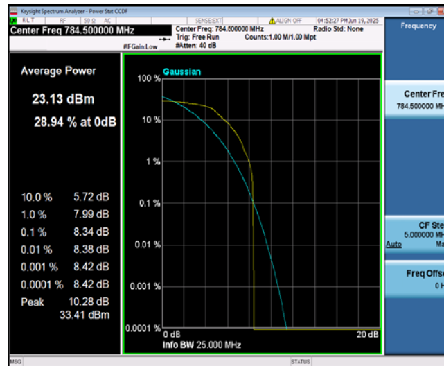
Band13-5MHz-QPSK-23255-1-0-High-8.34-<=13-PASS
