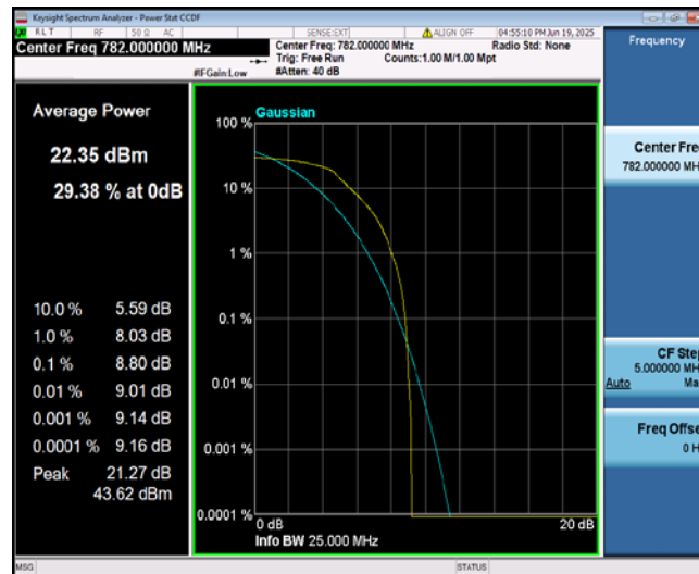
Band13-10MHz-QPSK-23230-6-0-Low-8.80-<=13-PASS
