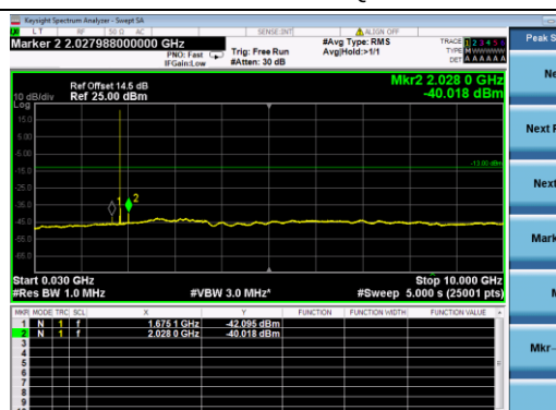
B2-20M-Low CH-CSE-1-QPSK-1 RB 0
