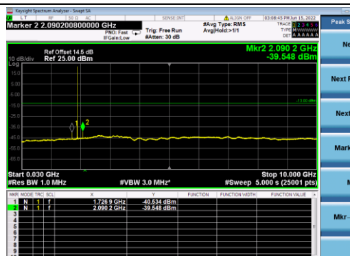
B2-20M-High CH-CSE-2-QPSK-1 RB 0
