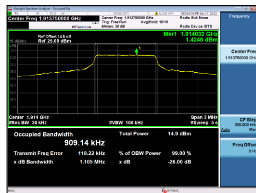
B25-10M-Low CH-OBW-Q16
