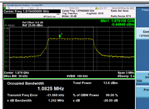
B2-3M-Mid CH-OBW-QPSK
