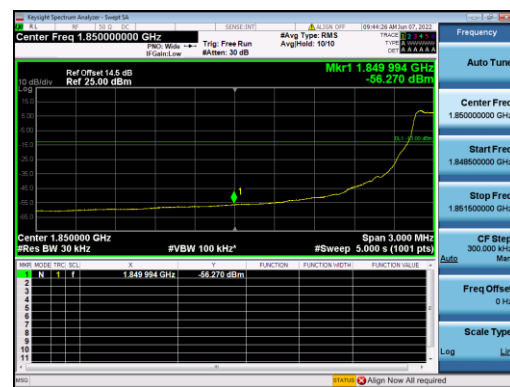
B2-20M-Low CH-BE-QPSK-1 RB 0
