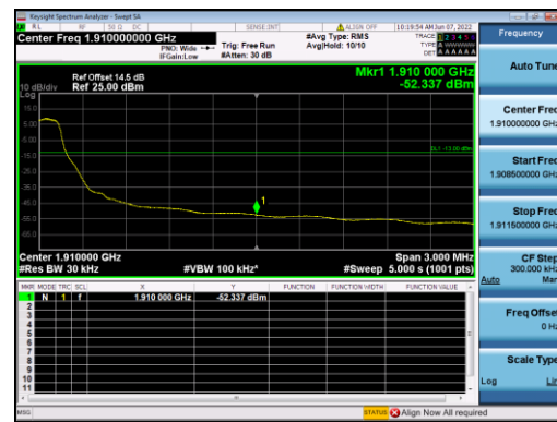
B2-20M-High CH-BE-QPSK-1 RB MAX
