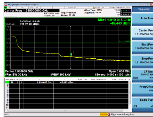
B2-20M-High CH-BE-QPSK-Full RB 0
