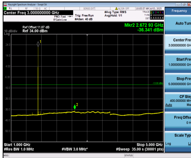
Band66-15MHz-QPSK-132047-1-0-Low-1000-5000--36.34-PASS
