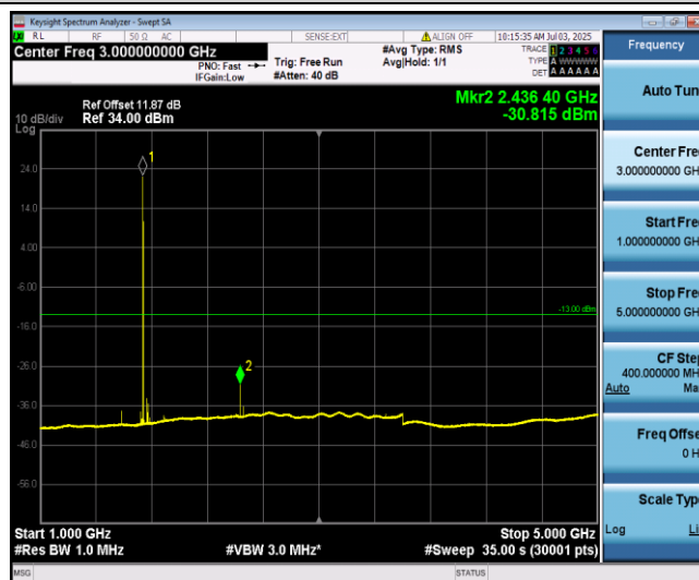
Band66-15MHz-16QAM-132322-1-0-Low-1000-5000--30.82-PASS
