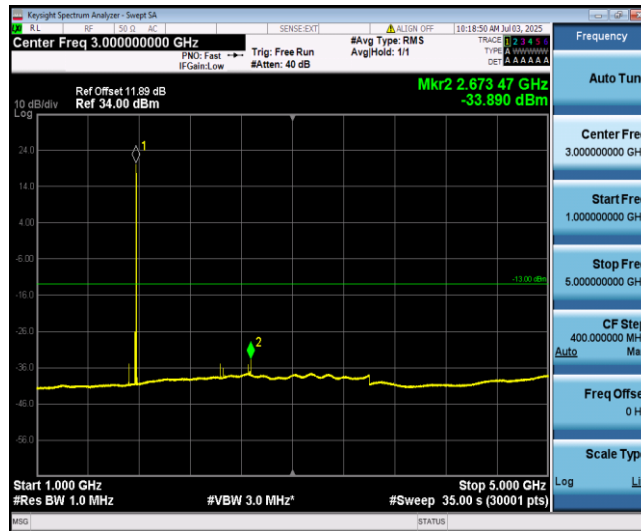
Band66-15MHz-QPSK-132597-1-0-High-1000-5000--33.89-PASS
