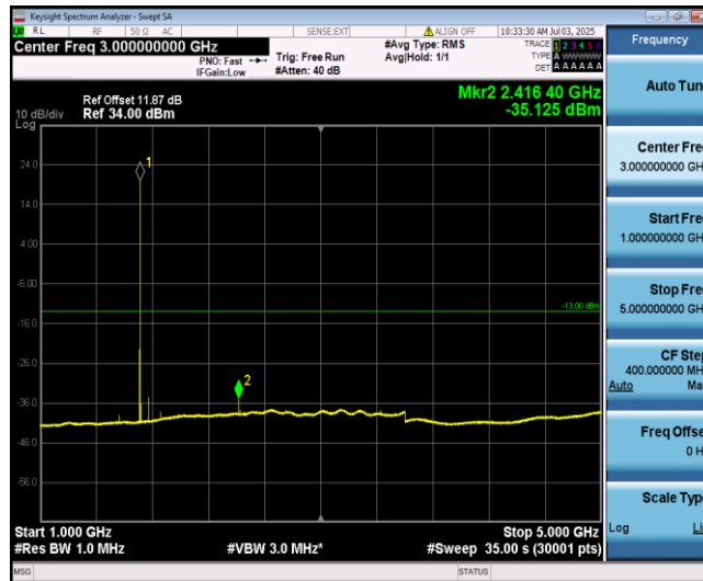
Band66-20MHz-16QAM-132072-1-0-Low-1000-5000--35.13-PASS
