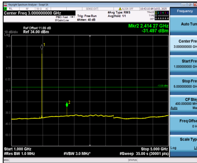
Band66-20MHz-QPSK-132572-1-0-High-1000-5000--31.5-PASS
