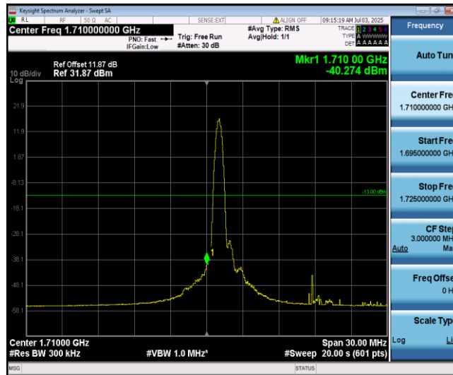
Band66-15MHz-16QAM-132047-1-0-Low--40.27-PASS
