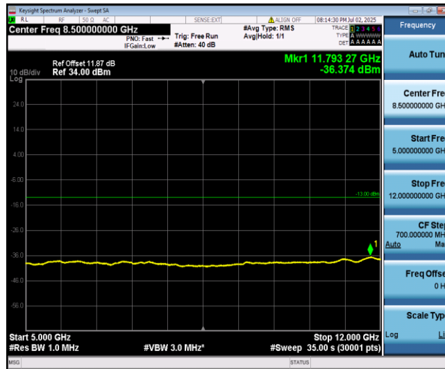
Band66-3MHz-QPSK-132322-1-0-Low-5000-12000--36.37-PASS
