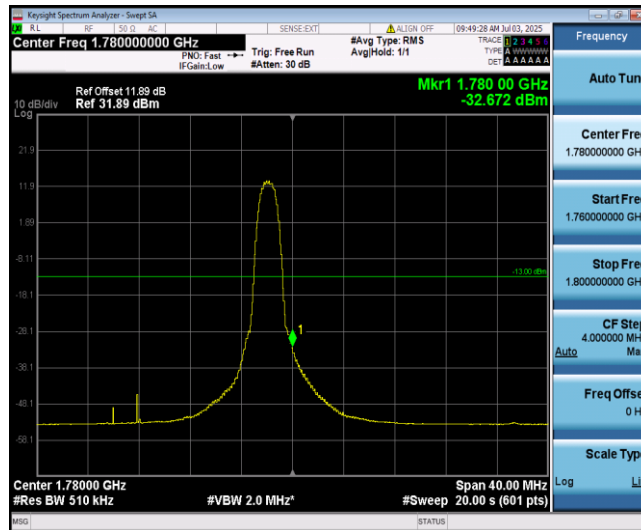
Band66-20MHz-QPSK-132572-6-0-High--32.67-PASS
