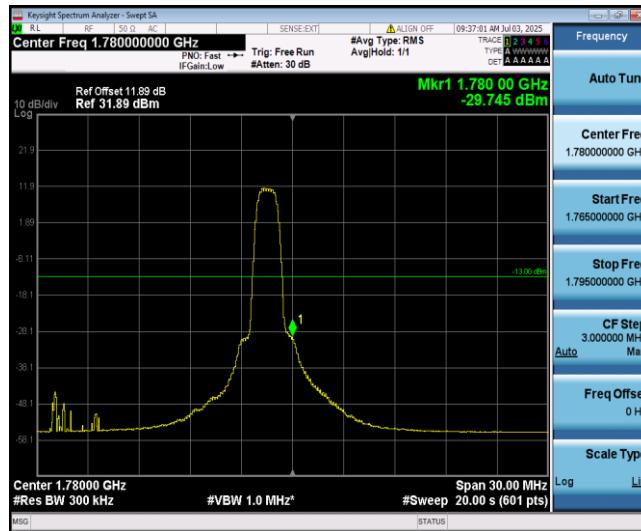
Band66-15MHz-16QAM-132597-6-0-High--29.75-PASS
