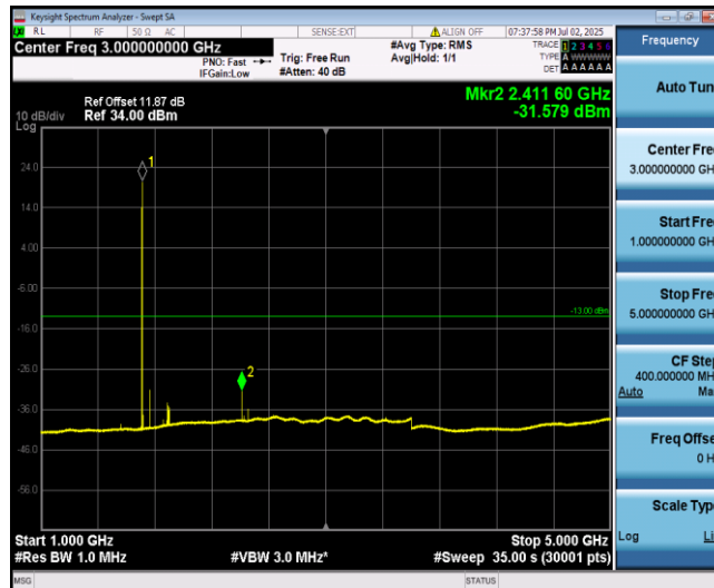
Band66-1.4MHz-16QAM-131979-1-0-Low-1000-5000--31.58-PASS
