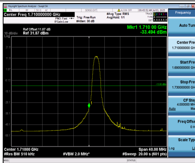
Band66-20MHz-QPSK-132072-6-0-Low--33.49-PASS
