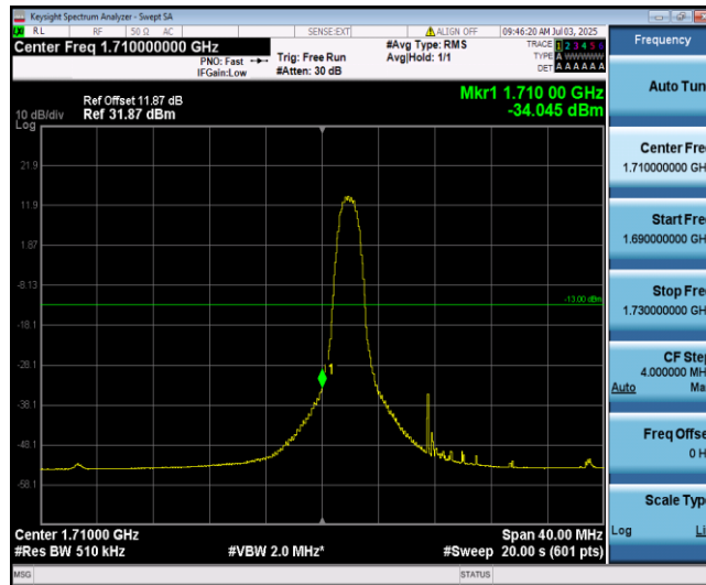
Band66-20MHz-16QAM-132072-6-0-Low--34.05-PASS
