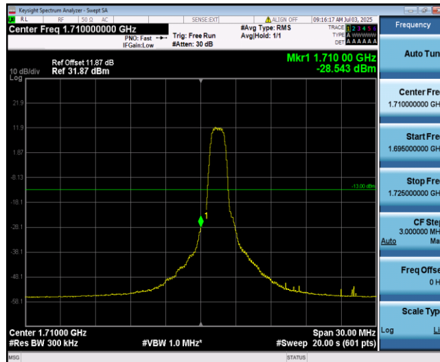
Band66-15MHz-16QAM-132047-6-0-Low--28.54-PASS
