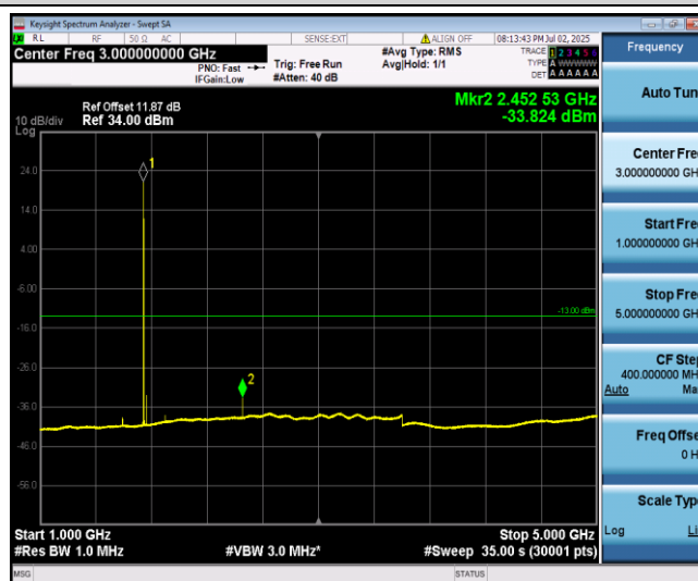
Band66-3MHz-QPSK-132322-1-0-Low-1000-5000--33.82-PASS
