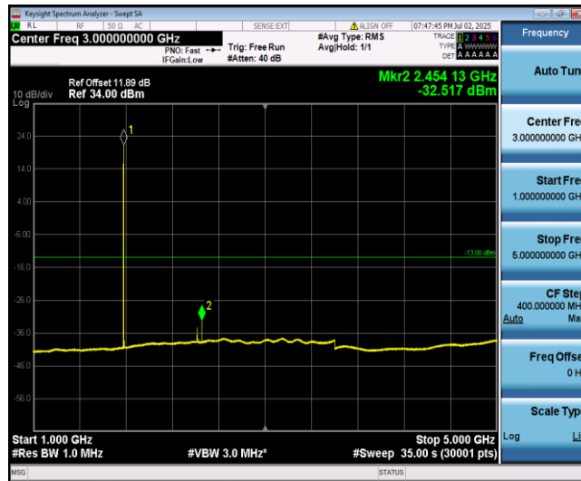
Band66-1.4MHz-QPSK-132665-1-0-High-1000-5000--32.52-PASS
