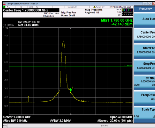
Band66-20MHz-QPSK-132572-1-0-High--42.14-PASS
