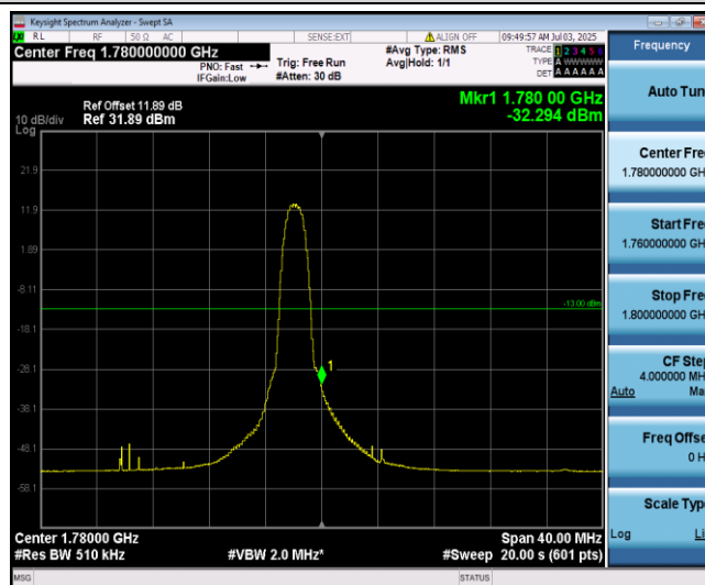
Band66-20MHz-16QAM-132572-6-0-High--32.29-PASS
