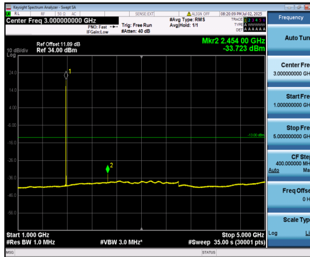
Band66-3MHz-QPSK-132657-1-0-High-1000-5000--33.72-PASS
