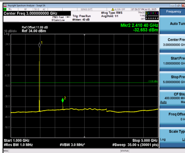
Band66-1.4MHz-16QAM-132665-1-0-High-1000-5000--32.65-PASS
