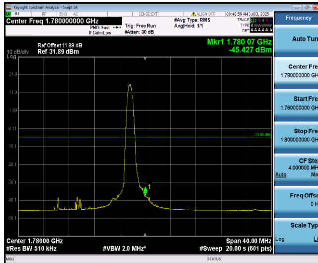
Band66-20MHz-16QAM-132572-1-0-High--45.43-PASS
