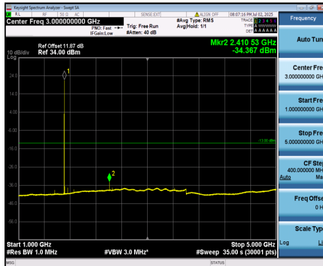
Band66-3MHz-QPSK-131987-1-0-Low-1000-5000--34.37-PASS
