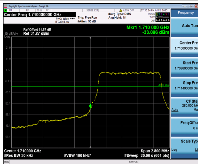
Band66-1.4MHz-16QAM-131979-6-0-Low--33.10-PASS
