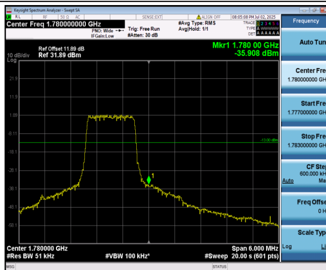
Band66-3MHz-QPSK-132657-6-0-High--35.91-PASS
