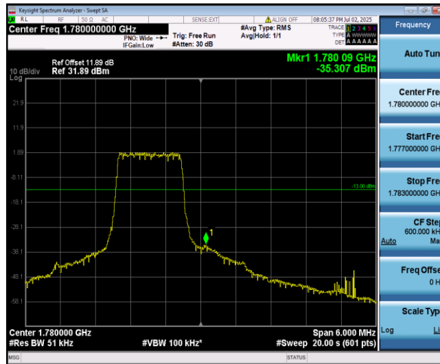
Band66-3MHz-16QAM-132657-6-0-High--35.31-PASS
