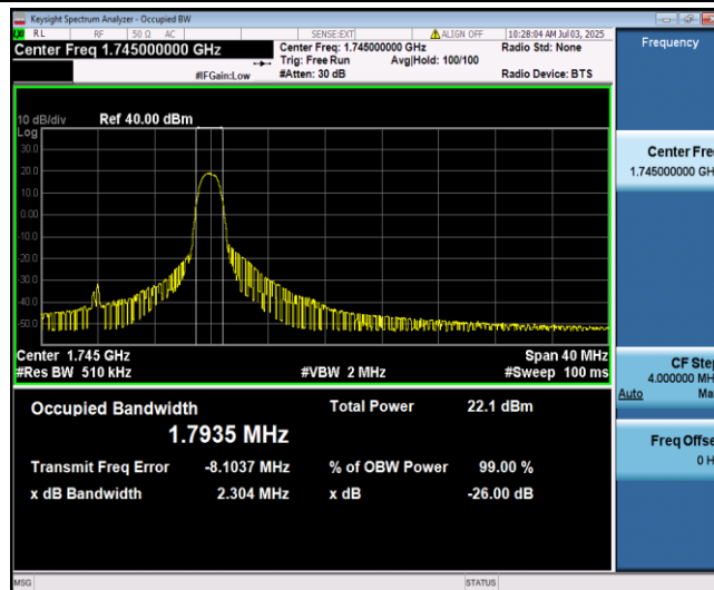
Band66-20MHz-16QAM-132322-6-0-Low-1.7935-1.794-PASS
