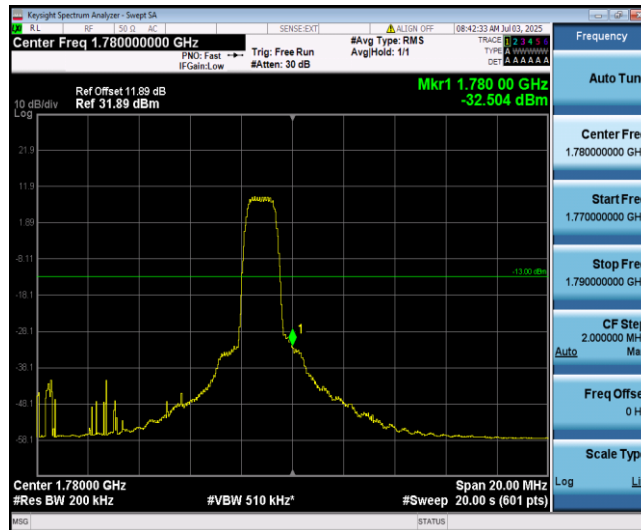
Band66-10MHz-16QAM-132622-6-0-High--32.50-PASS
