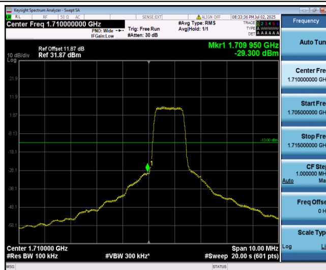
Band66-5MHz-QPSK-131997-6-0-Low--29.30-PASS
