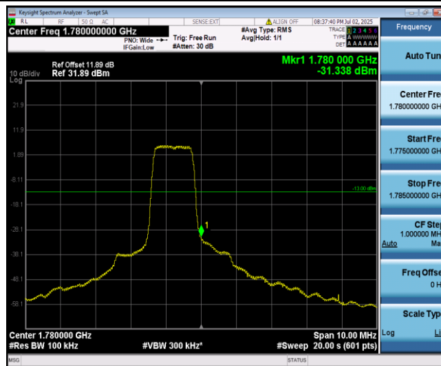
Band66-5MHz-16QAM-132647-6-0-High--31.34-PASS
