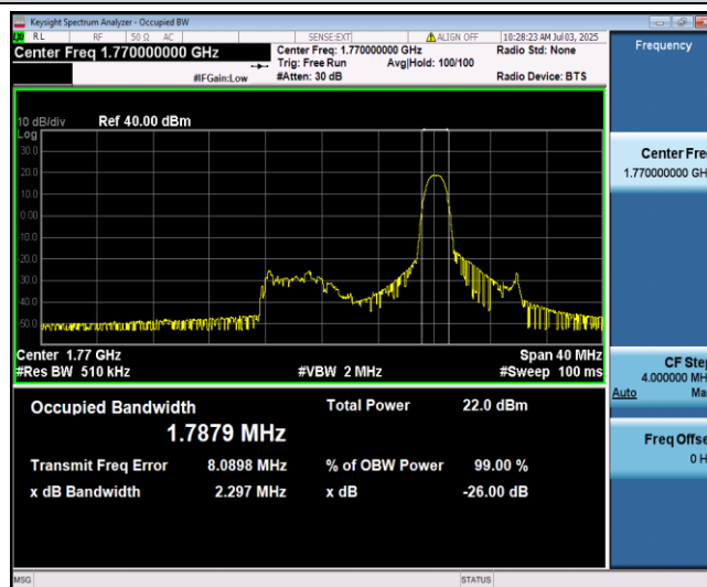
Band66-20MHz-QPSK-132572-6-0-High-1.7879-1.788-PASS
