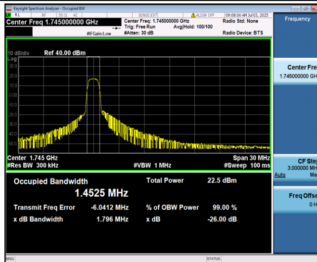
Band66-15MHz-16QAM-132322-6-0-Low-1.4525-1.453-PASS
