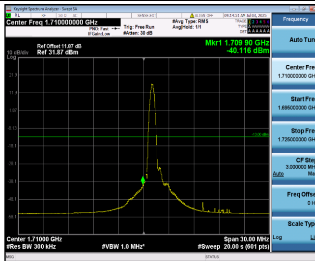
Band66-15MHz-QPSK-132047-1-0-Low--40.12-PASS
