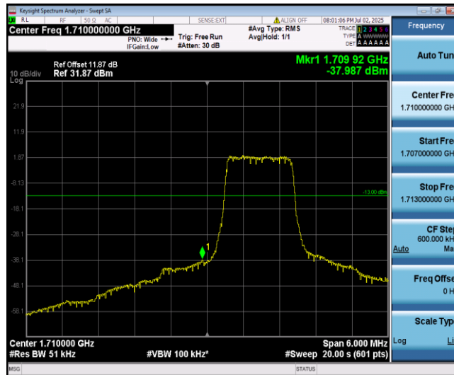
Band66-3MHz-16QAM-131987-6-0-Low--37.99-PASS
