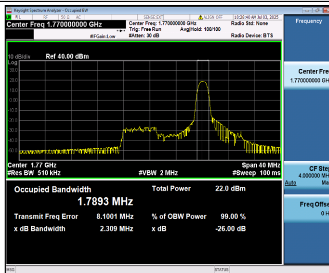
Band66-20MHz-16QAM-132572-6-0-High-1.7893-1.789-PASS
