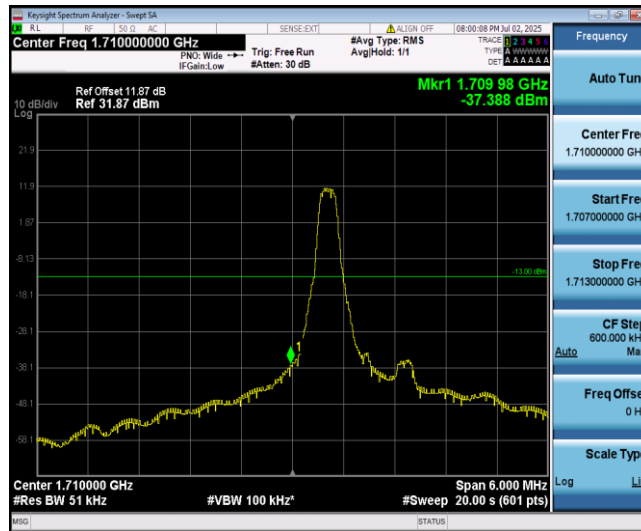
Band66-3MHz-16QAM-131987-1-0-Low--37.39-PASS
