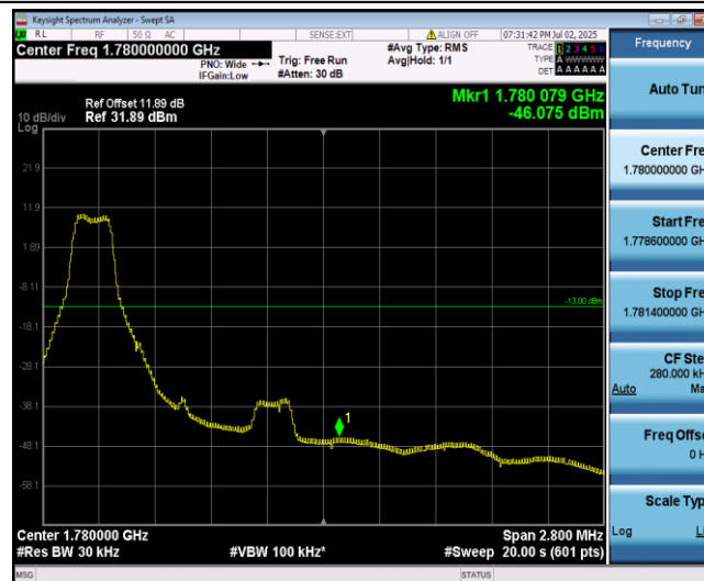
Band66-1.4MHz-QPSK-132665-1-0-High--46.07-PASS
