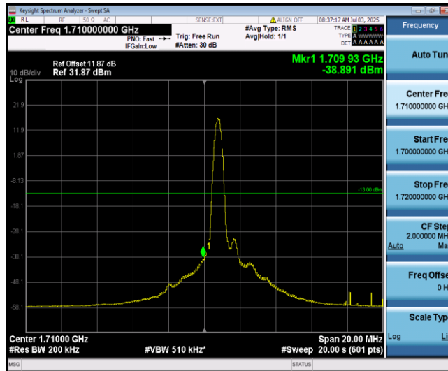
Band66-10MHz-QPSK-132022-1-0-Low--38.89-PASS
