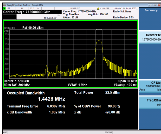
Band66-15MHz-16QAM-132597-6-0-High-1.4428-1.443-PASS
