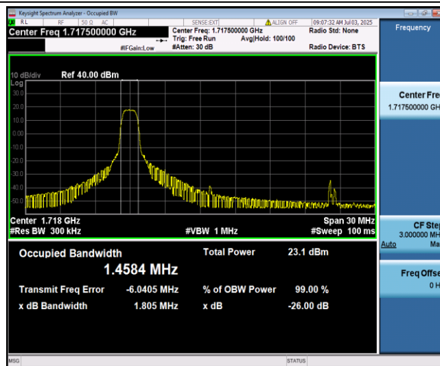
Band66-15MHz-16QAM-132047-6-0-Low-1.4584-1.458-PASS
