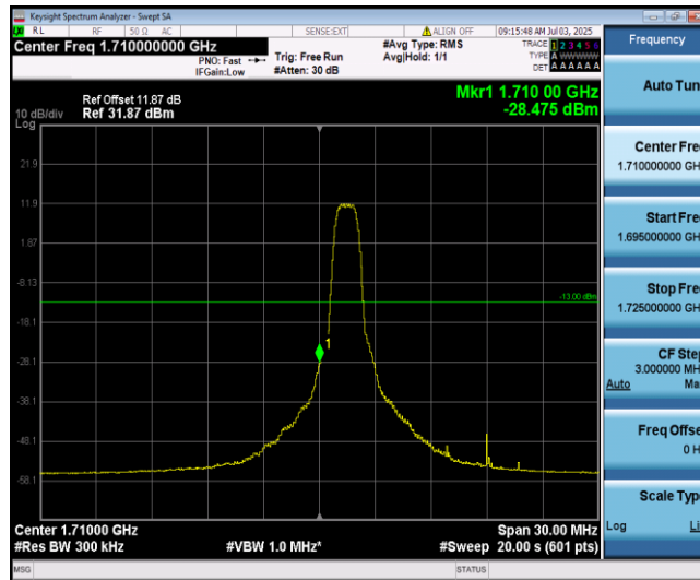
Band66-15MHz-QPSK-132047-6-0-Low--28.48-PASS
