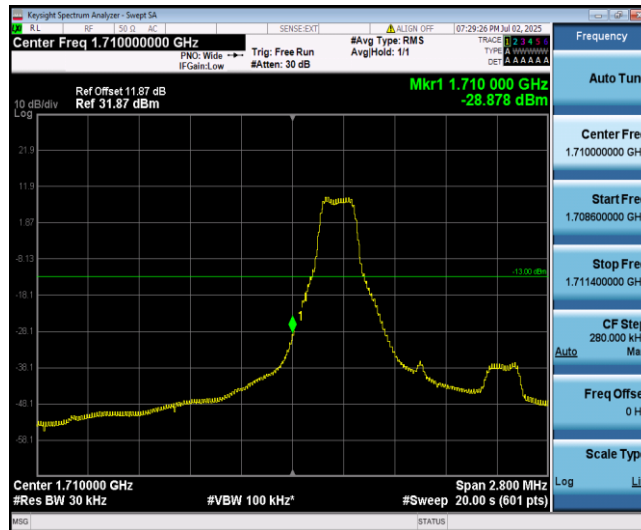
Band66-1.4MHz-16QAM-131979-1-0-Low--28.88-PASS
