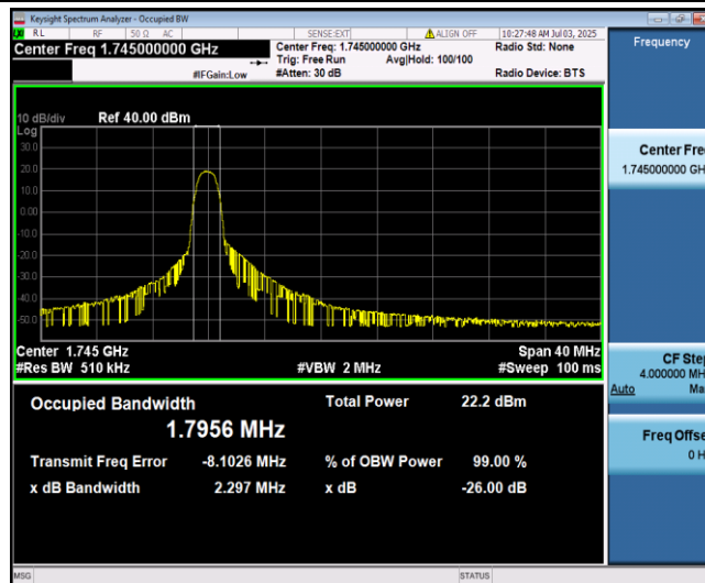
Band66-20MHz-QPSK-132322-6-0-Low-1.7956-1.796-PASS
