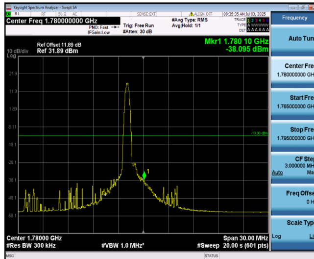
Band66-15MHz-QPSK-132597-1-0-High--38.10-PASS
