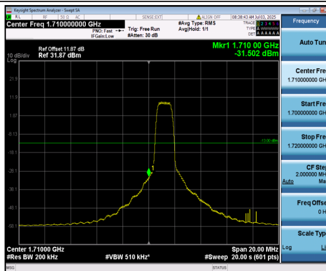
Band66-10MHz-16QAM-132022-6-0-Low--31.50-PASS
