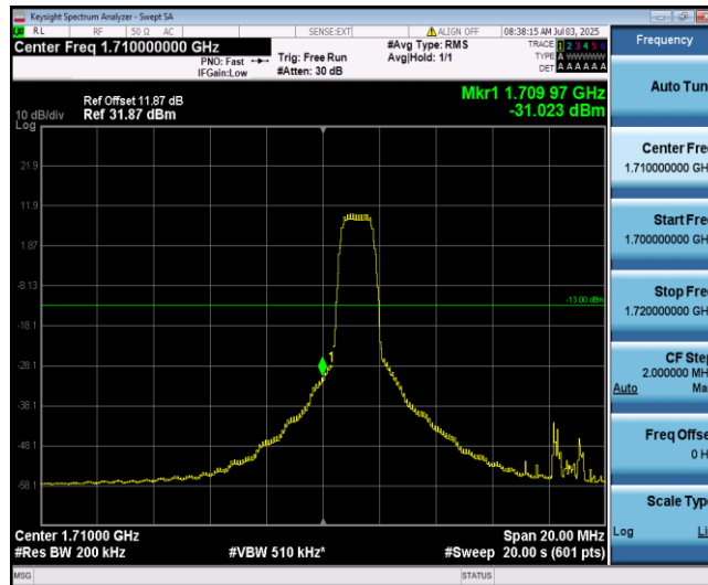
Band66-10MHz-QPSK-132022-6-0-Low--31.02-PASS
