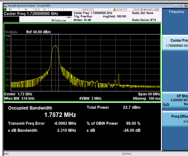
Band66-20MHz-16QAM-132072-6-0-Low-1.7872-1.787-PASS
