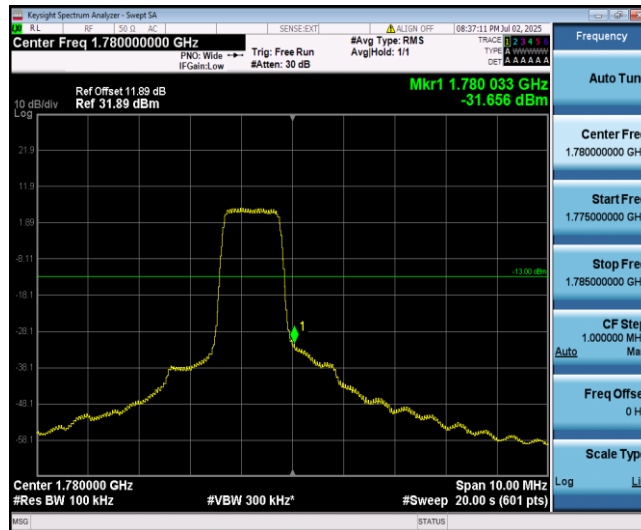
Band66-5MHz-QPSK-132647-6-0-High--31.66-PASS
