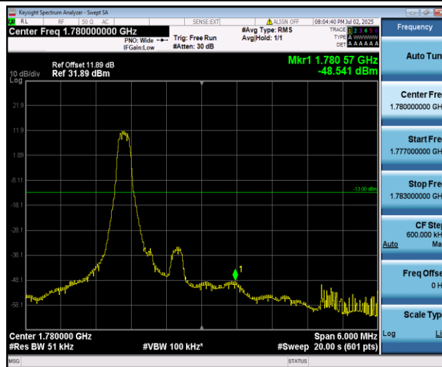
Band66-3MHz-16QAM-132657-1-0-High--48.54-PASS
