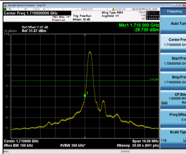
Band66-5MHz-16QAM-131997-1-0-Low--29.73-PASS
