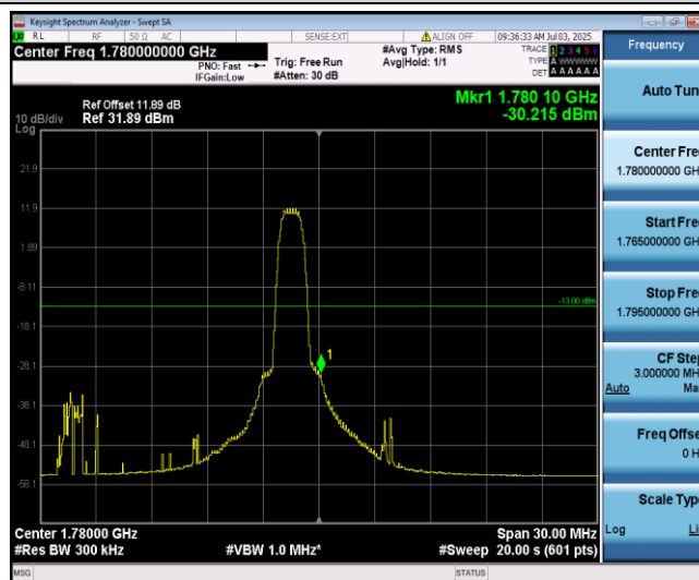
Band66-15MHz-QPSK-132597-6-0-High--30.22-PASS
