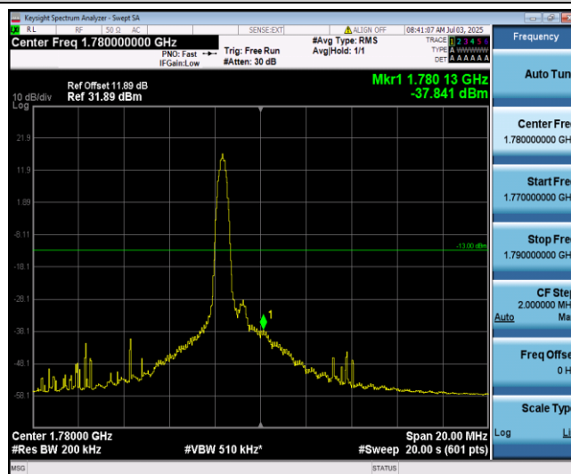
Band66-10MHz-QPSK-132622-1-0-High--37.84-PASS
