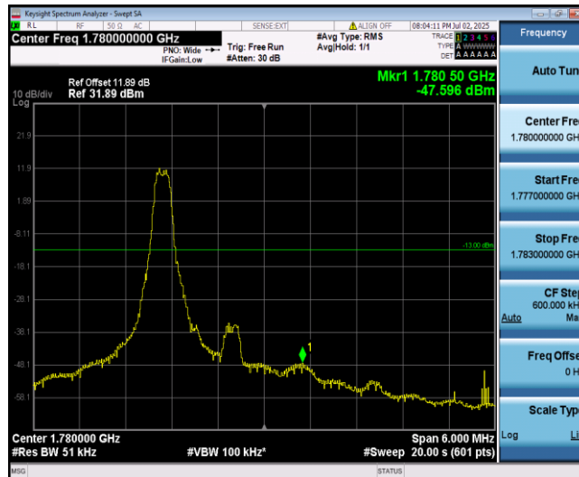
Band66-3MHz-QPSK-132657-1-0-High--47.60-PASS
