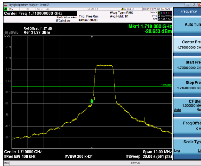
Band66-5MHz-16QAM-131997-6-0-Low--28.65-PASS
