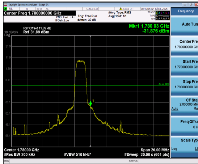
Band66-10MHz-QPSK-132622-6-0-High--31.88-PASS
