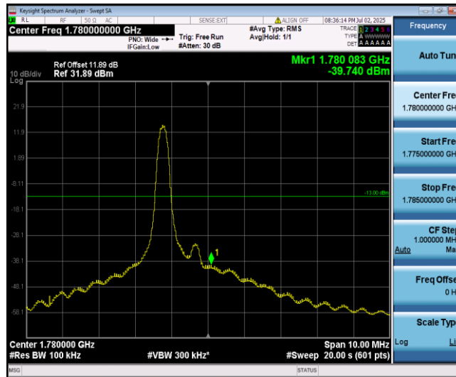
Band66-5MHz-QPSK-132647-1-0-High--39.74-PASS
