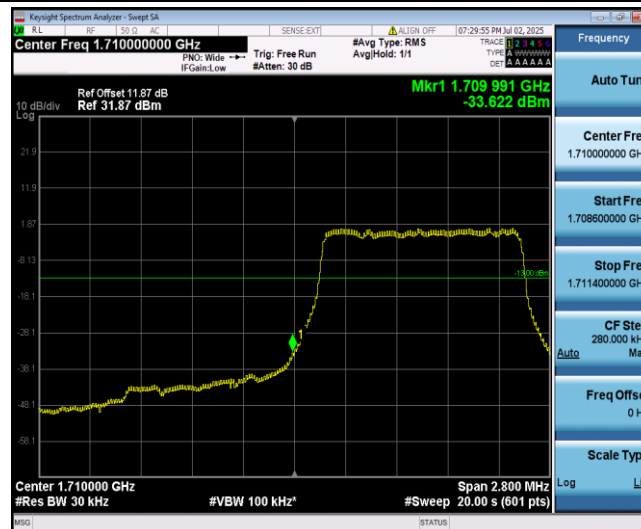
Band66-1.4MHz-QPSK-131979-6-0-Low--33.62-PASS
