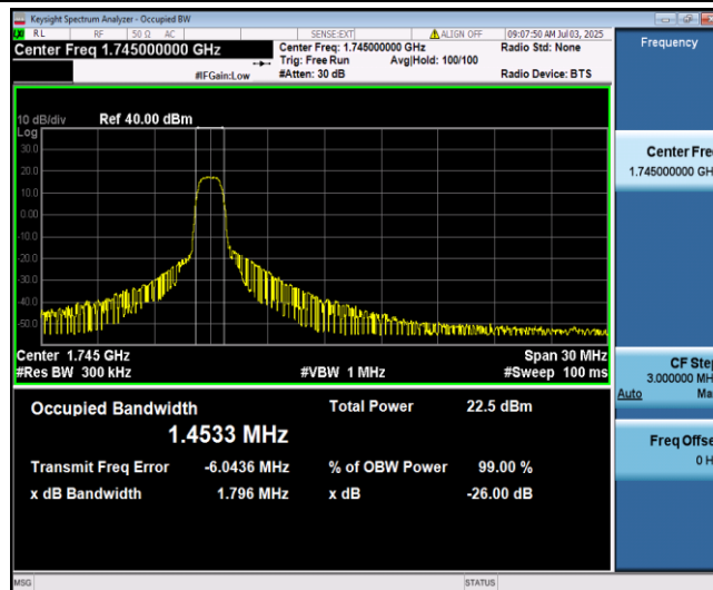
Band66-15MHz-QPSK-132322-6-0-Low-1.4533-1.453-PASS
