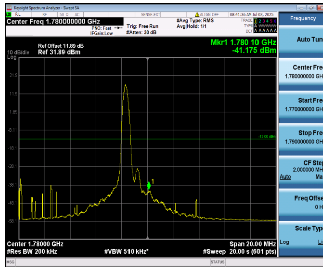
Band66-10MHz-16QAM-132622-1-0-High--41.17-PASS
