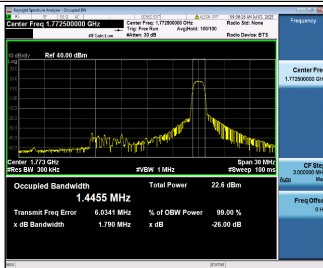
Band66-15MHz-QPSK-132597-6-0-High-1.4455-1.446-PASS
