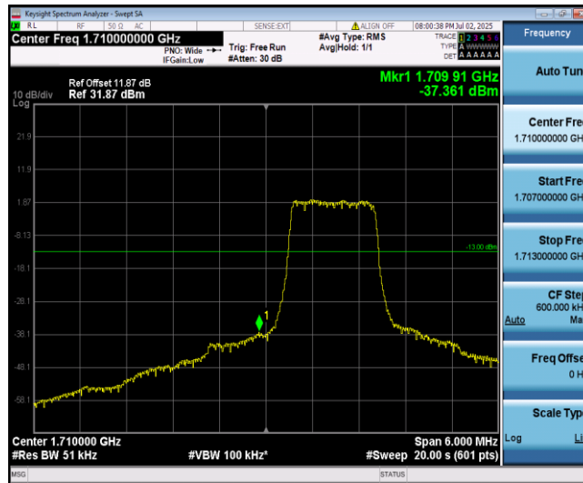
Band66-3MHz-QPSK-131987-6-0-Low--37.36-PASS
