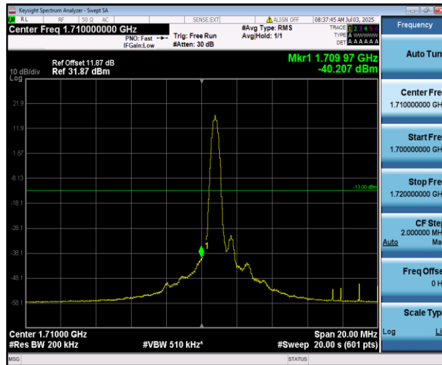
Band66-10MHz-16QAM-132022-1-0-Low--40.21-PASS
