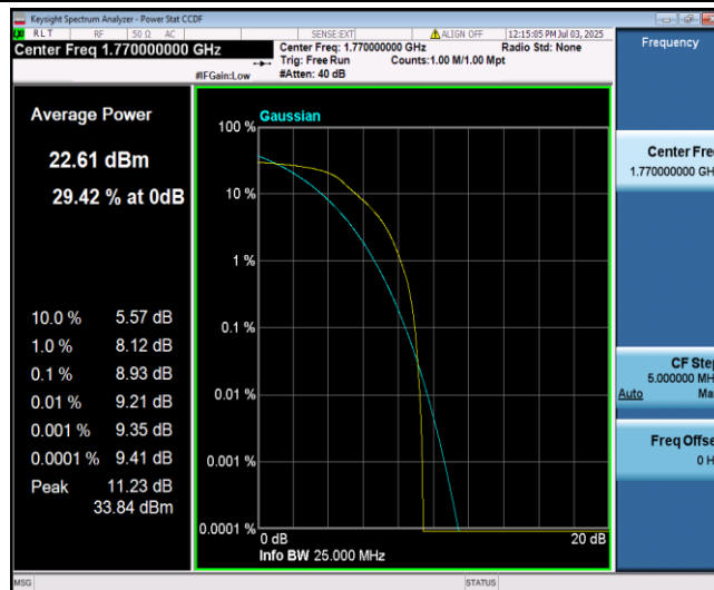
Band66-20MHz-QPSK-132572-6-0-High-8.93-<=13-PASS
