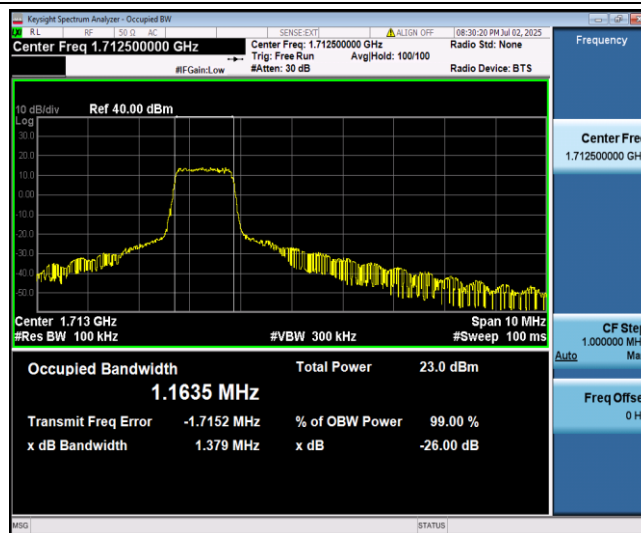
Band66-5MHz-QPSK-131997-6-0-Low-1.1635-1.163-PASS
