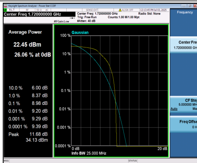
Band66-20MHz-QPSK-132072-6-0-Low-8.98-<=13-PASS
