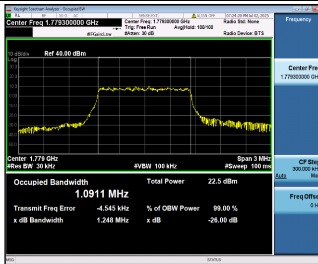
Band66-1.4MHz-16QAM-132665-6-0-High-1.0911-1.091-PASS
