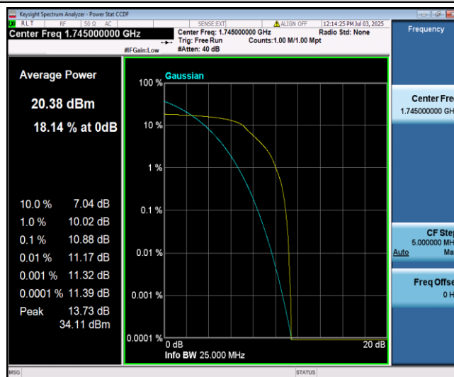
Band66-20MHz-QPSK-132322-6-0-Low-10.88-<=13-PASS
