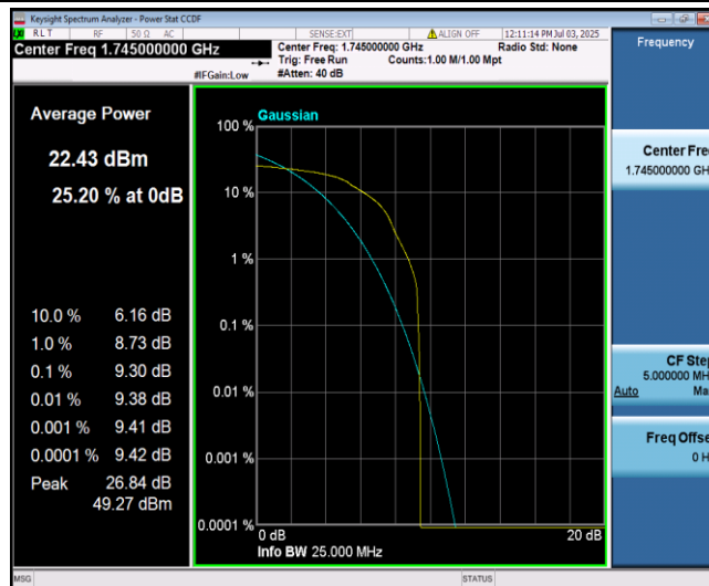
Band66-15MHz-16QAM-132322-1-0-Low-9.30-<=13-PASS
