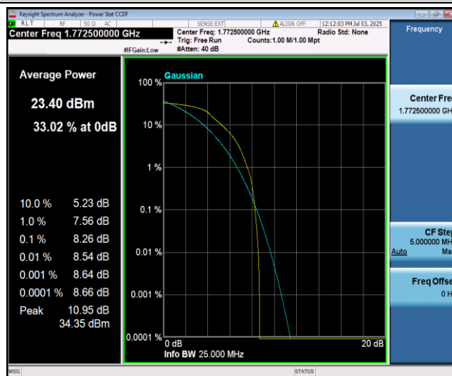
Band66-15MHz-QPSK-132597-6-0-High-8.26-<=13-PASS
