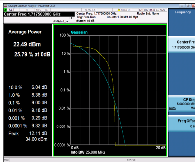
Band66-15MHz-16QAM-132047-6-0-Low-9.00-<=13-PASS
