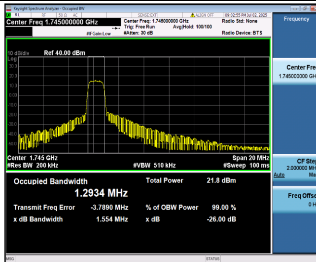
Band66-10MHz-QPSK-132322-6-0-Low-1.2934-1.293-PASS
