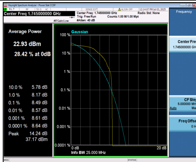
Band66-20MHz-QPSK-132322-1-0-Low-8.49-<=13-PASS
