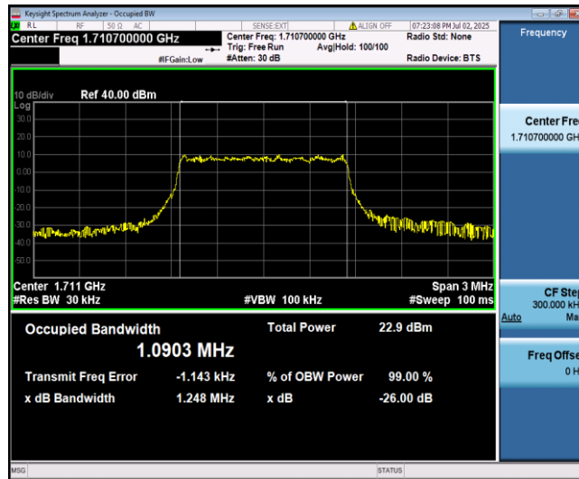
Band66-1.4MHz-16QAM-131979-6-0-Low-1.0903-1.090-PASS
