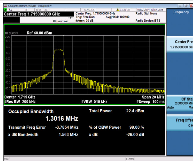
Band66-10MHz-QPSK-132022-6-0-Low-1.3016-1.302-PASS
