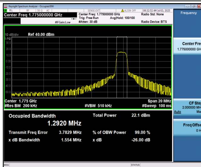
Band66-10MHz-16QAM-132622-6-0-High-1.2920-1.292-PASS
