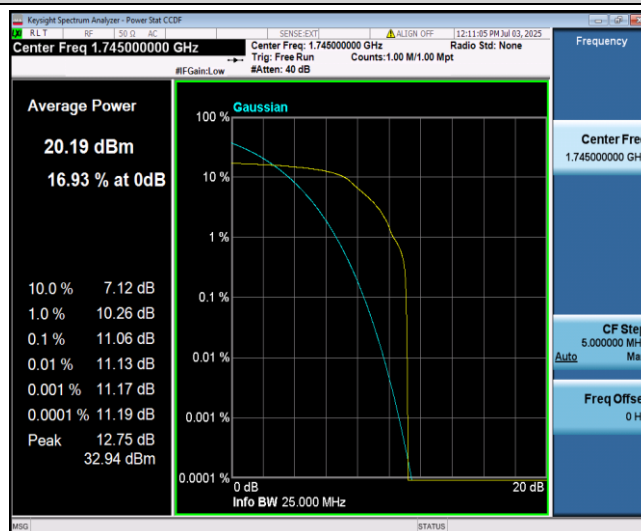
Band66-15MHz-QPSK-132322-1-0-Low-11.06-<=13-PASS
