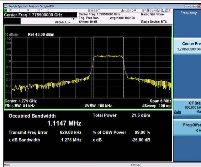
Band66-3MHz-QPSK-132657-6-0-High-1.1147-1.115-PASS
