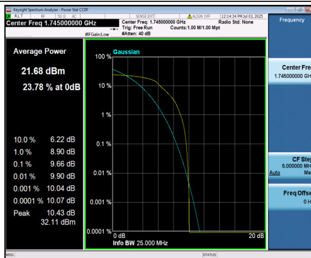
Band66-20MHz-16QAM-132322-6-0-Low-9.66-<=13-PASS
