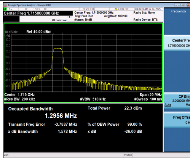
Band66-10MHz-16QAM-132022-6-0-Low-1.2956-1.296-PASS
