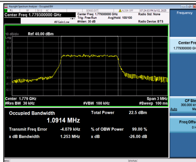
Band66-1.4MHz-QPSK-132665-6-0-High-1.0914-1.091-PASS
