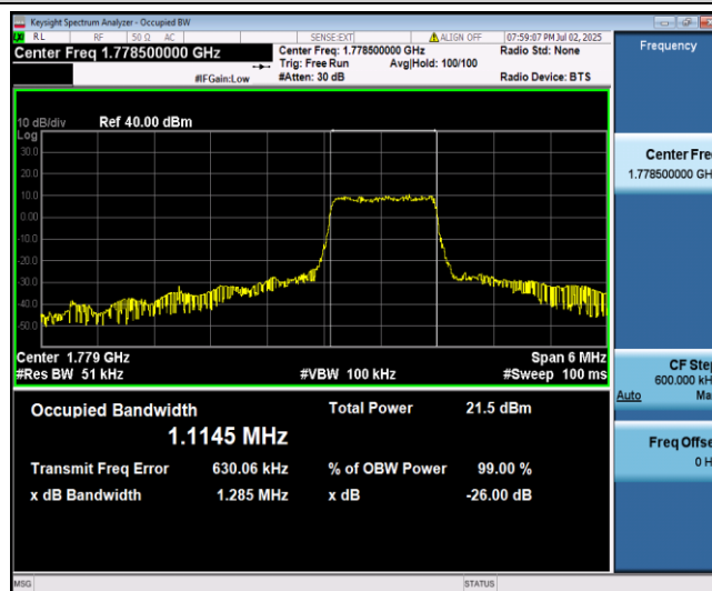
Band66-3MHz-16QAM-132657-6-0-High-1.1145-1.114-PASS
