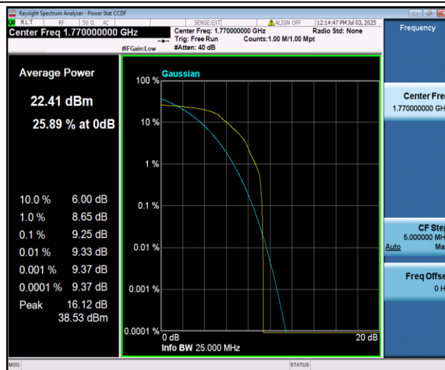
Band66-20MHz-QPSK-132572-1-0-High-9.25-<=13-PASS
