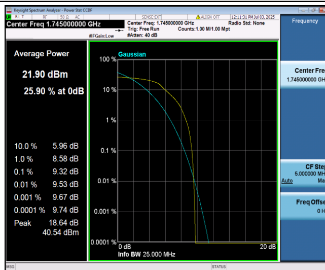
Band66-15MHz-16QAM-132322-6-0-Low-9.32-<=13-PASS
