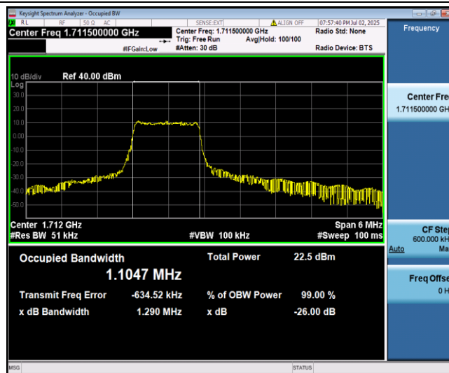
Band66-3MHz-QPSK-131987-6-0-Low-1.1047-1.105-PASS
