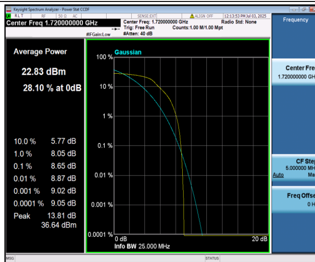
Band66-20MHz-16QAM-132072-6-0-Low-8.65-<=13-PASS
