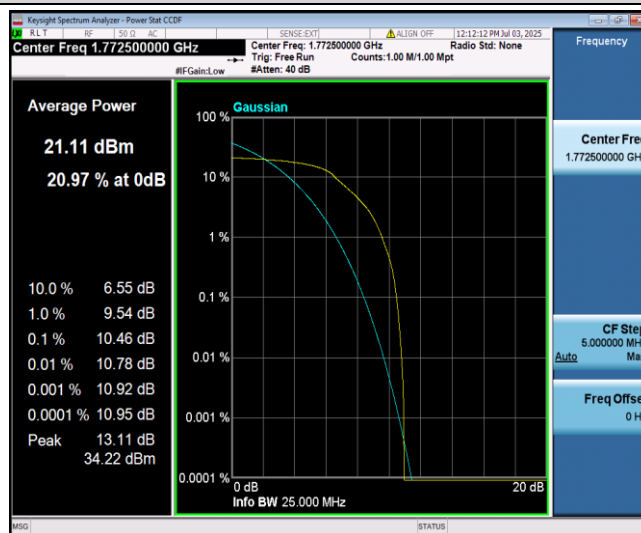
Band66-15MHz-16QAM-132597-6-0-High-10.46-<=13-PASS
