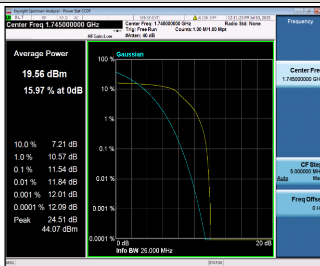
Band66-15MHz-QPSK-132322-6-0-Low-11.54-<=13-PASS
