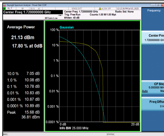
Band66-20MHz-16QAM-132072-1-0-Low-10.78-<=13-PASS
