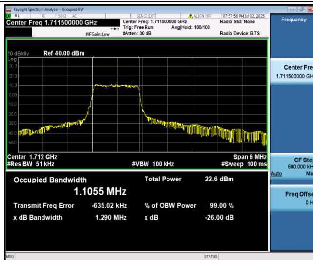
Band66-3MHz-16QAM-131987-6-0-Low-1.1055-1.106-PASS
