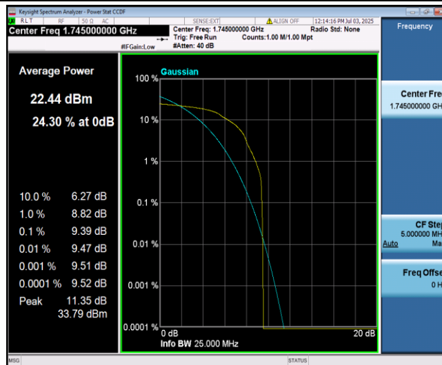
Band66-20MHz-16QAM-132322-1-0-Low-9.39-<=13-PASS
