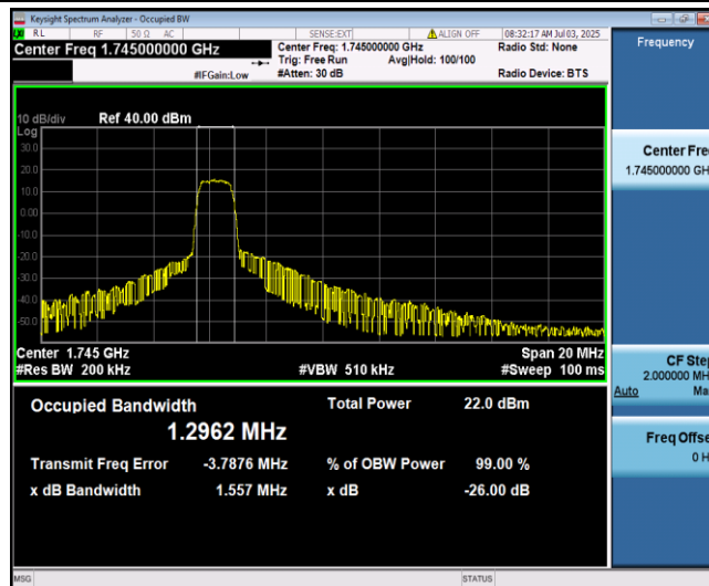
Band66-10MHz-16QAM-132322-6-0-Low-1.2962-1.296-PASS
