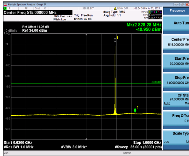
Band12-10MHz-QPSK-23060-1-0-Low-30-1000--40.95-PASS
