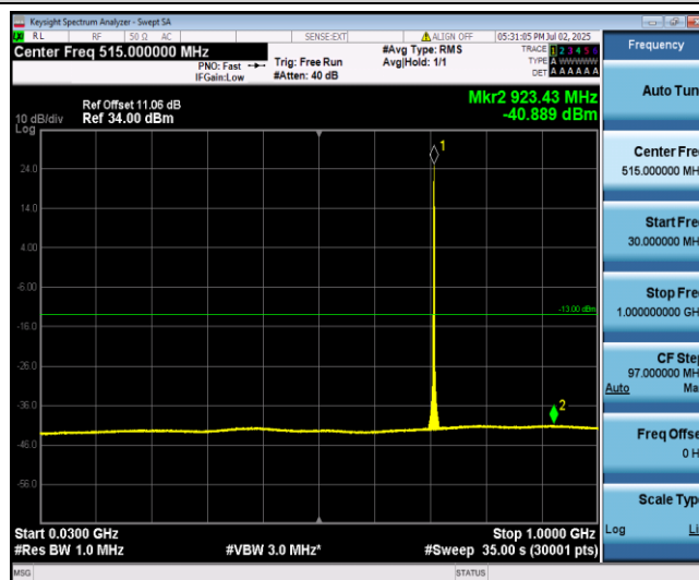
Band12-3MHz-16QAM-23165-1-0-High-30-1000--40.89-PASS
