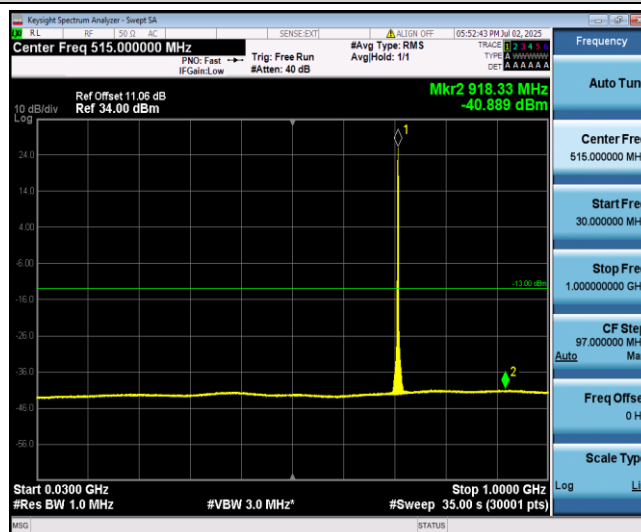
Band12-5MHz-QPSK-23155-1-0-High-30-1000--40.89-PASS
