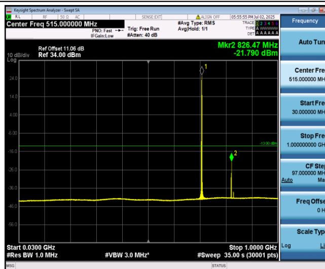
Band12-5MHz-16QAM-23155-1-0-High-30-1000--21.79-PASS
