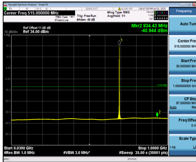
Band12-10MHz-16QAM-23060-1-0-Low-30-1000--40.94-PASS
