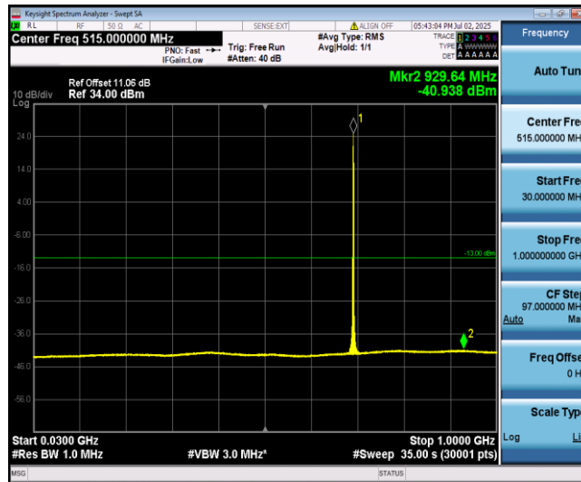
Band12-5MHz-16QAM-23035-1-0-Low-30-1000--40.94-PASS
