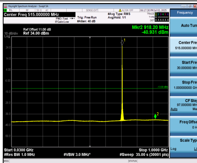
Band12-10MHz-QPSK-23130-1-0-High-30-1000--40.93-PASS
