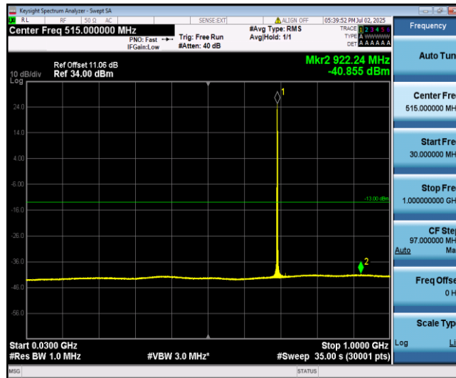
Band12-5MHz-QPSK-23035-1-0-Low-30-1000--40.86-PASS
