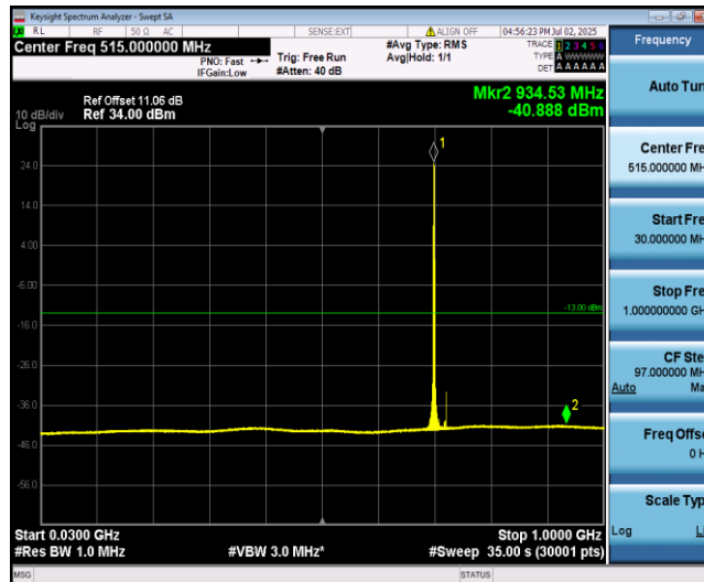
Band12-1.4MHz-QPSK-23095-1-0-Low-30-1000--40.89-PASS
