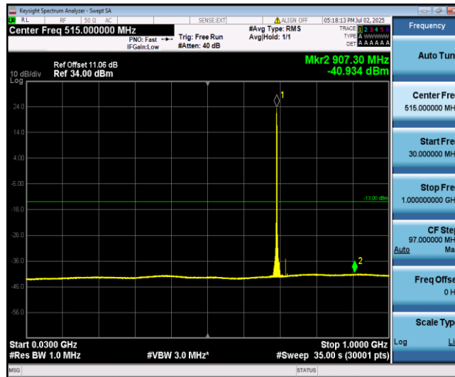
Band12-3MHz-16QAM-23025-1-0-Low-30-1000--40.93-PASS
