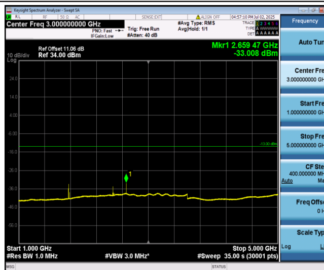
Band12-1.4MHz-QPSK-23095-1-0-Low-1000-5000--33.01-PASS
