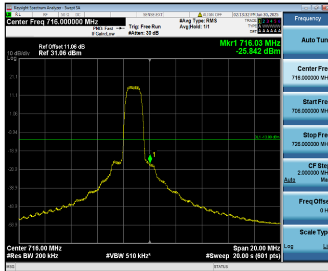
Band12-10MHz-16QAM-23130-6-0-High--25.84-PASS
