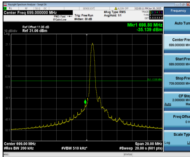
Band12-10MHz-16QAM-23060-1-0-Low--35.14-PASS
