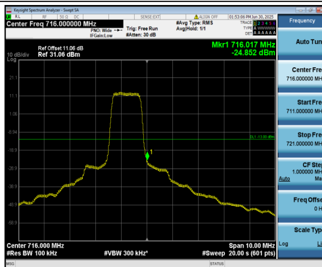
Band12-5MHz-16QAM-23155-6-0-High--24.85-PASS
