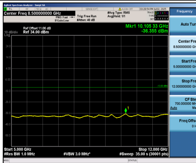
Band12-1.4MHz-16QAM-23017-1-0-Low-5000-12000--36.36-PASS
