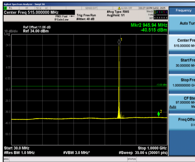
Band12-1.4MHz-16QAM-23017-1-0-Low-30-1000--40.52-PASS
