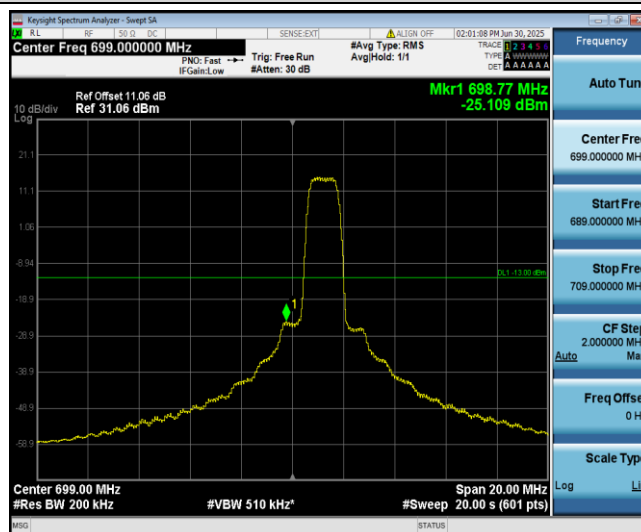
Band12-10MHz-16QAM-23060-6-0-Low--25.11-PASS
