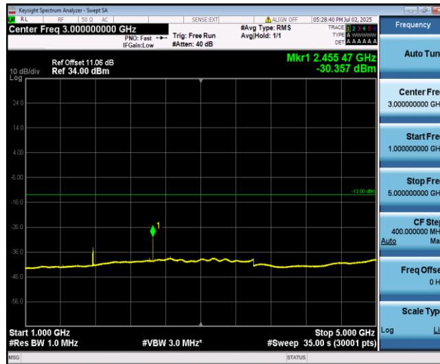
Band12-3MHz-QPSK-23165-1-0-High-1000-5000--30.36-PASS
