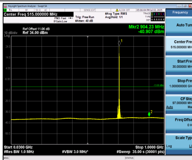
Band12-1.4MHz-16QAM-23173-1-0-High-30-1000--40.91-PASS
