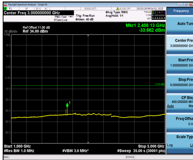
Band12-1.4MHz-QPSK-23173-1-0-High-1000-5000--33.66-PASS
