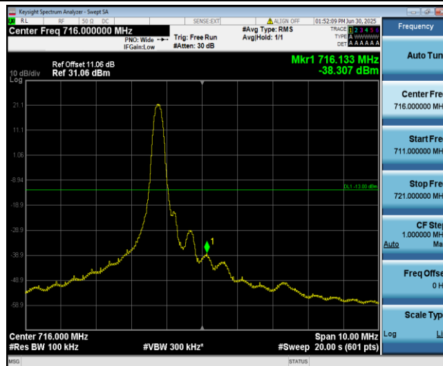
Band12-5MHz-16QAM-23155-1-0-High--38.31-PASS
