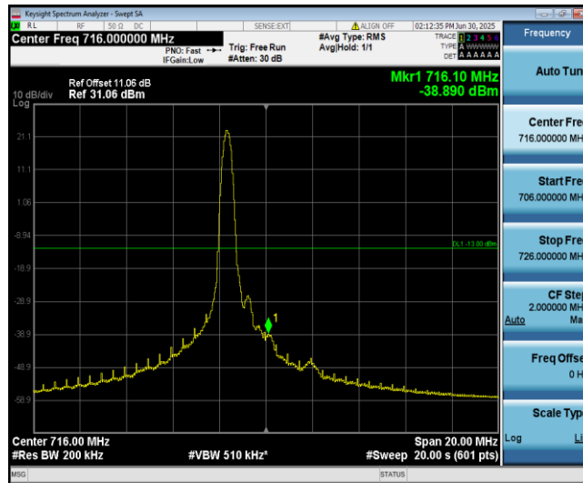
Band12-10MHz-16QAM-23130-1-0-High--38.89-PASS
