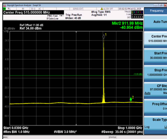
Band12-1.4MHz-QPSK-23173-1-0-High-30-1000--40.95-PASS
