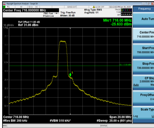
Band12-10MHz-QPSK-23130-6-0-High--25.63-PASS
