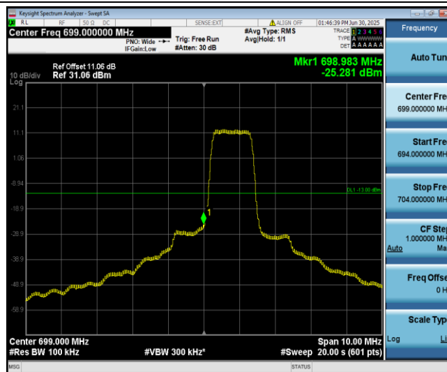
Band12-5MHz-16QAM-23035-6-0-Low--25.28-PASS
