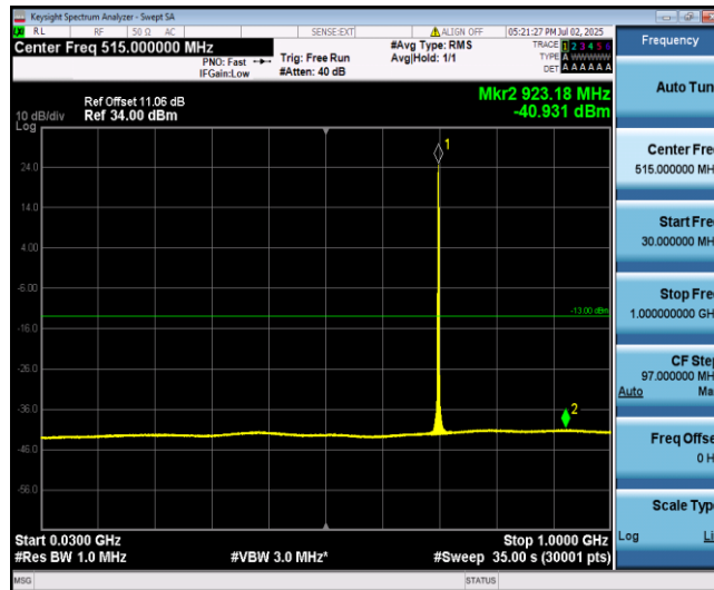
Band12-3MHz-QPSK-23095-1-0-Low-30-1000--40.93-PASS
