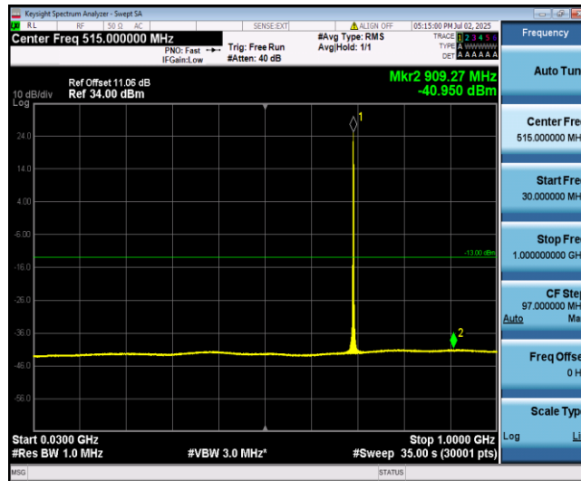
Band12-3MHz-QPSK-23025-1-0-Low-30-1000--40.95-PASS
