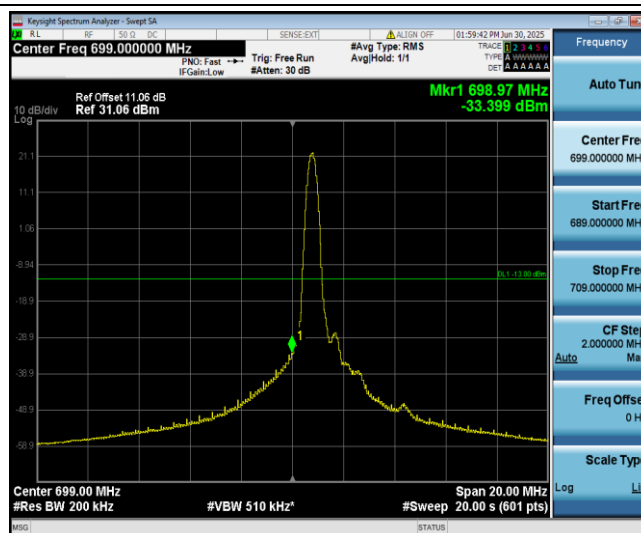
Band12-10MHz-QPSK-23060-1-0-Low--33.40-PASS
