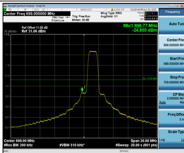
Band12-10MHz-QPSK-23060-6-0-Low--24.86-PASS
