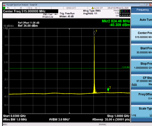
Band12-3MHz-QPSK-23165-1-0-High-30-1000--40.31-PASS
