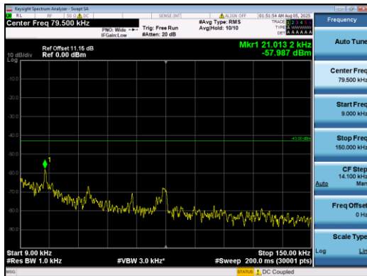
Band2-15MHz-QPSK-18675-1#0-0.009-0.15-PASS
