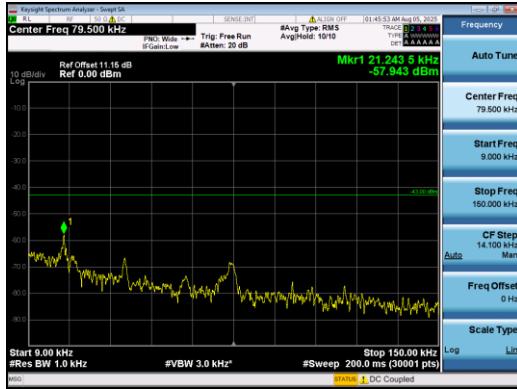
Band2-10MHz-16QAM-18650-1#0-0.009-0.15-PASS
