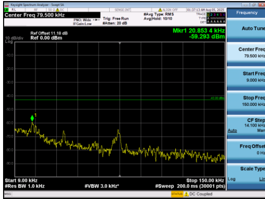
Band2-3MHz-16QAM-19185-1#5-0.009-0.15-PASS
