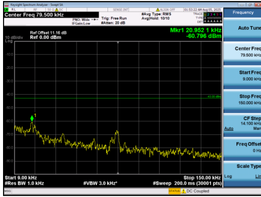
Band2-15MHz-16QAM-18900-1#0-0.009-0.15-PASS
