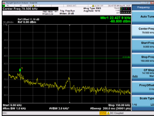
Band2-10MHz-16QAM-19150-1#5-0.009-0.15-PASS
