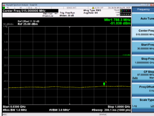
Band2-3MHz-QPSK-19185-1#5-30-1000-PASS
