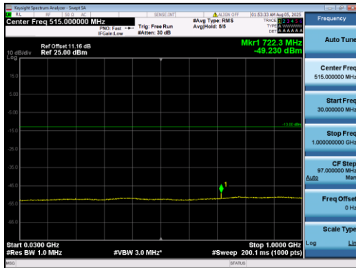
Band2-15MHz-16QAM-18900-1#0-30-1000-PASS
