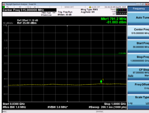
Band2-5MHz-16QAM-18900-1#0-30-1000-PASS
