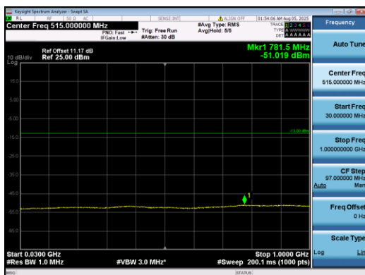
Band2-15MHz-QPSK-19125-1#5-30-1000-PASS
