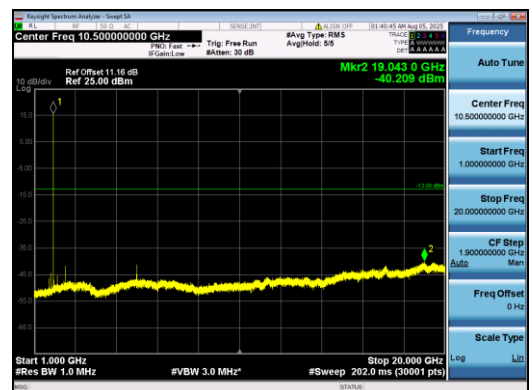
Band2-5MHz-QPSK-18900-1#0-1000-20000-PASS
