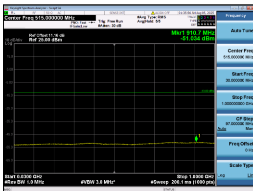
Band2-3MHz-QPSK-18900-1#0-30-1000-PASS
