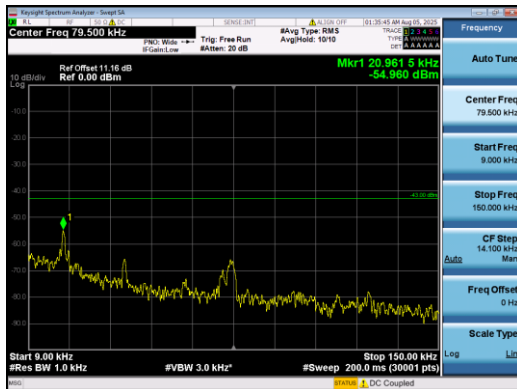
Band2-3MHz-QPSK-18900-1#0-0.009-0.15-PASS
