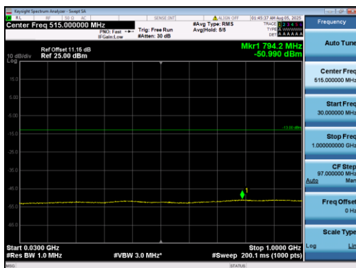
Band2-10MHz-QPSK-18650-1#0-30-1000-PASS
