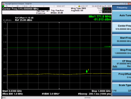
Band2-5MHz-16QAM-18625-1#0-30-1000-PASS
