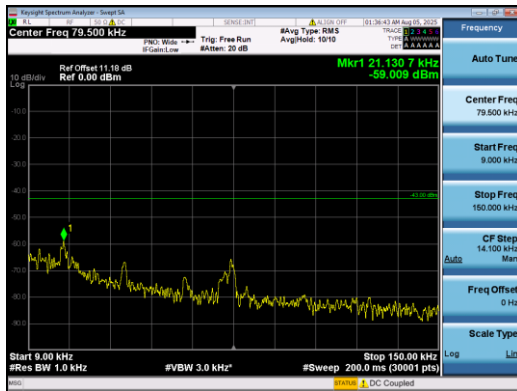
Band2-3MHz-QPSK-19185-1#5-0.009-0.15-PASS
