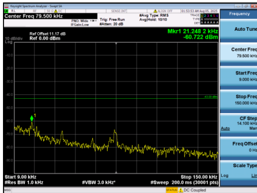
Band2-15MHz-QPSK-19125-1#5-0.009-0.15-PASS
