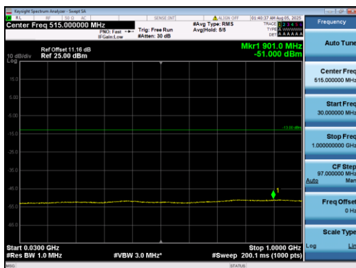
Band2-5MHz-QPSK-18900-1#0-30-1000-PASS
