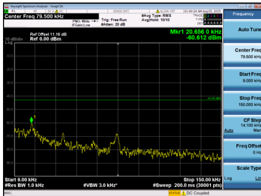
Band2-5MHz-QPSK-18900-1#0-0.009-0.15-PASS
