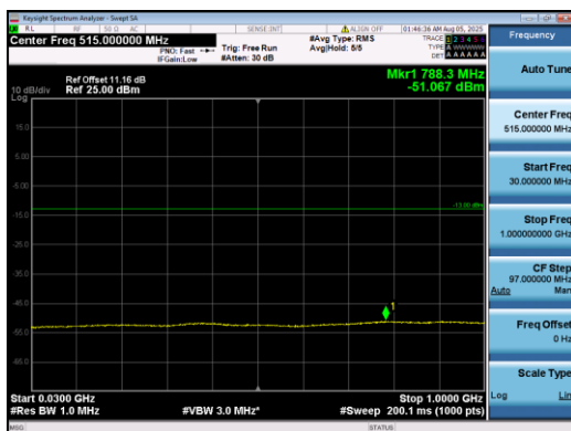
Band2-10MHz-QPSK-18900-1#0-30-1000-PASS
