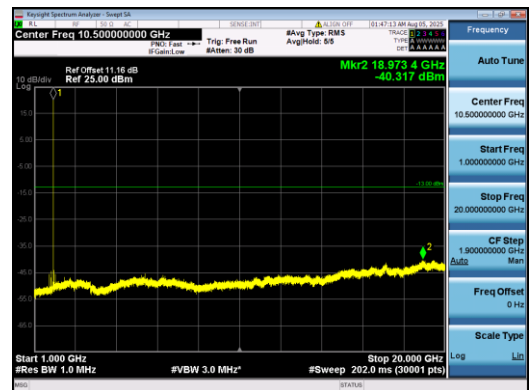
Band2-10MHz-16QAM-18900-1#0-1000-20000-PASS
