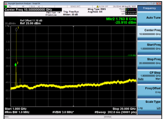
Band2-15MHz-16QAM-18900-1#0-1000-20000-PASS
