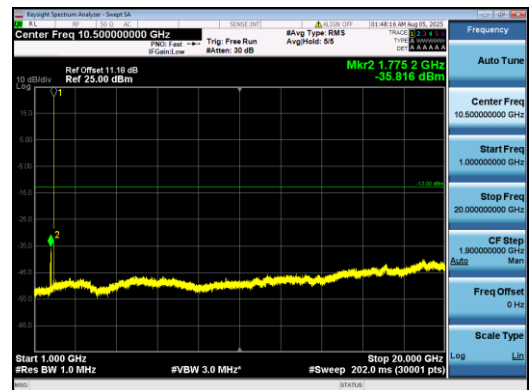
Band2-10MHz-16QAM-19150-1#5-1000-20000-PASS
