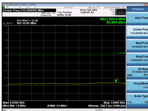
Band2-5MHz-QPSK-18625-1#0-30-1000-PASS
