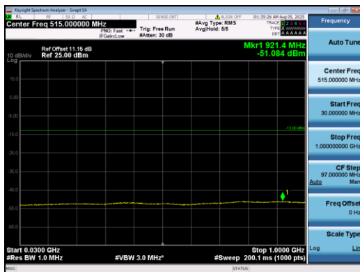
Band2-3MHz-16QAM-18615-1#0-30-1000-PASS
