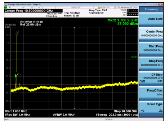
Band2-3MHz-16QAM-19185-1#5-1000-20000-PASS
