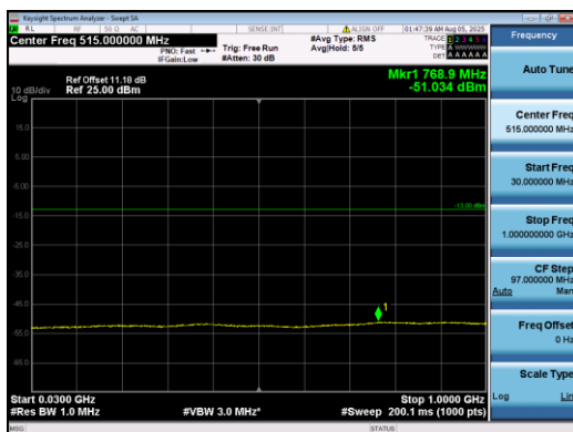
Band2-10MHz-QPSK-19150-1#5-30-1000-PASS
