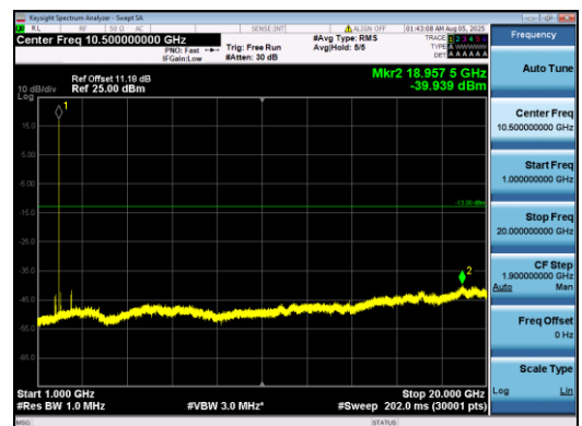
Band2-5MHz-QPSK-19175-1#5-1000-20000-PASS
