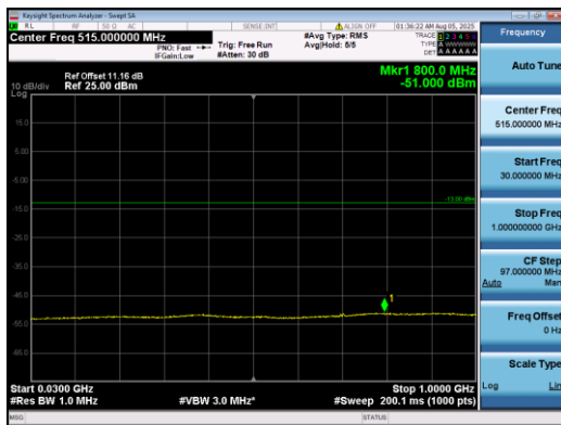
Band2-3MHz-16QAM-18900-1#0-30-1000-PASS
