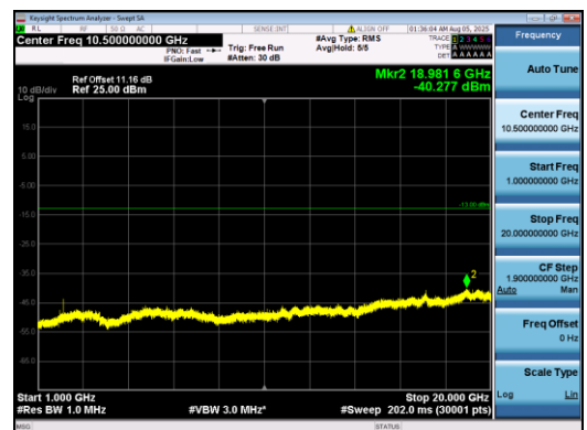
Band2-3MHz-QPSK-18900-1#0-1000-20000-PASS
