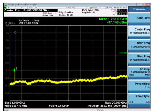
Band2-15MHz-QPSK-18900-1#0-1000-20000-PASS
