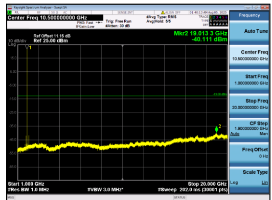
Band2-5MHz-16QAM-18625-1#0-1000-20000-PASS
