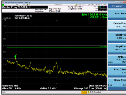
Band2-3MHz-16QAM-18900-1#0-0.009-0.15-PASS
