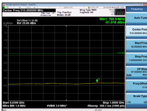
Band2-5MHz-QPSK-19175-1#5-30-1000-PASS
