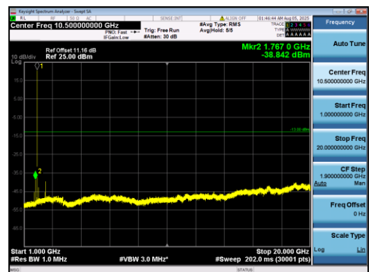
Band2-10MHz-QPSK-18900-1#0-1000-20000-PASS
