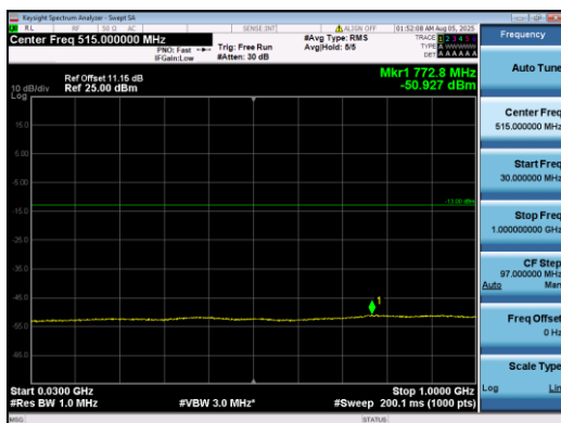
Band2-15MHz-QPSK-18675-1#0-30-1000-PASS
