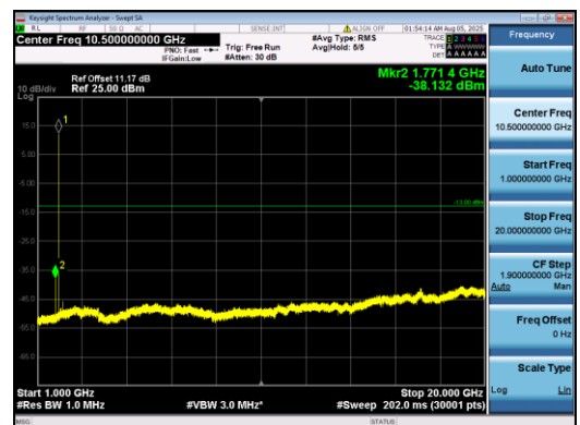
Band2-15MHz-QPSK-19125-1#5-1000-20000-PASS
