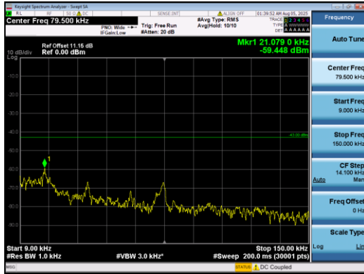
Band2-5MHz-16QAM-18625-1#0-0.009-0.15-PASS
