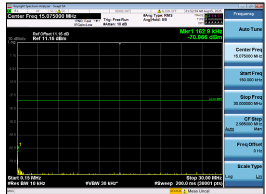
Band2-15MHz-QPSK-18900-1#0-0.15-30-PASS
