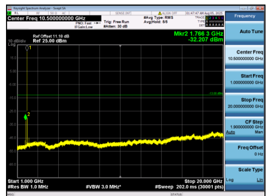
Band2-10MHz-QPSK-19150-1#5-1000-20000-PASS
