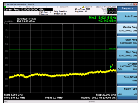
Band2-3MHz-QPSK-19185-1#5-1000-20000-PASS
