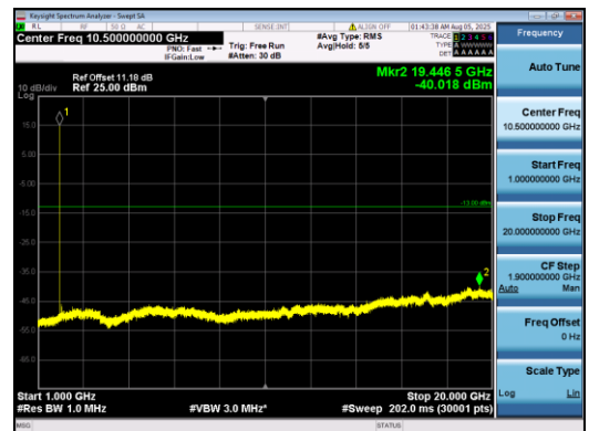
Band2-5MHz-16QAM-19175-1#5-1000-20000-PASS
