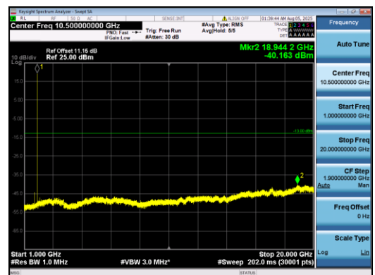
Band2-5MHz-QPSK-18625-1#0-1000-20000-PASS
