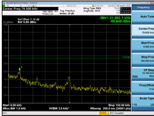
Band2-5MHz-16QAM-19175-1#5-0.009-0.15-PASS
