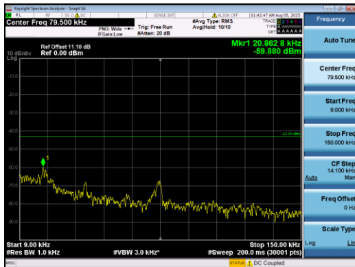
Band2-5MHz-QPSK-19175-1#5-0.009-0.15-PASS
