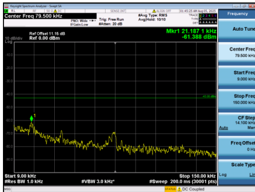
Band2-10MHz-QPSK-18650-1#0-0.009-0.15-PASS
