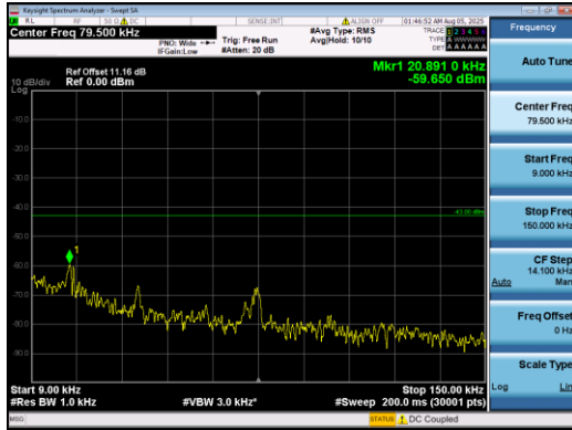
Band2-10MHz-16QAM-18900-1#0-0.009-0.15-PASS
