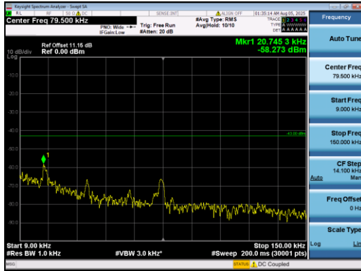
Band2-3MHz-16QAM-18615-1#0-0.009-0.15-PASS
