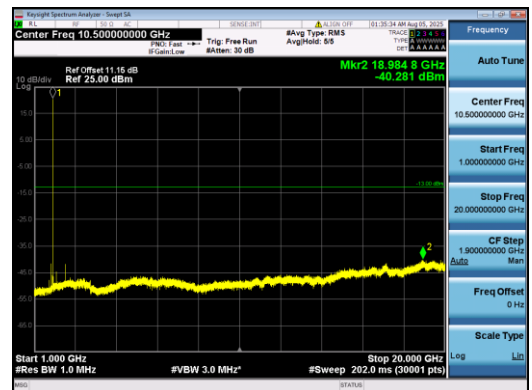
Band2-3MHz-16QAM-18615-1#0-1000-20000-PASS
