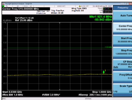
Band2-10MHz-16QAM-19150-1#5-30-1000-PASS
