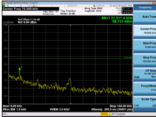
Band2-5MHz-16QAM-18900-1#0-0.009-0.15-PASS
