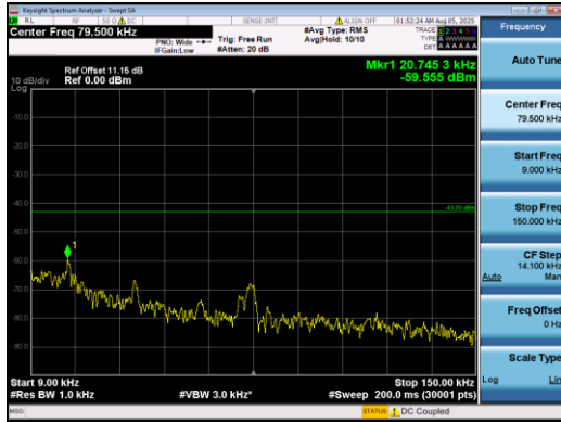
Band2-15MHz-16QAM-18675-1#0-0.009-0.15-PASS
