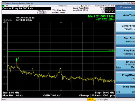
Band2-5MHz-QPSK-18625-1#0-0.009-0.15-PASS
