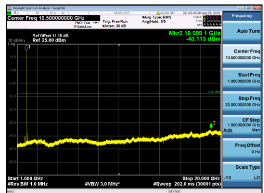
Band2-10MHz-QPSK-18650-1#0-1000-20000-PASS
