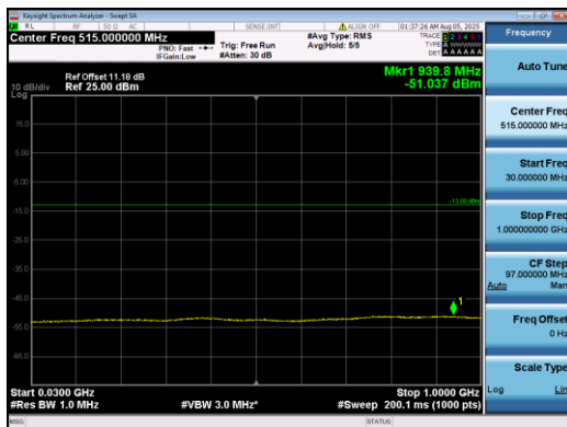
Band2-3MHz-16QAM-19185-1#5-30-1000-PASS
