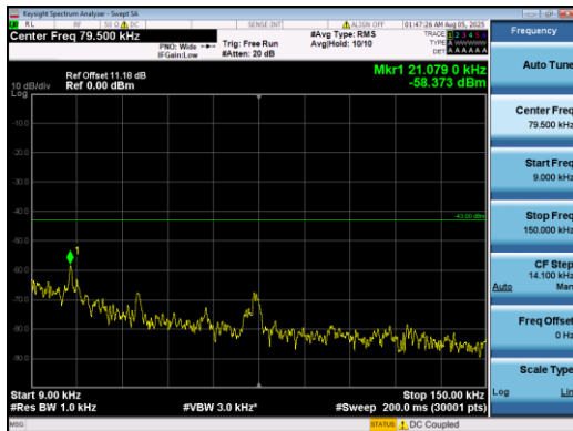
Band2-10MHz-QPSK-19150-1#5-0.009-0.15-PASS
