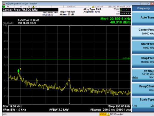
Band2-15MHz-QPSK-18900-1#0-0.009-0.15-PASS
