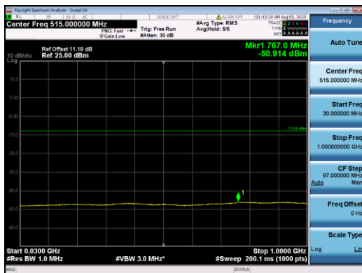
Band2-5MHz-16QAM-19175-1#5-30-1000-PASS
