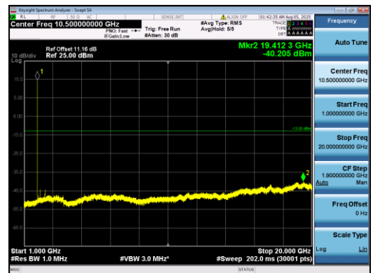
Band2-5MHz-16QAM-18900-1#0-1000-20000-PASS
