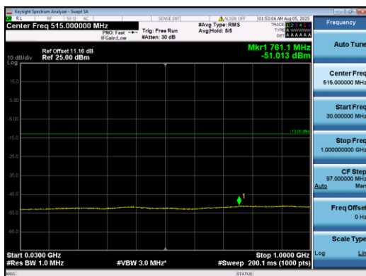
Band2-15MHz-QPSK-18900-1#0-30-1000-PASS
