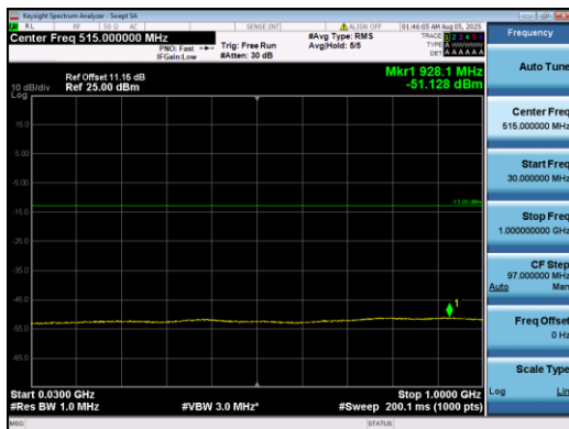
Band2-10MHz-16QAM-18650-1#0-30-1000-PASS
