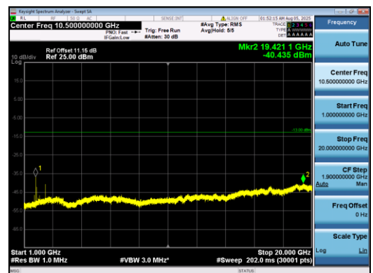
Band2-15MHz-QPSK-18675-1#0-1000-20000-PASS
