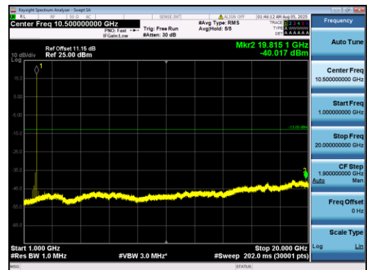
Band2-10MHz-16QAM-18650-1#0-1000-20000-PASS
