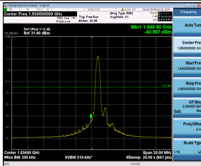
Band2-10MHz-16QAM-18650-1-0-Low--40.99-PASS
