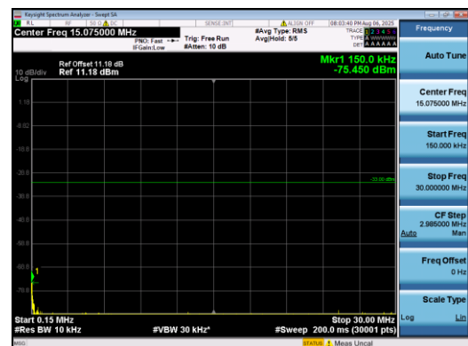
Band2-1.4MHz-16QAM-19193-1#5-0.15-30-PASS
