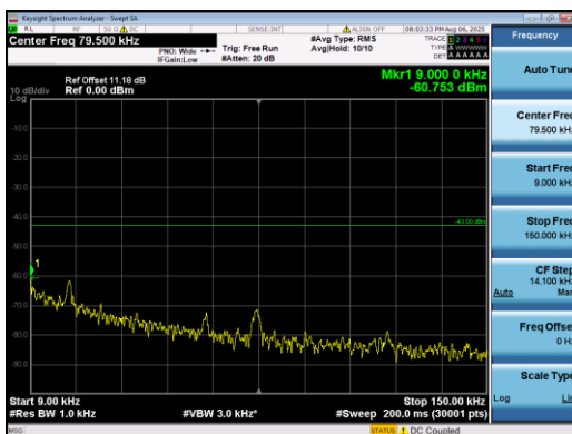
Band2-1.4MHz-16QAM-19193-1#5-0.009-0.15-PASS
