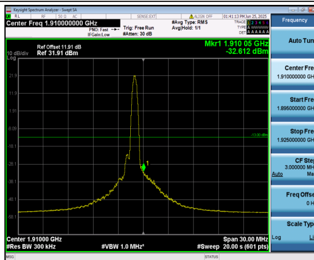
Band2-15MHz-16QAM-19125-1-5-High--32.61-PASS
