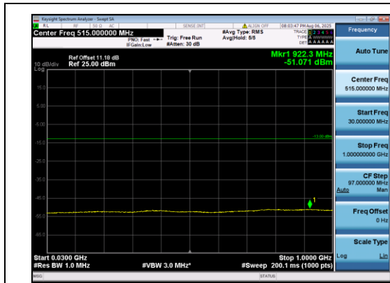
Band2-1.4MHz-16QAM-19193-1#5-30-1000-PASS
