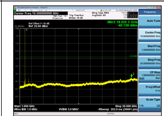
Band2-3MHz-QPSK-18615-1#0-1000-20000-PASS
