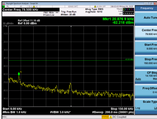
Band2-1.4MHz-QPSK-19193-1#5-0.009-0.15-PASS
