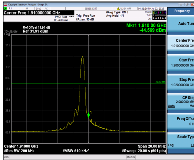
Band2-10MHz-16QAM-19150-1-5-High--44.57-PASS
