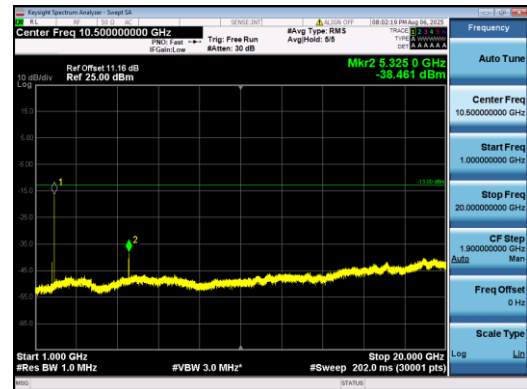
Band2-1.4MHz-QPSK-18900-1#0-1000-20000-PASS
