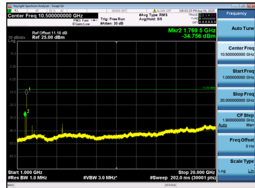
Band2-1.4MHz-QPSK-19193-1#5-1000-20000-PASS
