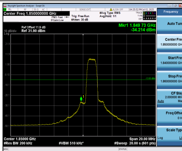
Band2-10MHz-16QAM-18650-6-0-Low--34.21-PASS
