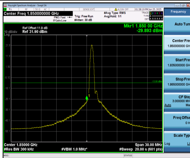
Band2-15MHz-QPSK-18675-1-0-Low--29.89-PASS
