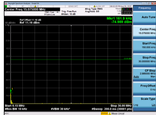
Band2-1.4MHz-QPSK-18900-1#0-0.15-30-PASS
