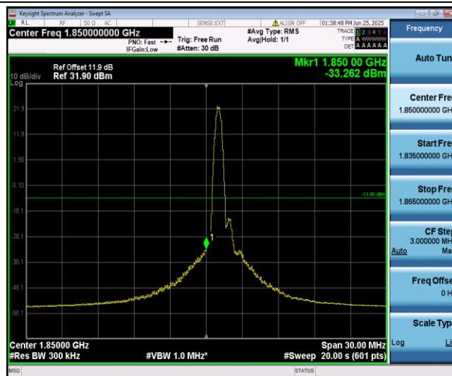
Band2-15MHz-16QAM-18675-1-0-Low--33.26-PASS
