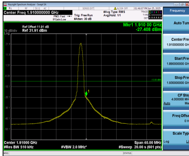
Band2-20MHz-QPSK-19100-1-5-High--27.41-PASS
