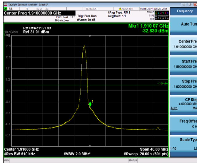
Band2-20MHz-16QAM-19100-1-5-High--32.83-PASS
