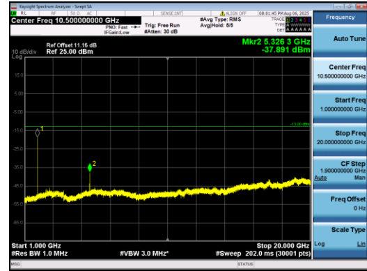
Band2-1.4MHz-16QAM-18607-1#0-1000-20000-PASS
