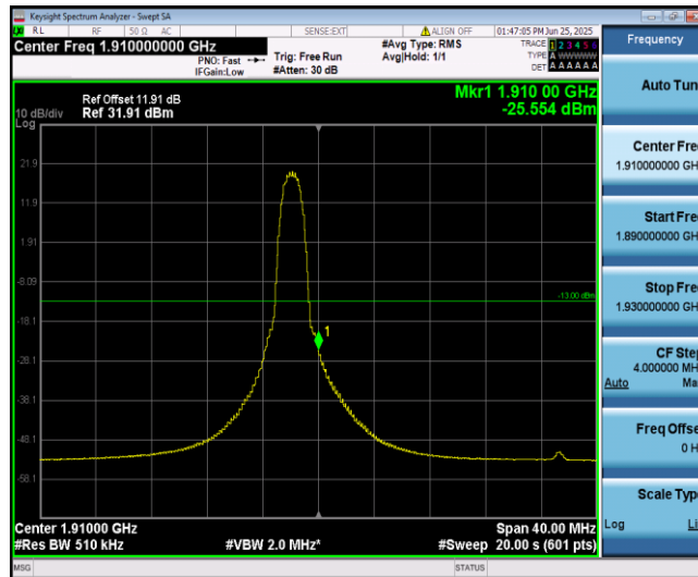
Band2-20MHz-QPSK-19100-6-0-High--25.55-PASS
