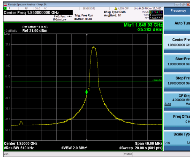
Band2-20MHz-16QAM-18700-6-0-Low--25.28-PASS
