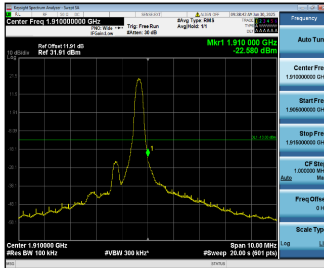
Band2-5MHz-16QAM-19175-1-5-High--22.58-PASS
