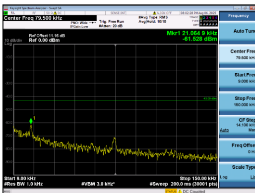
Band2-1.4MHz-16QAM-18900-1#0-0.009-0.15-PASS
