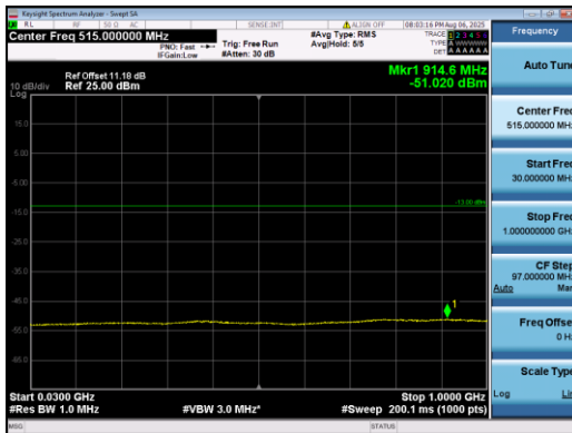
Band2-1.4MHz-QPSK-19193-1#5-30-1000-PASS
