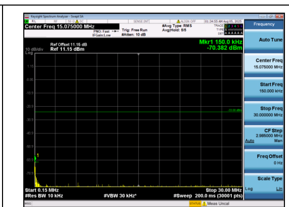
Band2-3MHz-QPSK-18615-1#0-0.15-30-PASS
