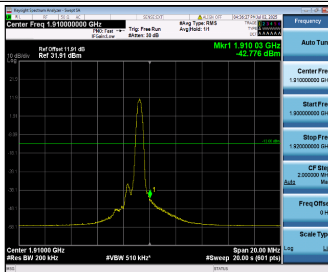
Band2-10MHz-QPSK-19150-1-5-High--42.78-PASS
