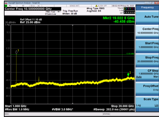
Band2-1.4MHz-16QAM-18900-1#0-1000-20000-PASS
