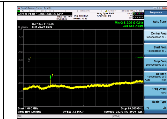
Band2-1.4MHz-16QAM-19193-1#5-1000-20000-PASS
