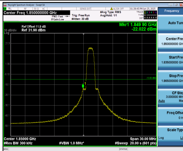
Band2-15MHz-16QAM-18675-6-0-Low--22.02-PASS
