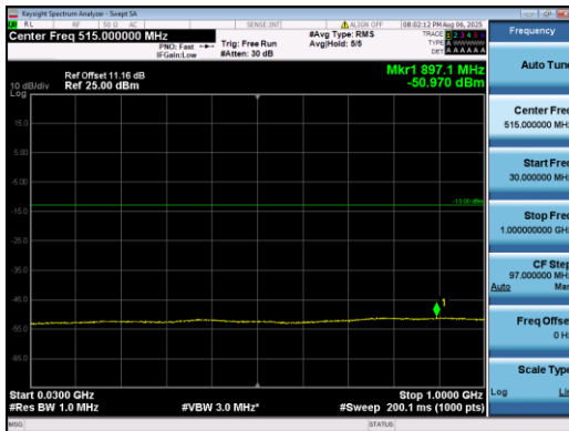
Band2-1.4MHz-QPSK-18900-1#0-30-1000-PASS
