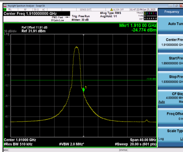
Band2-20MHz-16QAM-19100-6-0-High--24.77-PASS
