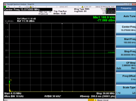
Band2-1.4MHz-16QAM-18900-1#0-0.15-30-PASS
