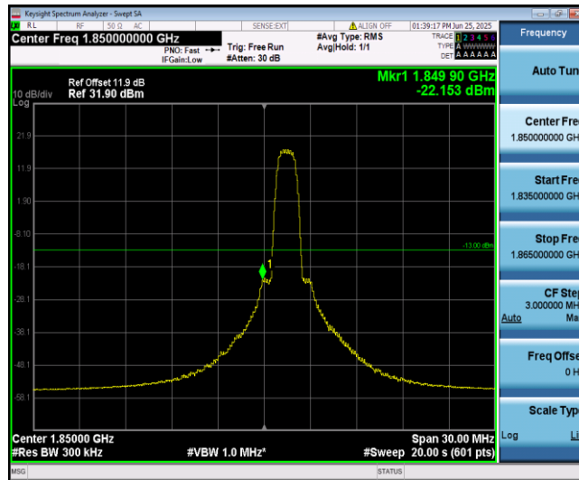
Band2-15MHz-QPSK-18675-6-0-Low--22.15-PASS
