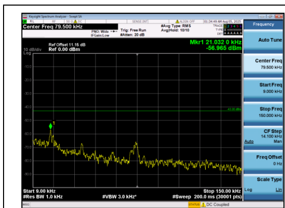
Band2-3MHz-QPSK-18615-1#0-0.009-0.15-PASS
