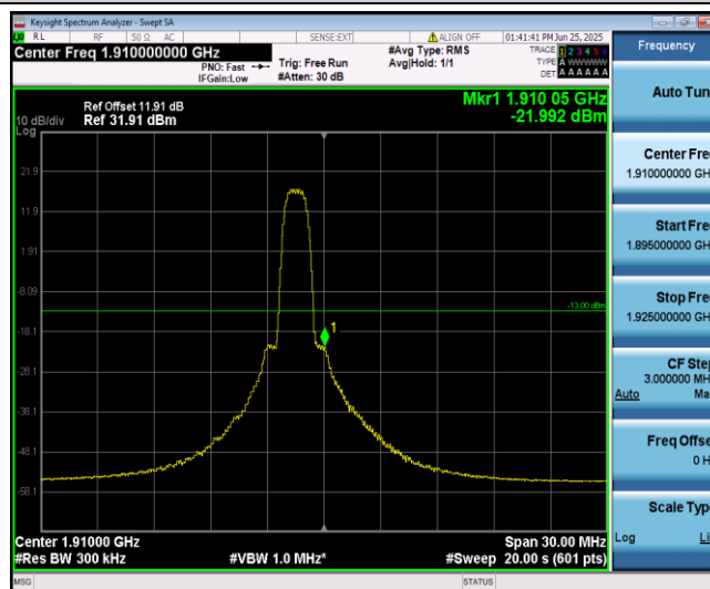
Band2-15MHz-QPSK-19125-6-0-High--21.99-PASS
