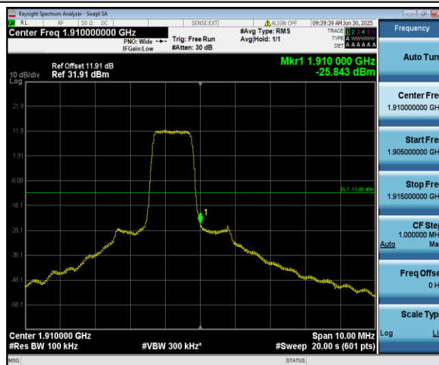
Band2-5MHz-16QAM-19175-6-0-High--25.84-PASS
