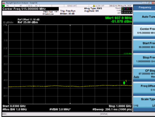
Band2-1.4MHz-16QAM-18900-1#0-30-1000-PASS
