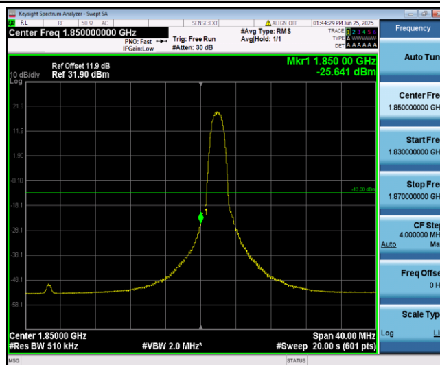
Band2-20MHz-QPSK-18700-6-0-Low--25.64-PASS
