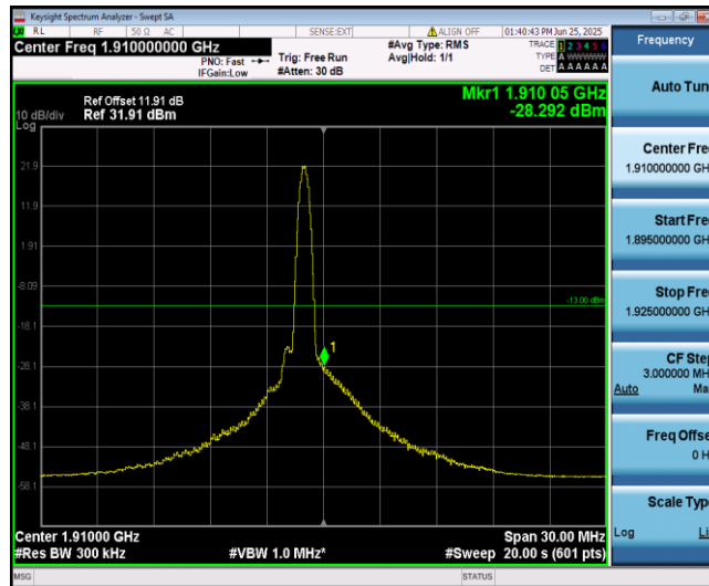
Band2-15MHz-QPSK-19125-1-5-High--28.29-PASS
