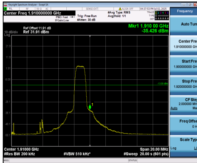
Band2-10MHz-16QAM-19150-6-0-High--35.43-PASS
