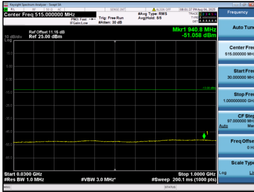
Band2-1.4MHz-16QAM-18607-1#0-30-1000-PASS
