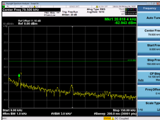
Band2-1.4MHz-QPSK-18900-1#0-0.009-0.15-PASS
