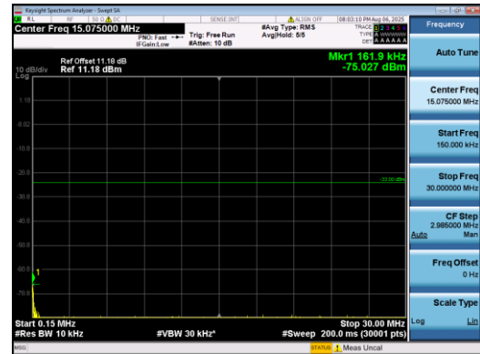
Band2-1.4MHz-QPSK-19193-1#5-0.15-30-PASS
