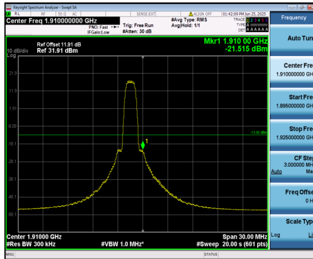
Band2-15MHz-16QAM-19125-6-0-High--21.52-PASS
