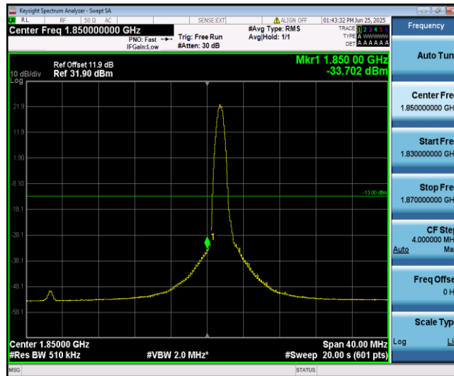
Band2-20MHz-QPSK-18700-1-0-Low--33.70-PASS
