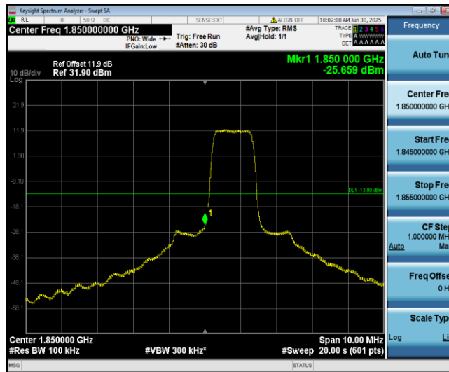
Band2-5MHz-16QAM-18625-6-0-Low--25.66-PASS
