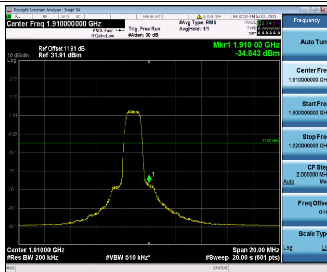
Band2-10MHz-QPSK-19150-6-0-High--34.84-PASS
