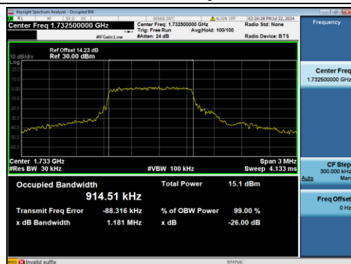
B4-1.4M-Mid CH-OBW-Q16
