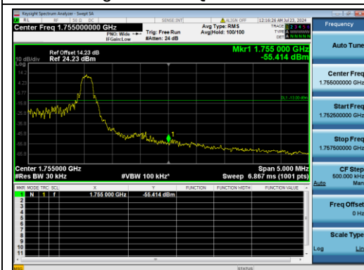
B4-20M-High CH-BE-QPSK-1 RB MAX
