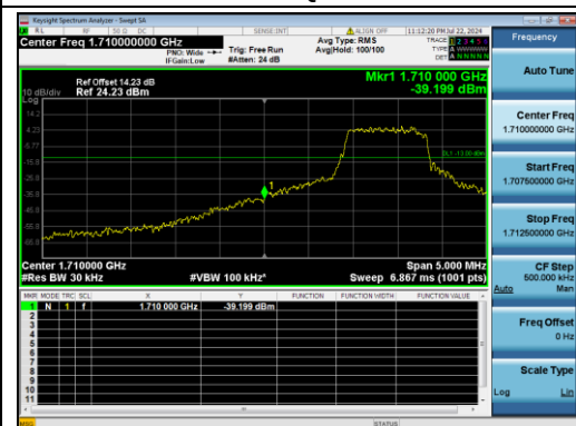
B4-15M-Low CH-BE-QPSK-Full RB 0
