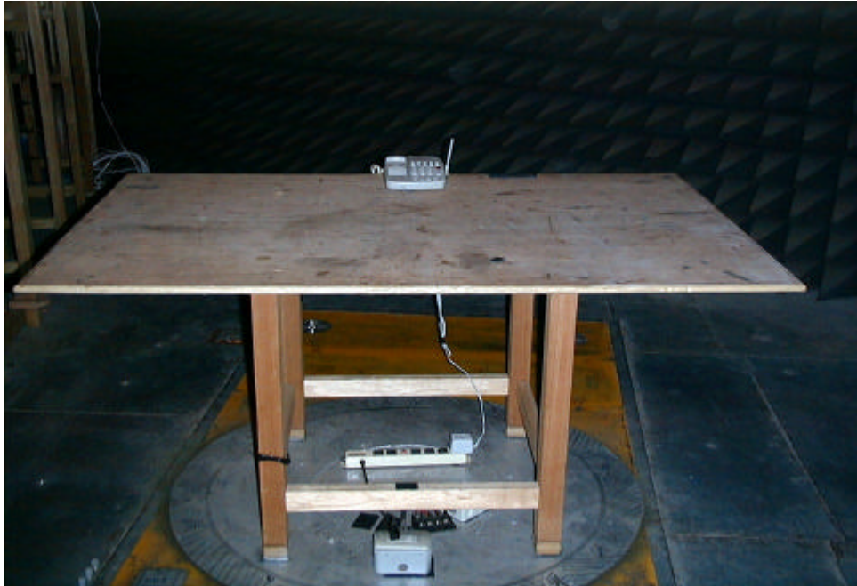
Pig 1 Front View of the Test Configuration ( BASE )
