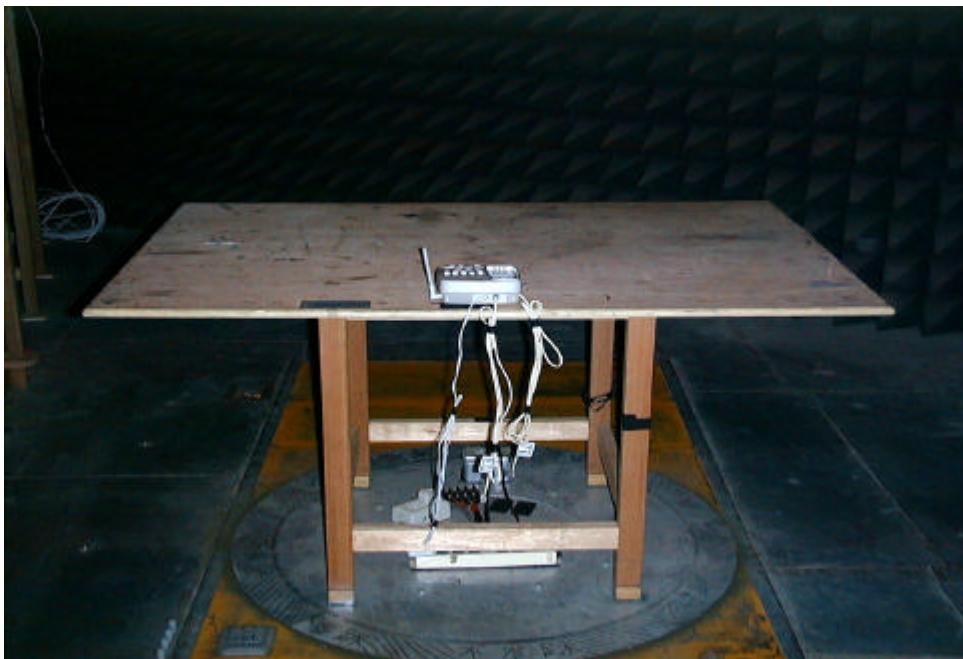
Pig 2 Rear View of the Test Configuration ( BASE )
