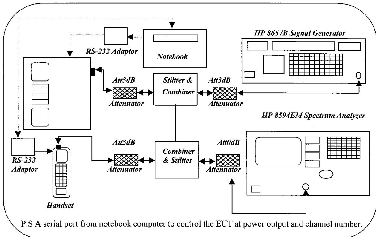
Fig. 14 Test Configuration of processing gain for handset
