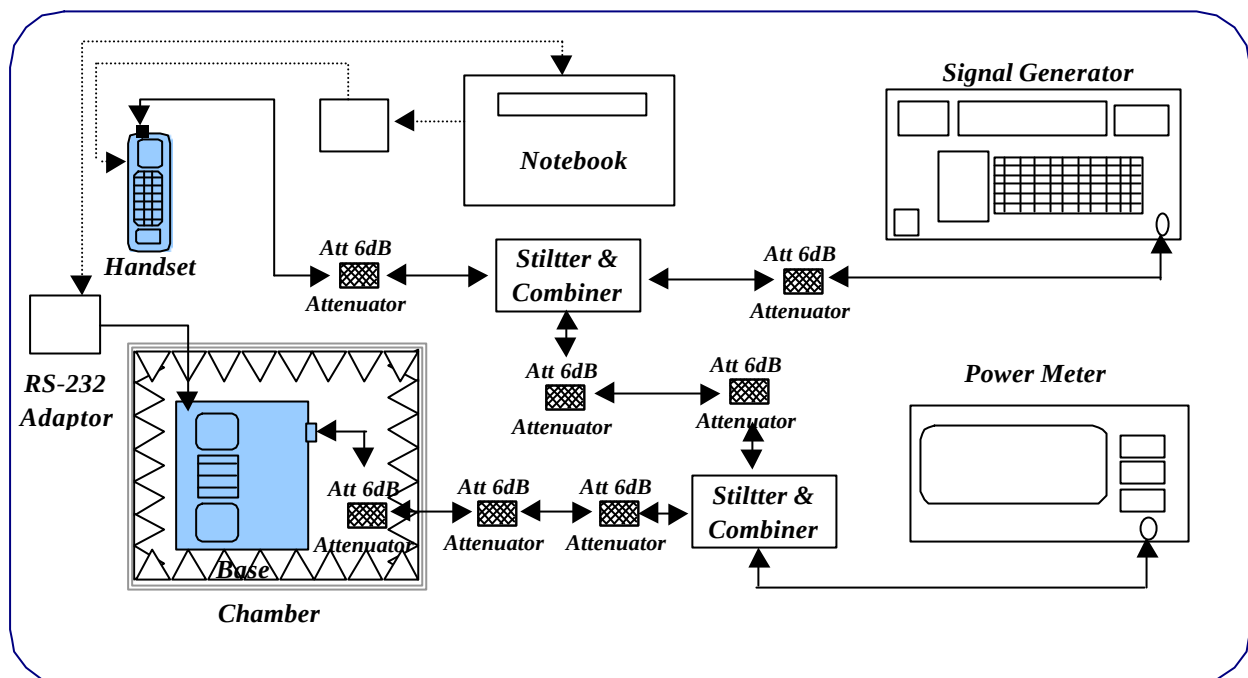
Fig. 13. Test Configuration of processing gain for base station
