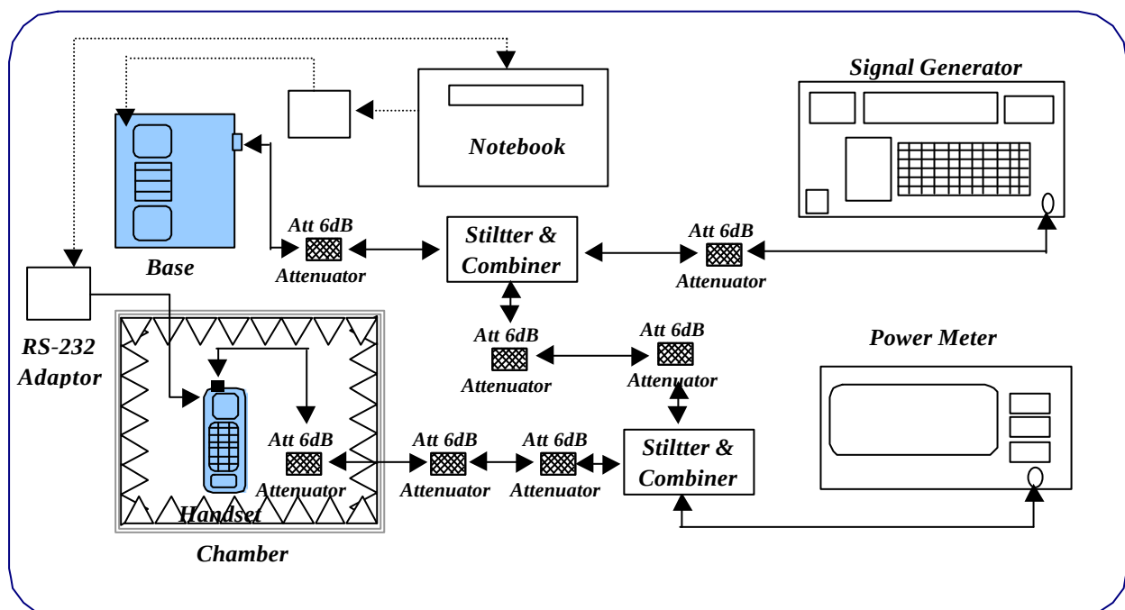
Fig. 14. Test Configuration of processing gain for handset
