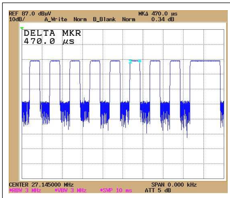
Duty Cycle 3
