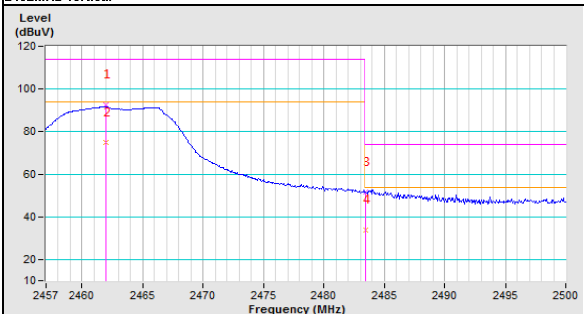
2462MHz Vertical
