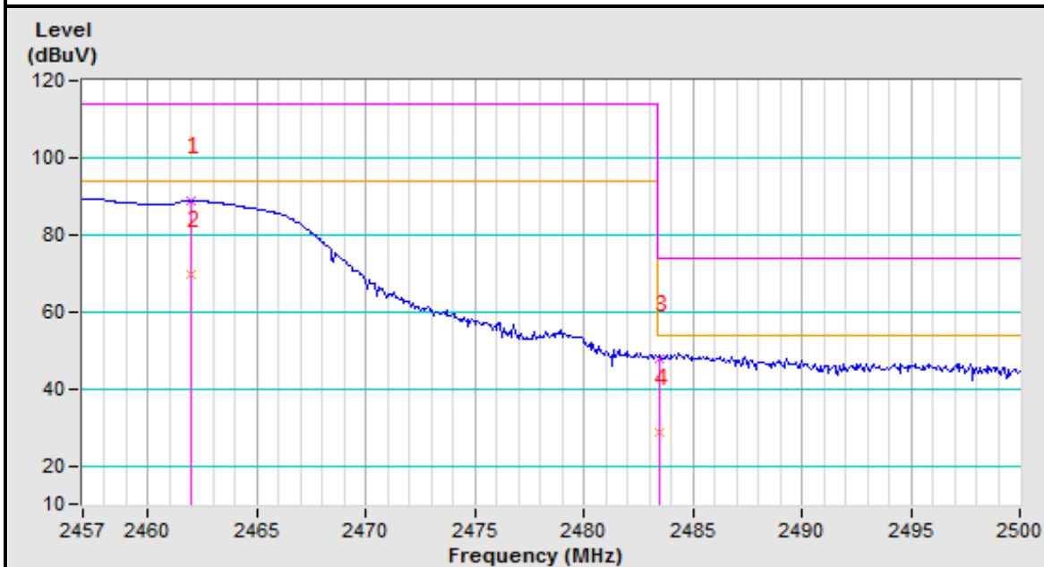
2462MHz Vertical
