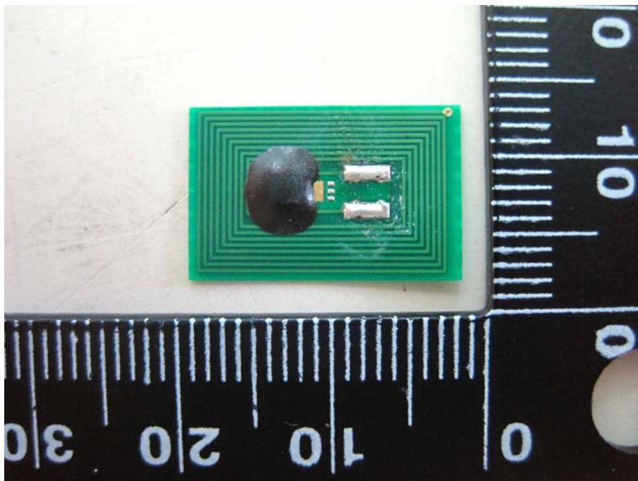
Front view of Passive NFC module
