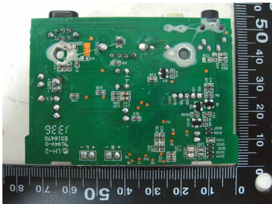
Rear View of the EUT's PCB-1
