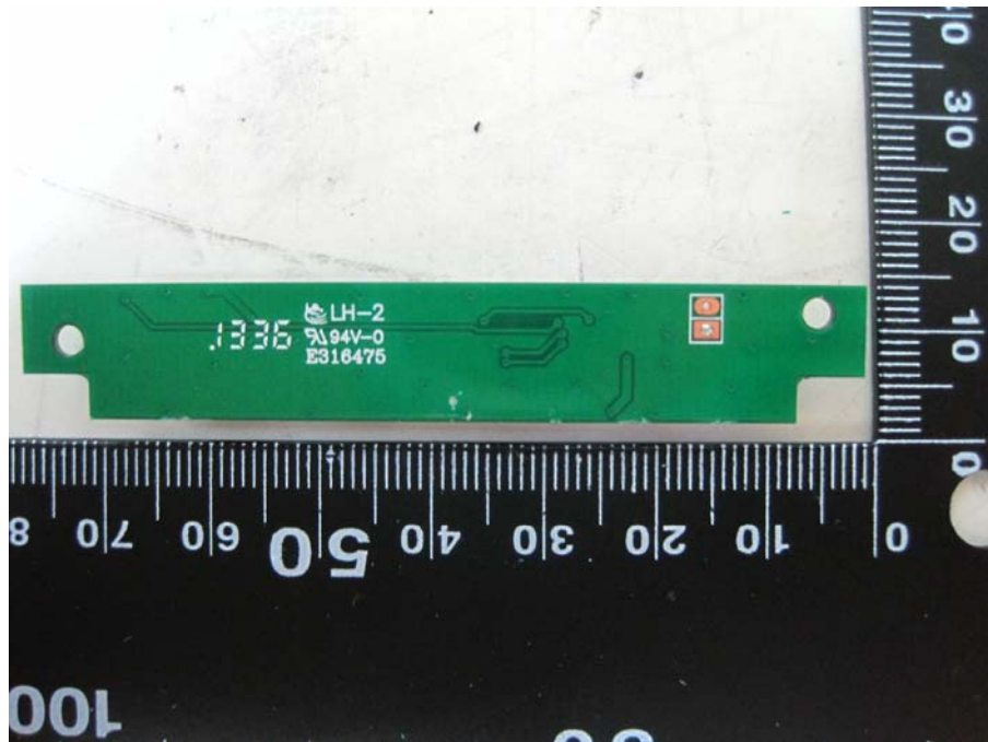
Rear View of the EUT's PCB-2
