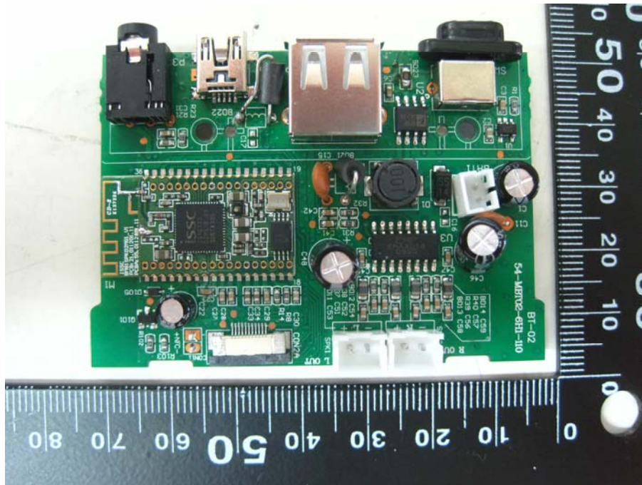
Front View of the EUT's PCB-1
