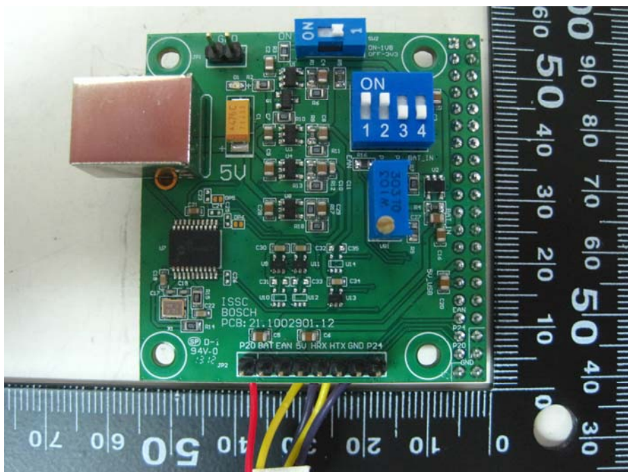
Front view of BT Test Board
