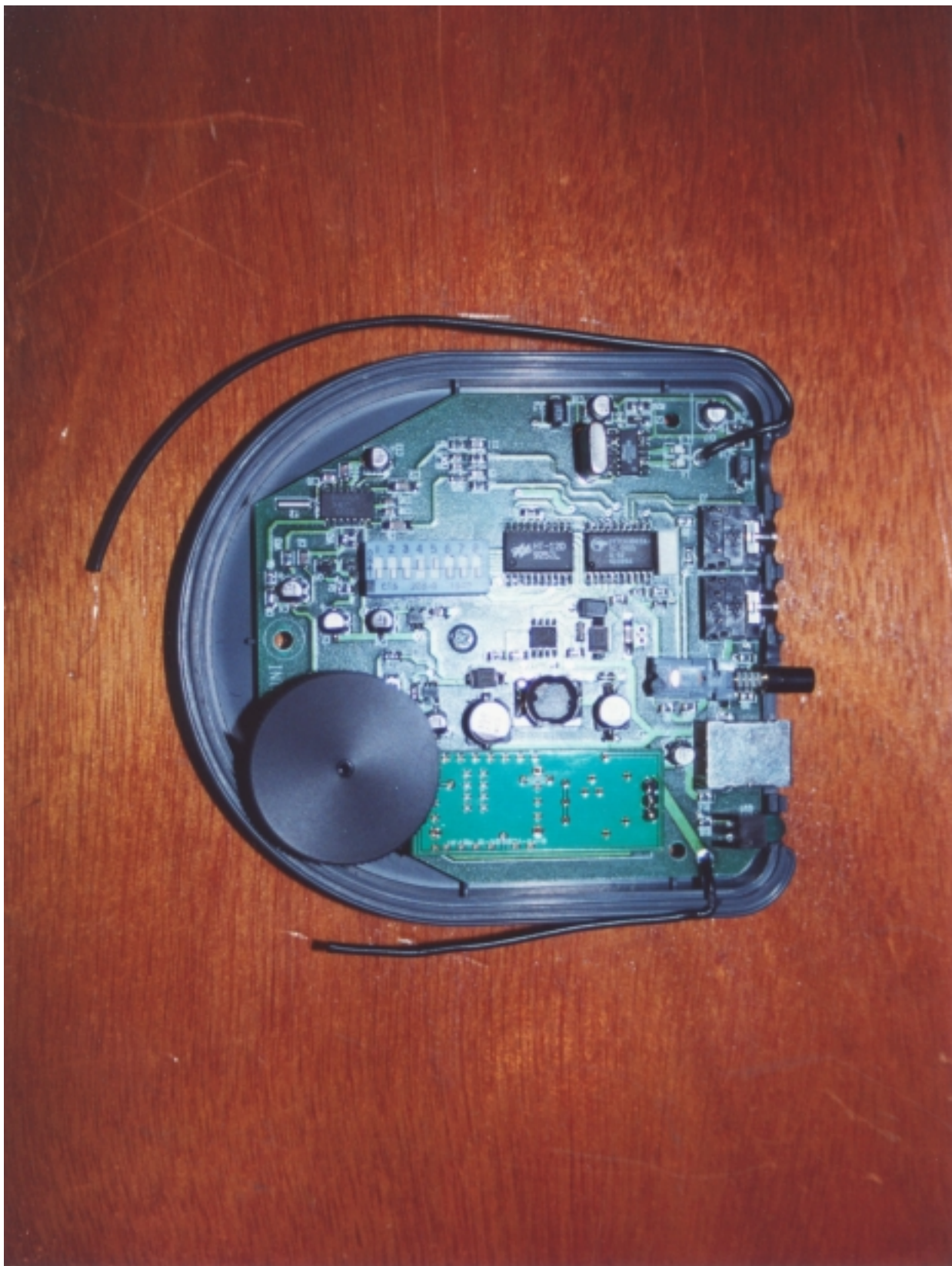
TOP INSIDE VIEW OF EUT
