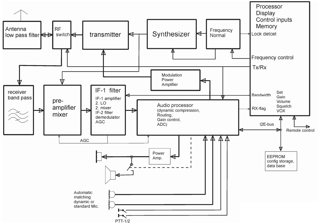
Figure 7 : KRT-2 Block Diagram
