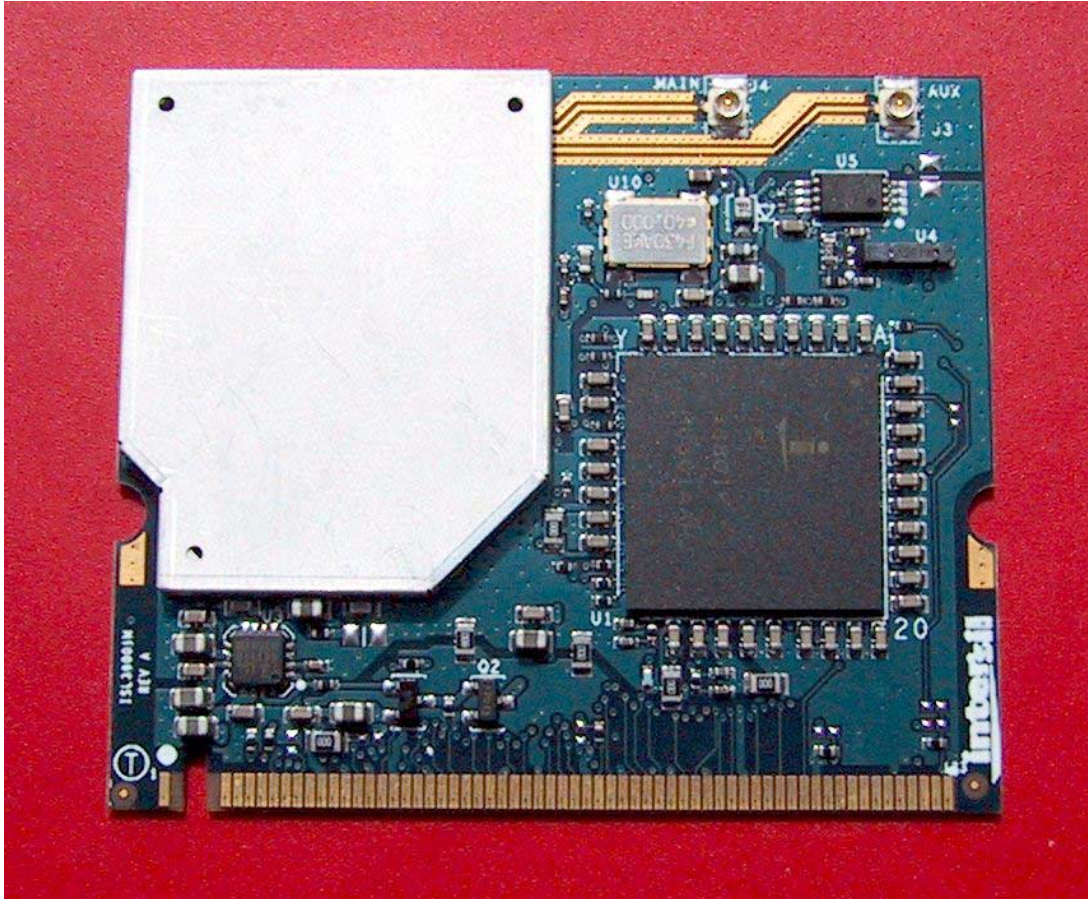
ISL38001M PCB front with shield
