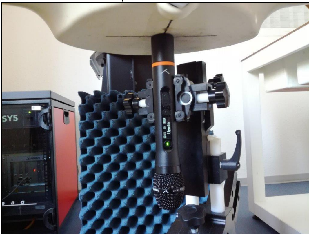
Photo 10: Test position - bottom with 0mm distance
