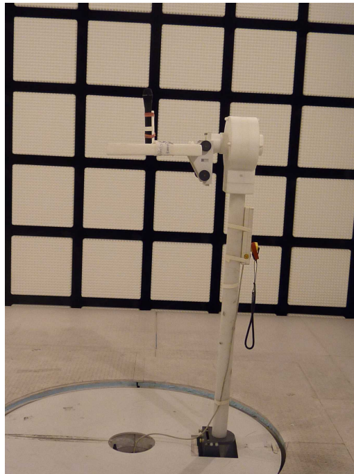
Photo 3: EUT at the anechoic chamber
