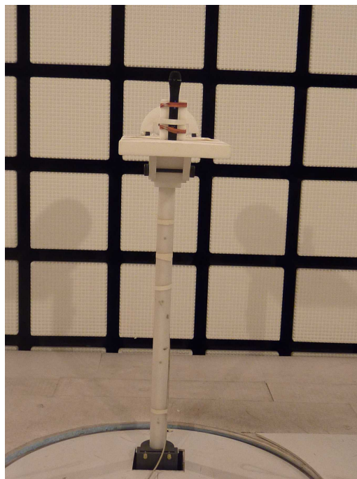
Photo 4: EUT at the anechoic chamber
