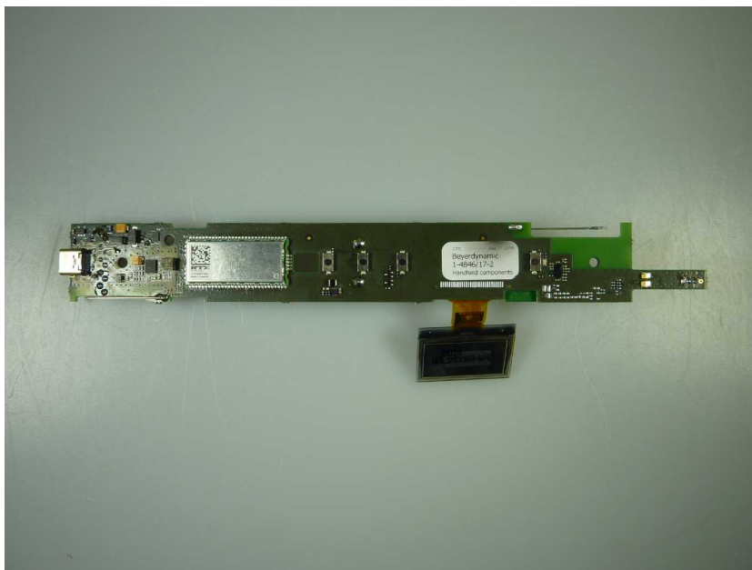
Photo 2: PCB rear side view
