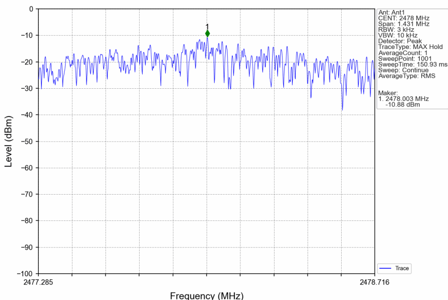
2M_HCH_2478MHz_Ant1_NTNV
