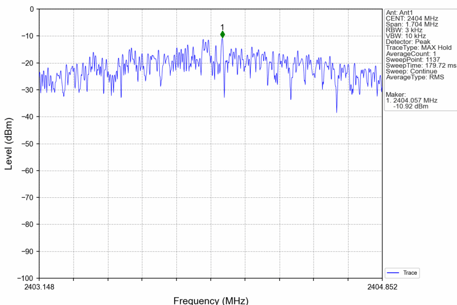
2M_LCH_2404MHz_Ant1_NTNV
