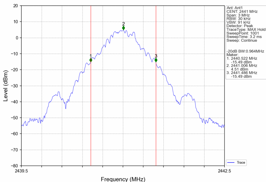
2.4G_MCH_2441MHz_Ant1_NTNV
