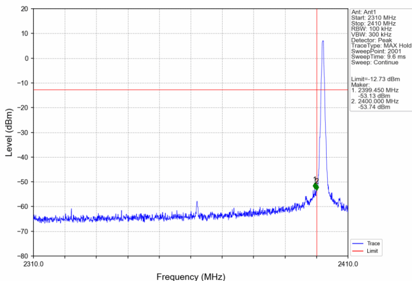
2.4G_LCH_2402MHz_Ant1_NTNV
