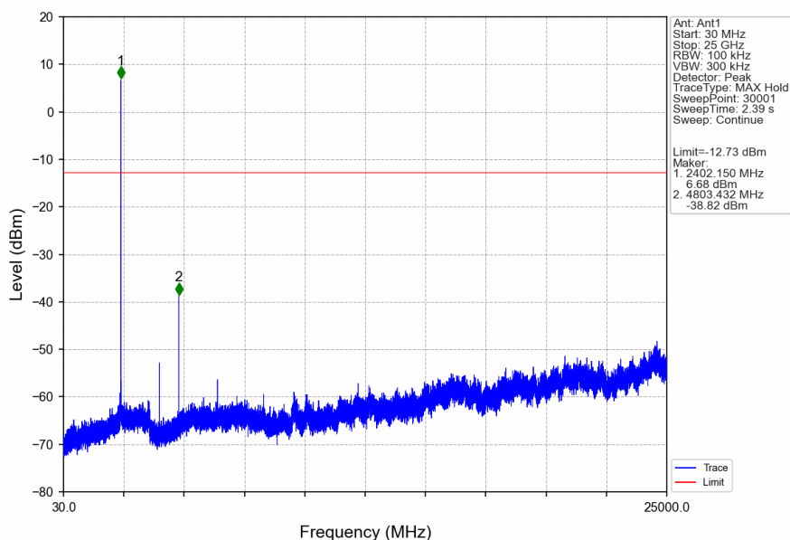
2.4G_LCH_2402MHz_Ant1_NTNV
