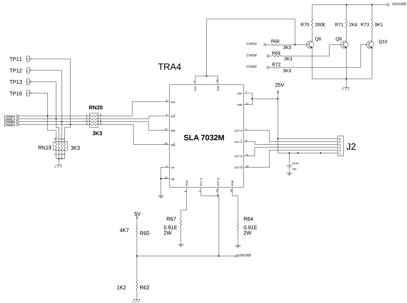
CARRAIGE MOTOR DRIVER
